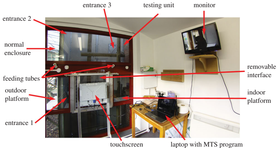
Figure 1. Overview of the Macaque Study Centre. The macaques sit on the outdoor platform until they are granted access to the testing unit. Then they sit on the indoor platform and can use the touchscreen through the interface.
