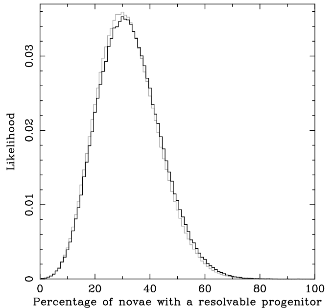
Figure 7. A plot showing the distribution of likelihood probabilities over the full range of RG-nova population proportions, 0 \leq \phi \leq 1 (resolution \phi = 0.01 ). The gray line shows the results of the basic simulation, and the black line the results of the detailed simulation that includes the effect of observational biases.
