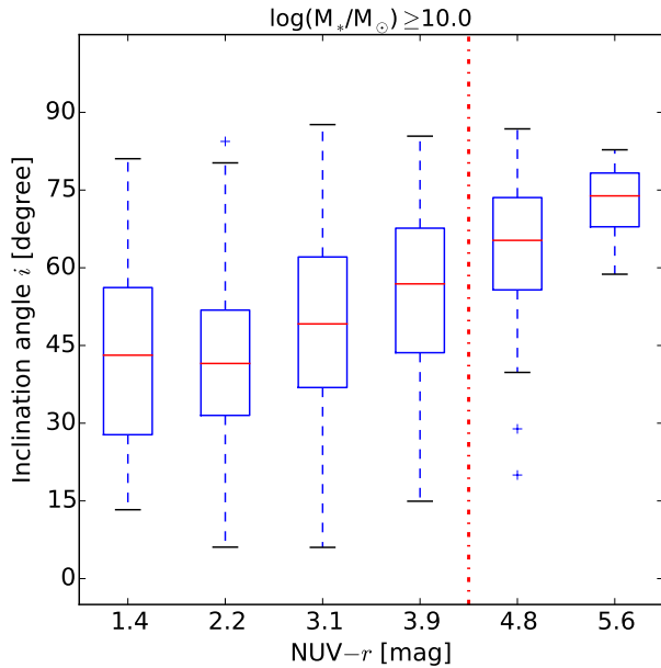
Figure 11. Distribution of galactic inclination angles i for blue and red -S galaxies, having stellar masses \log(M_*/M_{\odot}) \geq 10.0 , vs. \text{NUV}-r colour. Each box extends from the lower to upper quartile values of data, with a line at the median (red line). Inclination angles are computed using Eq. 2. Dashed lines extending vertically from the boxes indicating variability outside the upper and lower quartiles. Individual data points indicate outliers. The vertical dashed-dotted line intersects the x-axis at \text{NUV}-r = 4.5 above which galaxies are classified as red .
