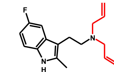
5-F-2-Me-DALT
