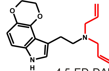
4,5-ED-DALT
