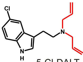
5-Cl-DALT
