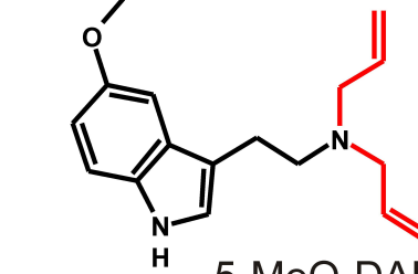
5-MeO-DALT
