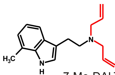
7-Me-DALT
