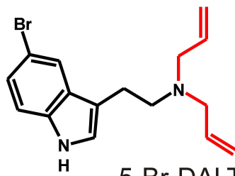
5-Br-DALT
