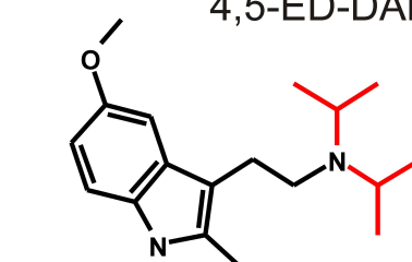
5-MeO-2-Me-DIPT
