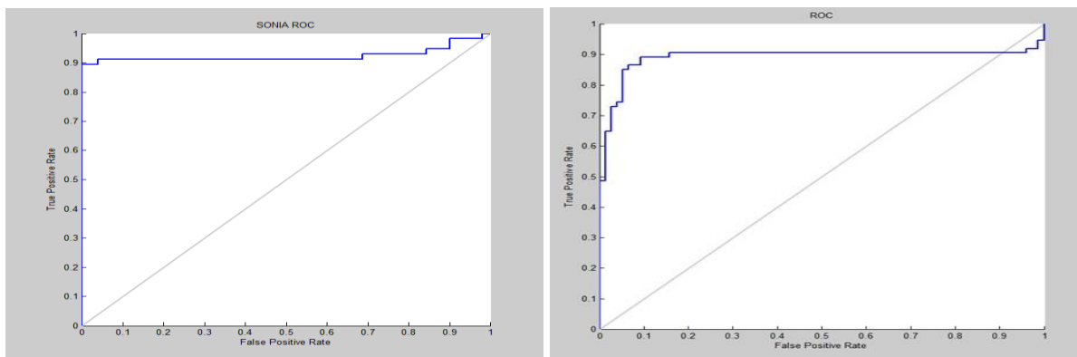
a) ROC curve for SONIA
