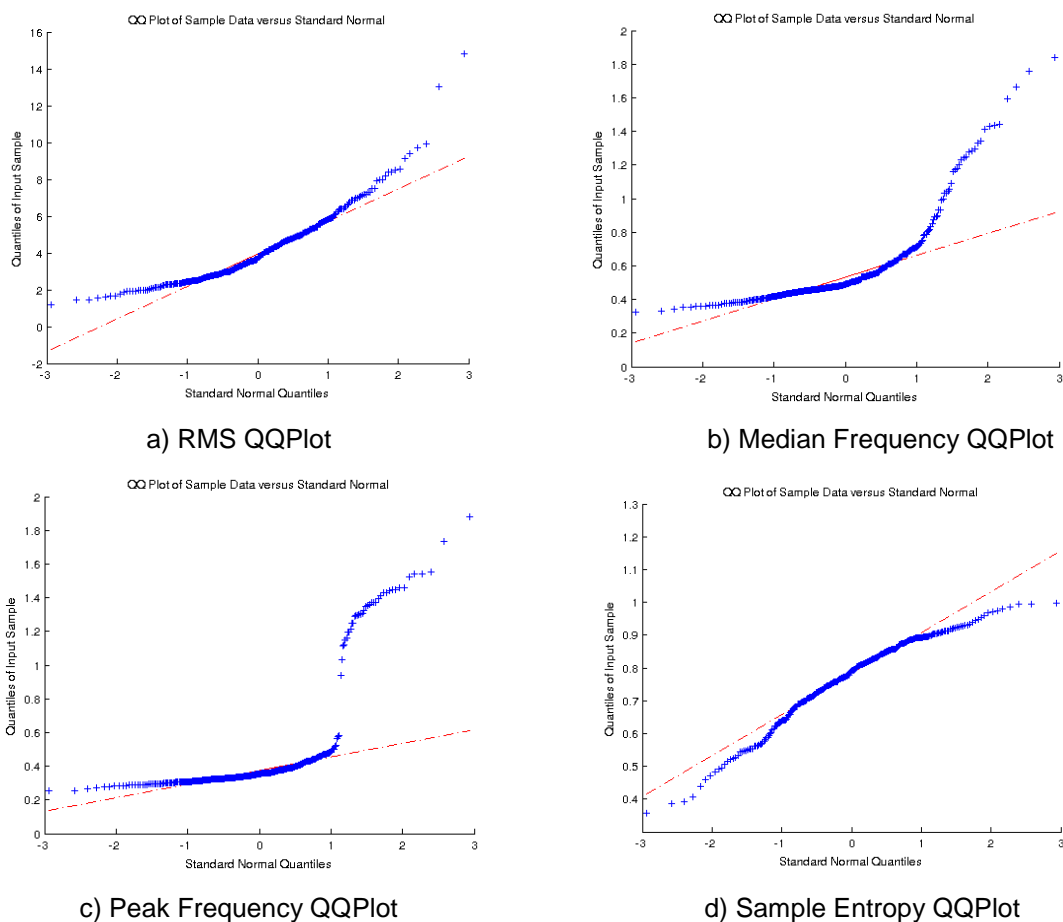
Figure 3: Outliers in TPEHG data
