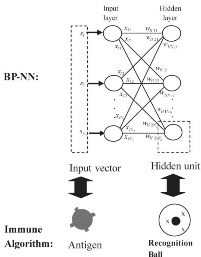
Figure 1: Input vector and hidden units of Backpropagation-NN are considered as antigen and recognition ball of immune algorithm [70].
