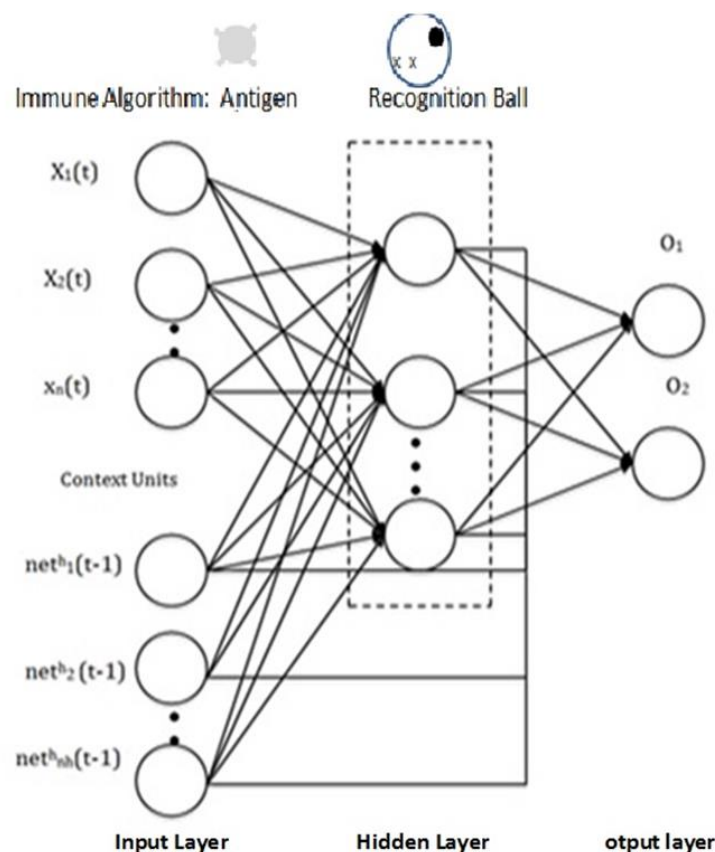
Figure 2: Dynamic Self-organized neural network inspired by immune algorithm (DSIA)
