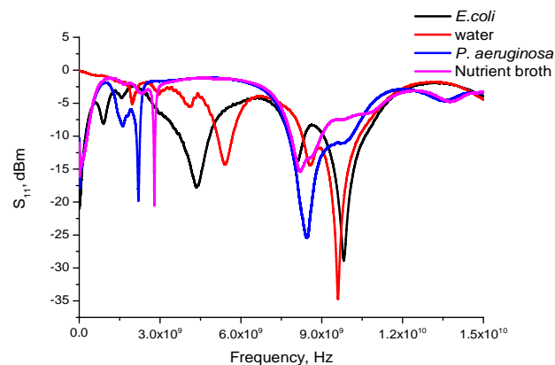
Figure 3. S_{11} signal distribution of microwave sensor in 0.01-15 GHz frequency range when in contact with deionised water, Escherichia coli , sterile nutrient broth and Pseudomonas aeruginosa solutions.
