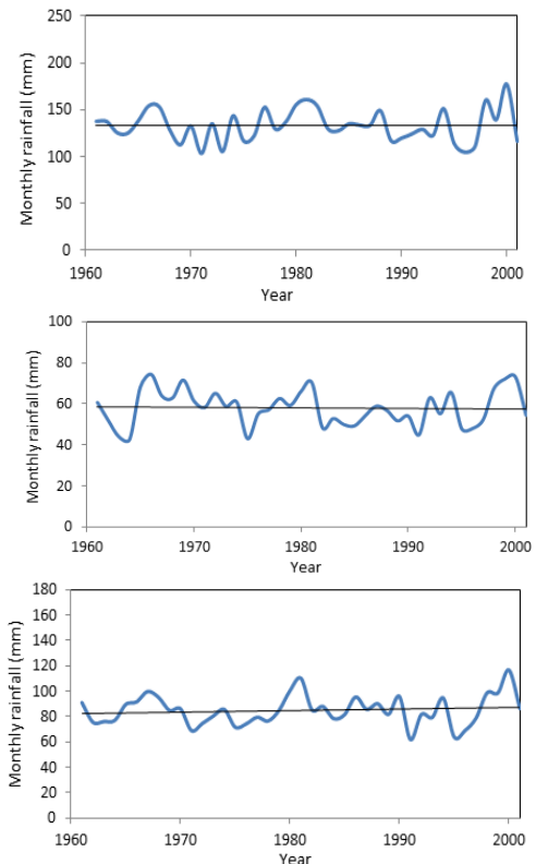
Fig. 5. The average monthly rainfall series with linear trend lines annual at Cumbria, Lancashire & Cheshire (top to bottom).
