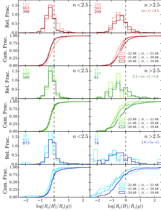
Figure 6. Effective radii of galaxies binned by absolute magnitude, for colour and Sérsic index subsamples. Panels and colours are chosen similar to Fig 3.
