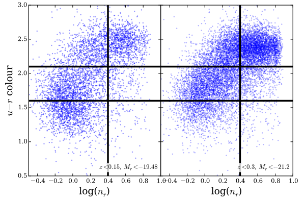
Figure 2. (u-r) rest frame colour vs. n_r for the galaxies in our two samples. Lines illustrate the cuts we apply to divide the galaxies by colour and Sérsic index.
