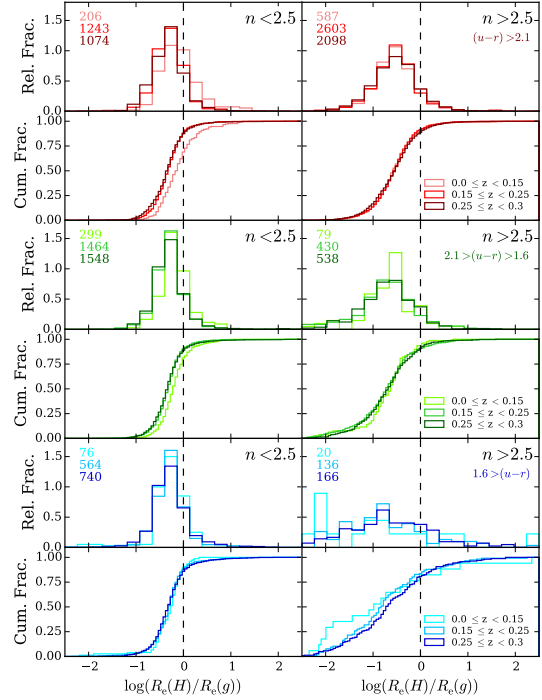
Figure 3. Effective radii of galaxies binned by redshift, for colour and Sérsic index subsamples. The left column shows low- n galaxies, the right column shows high- n galaxies. The top, middle and bottom groups of four panels contain red , green and blue samples, respectively. Within each group, the top panels show normalised histograms, whilst the bottom panels present corresponding cumulative histograms to better visualise subtle shifts in the distributions. In each panel lines in light colours show galaxies in the low redshift bin ( 0 \leq z < 0.15 ), mid-shades indicate the intermediate redshift bin ( 0.15 \leq z < 0.25 ), whilst the darkest colours show galaxies in the high redshift bin ( 0.25 \leq z < 0.3 ).
