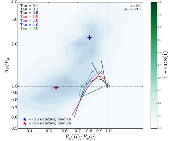
Figure 11. Dust corrected \mathcal{N}_g^H vs \mathcal{R}_g^H for discs. Underlaid are contours for all galaxies in the V14 sample, as in Fig. 9. Overplotted are the mean locations of low- and high- n galaxies within the V14 volume limited sample. Black lines show model tracks for optically thin discs having a nominal value (\mathcal{N}_g^H, \mathcal{R}_g^H) = (1, 1) , whilst coloured lines correspond to model tracks for optically thick discs. The intensity of the colour in each line shows the inclination of the galaxy. Crosses indicate the point at which (1 - \cos i) = 0.5 .
