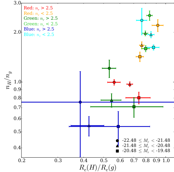
Figure 8. Median \mathcal{N}_g^H versus median \mathcal{R}_g^H for galaxies in each of our different subsamples divided by colour, Sérsic index and luminosity. Colours are the same as in figure 17 of V14.
