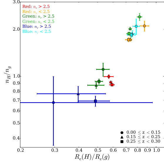
Figure 5. Median \mathcal{N}_g^H versus median \mathcal{R}_g^H for galaxies in each of our different subsamples divided by colour, Sérsic index and redshift bin. Colours are the same as in figure 17 of V14. Error bars show uncertainty on the median, estimated as 1.253\sigma/\sqrt{N} , where \sigma is the standard deviation about the median and N is the number of galaxies in the sample. There are small trends with redshift due to observational biases. However, the distinction between the subsamples, particularly the contrast between low- and high- n , remains very clear. Note that the blue 0 \leq z < 0.15 , n > 2.5 point lies at \mathcal{R}_g^H = 0.15 , \mathcal{N}_g^H = 0.56 , but is consistent with the higher z points given its large uncertainties.
