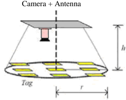
Fig 8 Recognition area of camera and RFID reader
