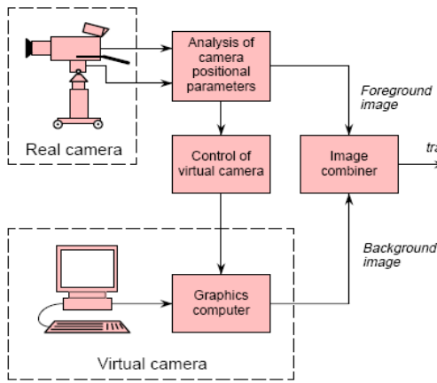
Fig 1 Camera tracking system for virtual studio
