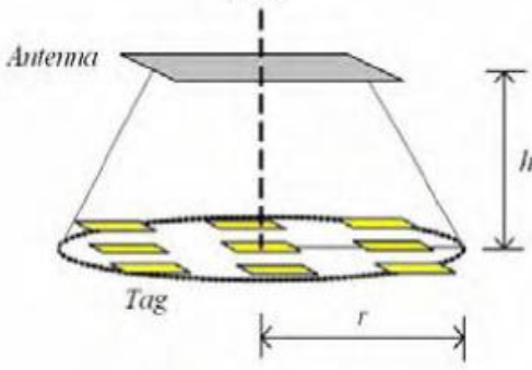
Fig 3 Recognition area model of RFID antenna.
