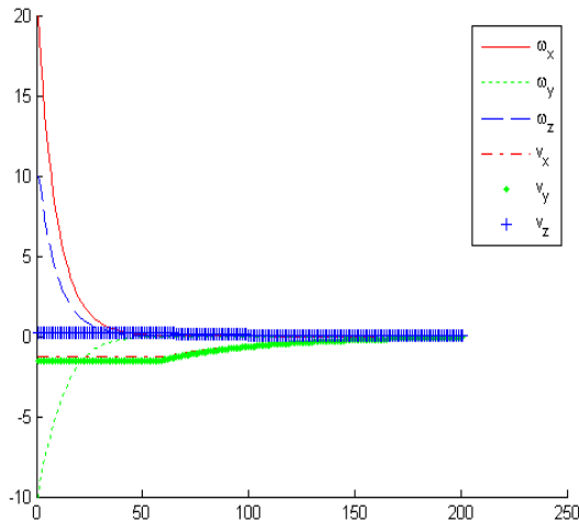
Fig 11 6DOF of camera extraction error
