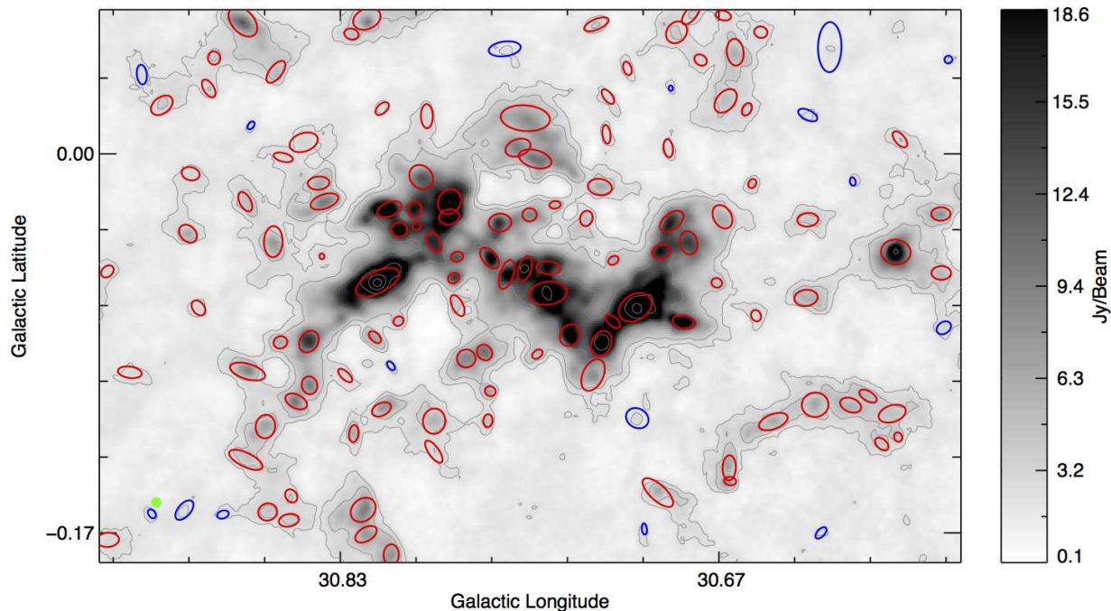
Figure 8. Example of the source-extraction results in a small portion of the \ell = 30^\circ region. The greyscale image shows the 850\text{-}\mu\text{m} emission and the red and blue ellipses show the approximate sizes and orientations of the sources above and below 5\sigma . The grey contours start at 3\sigma and increase in steps of 0.17, 0.8, 2.75, 6.81, 13.85 \text{Jy beam}^{-1} . The green filled circle in the lower-left corner indicates the FWHM size of the JCMT beam at 850\text{ }\mu\text{m} .
