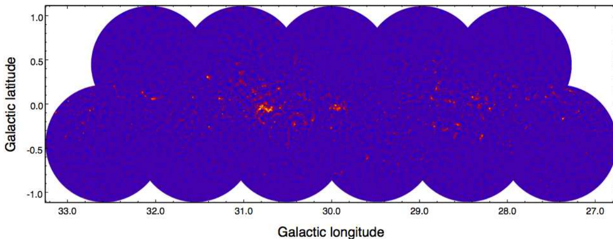
Figure 4. JPS 850- \mu\text{m} surface-brightness distribution in the \ell = 30^\circ field as of October 2013 with about 40 per cent of the data acquired. Individual circular pong tiles have been cropped at a radius of around 0.65^\circ . The bright sources near longitudes of 30.0^\circ and 30.8^\circ are the well-known star-forming regions G29.96 and W43, respectively. The colour scale range is logarithmic from zero to 23 \text{ Jy beam}^{-1}
