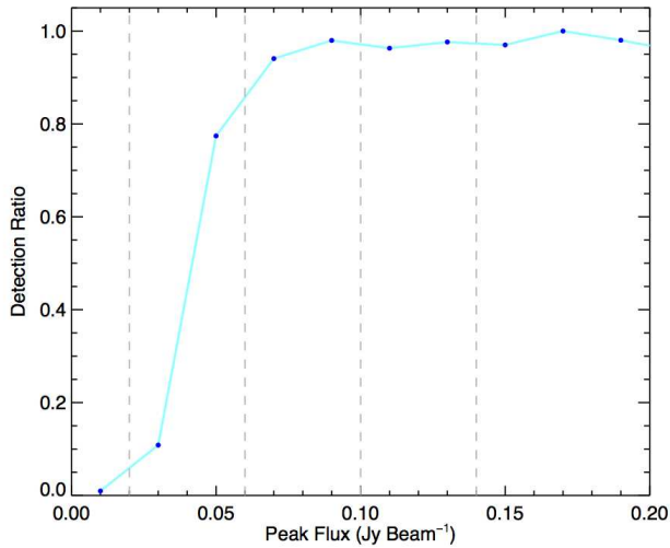
Figure 11. The ratio of recovered to injected source counts as a function of input peak flux density. The dashed vertical lines indicate (from left to right) the 1\sigma , 3\sigma , 5\sigma , and 7\sigma noise levels.
