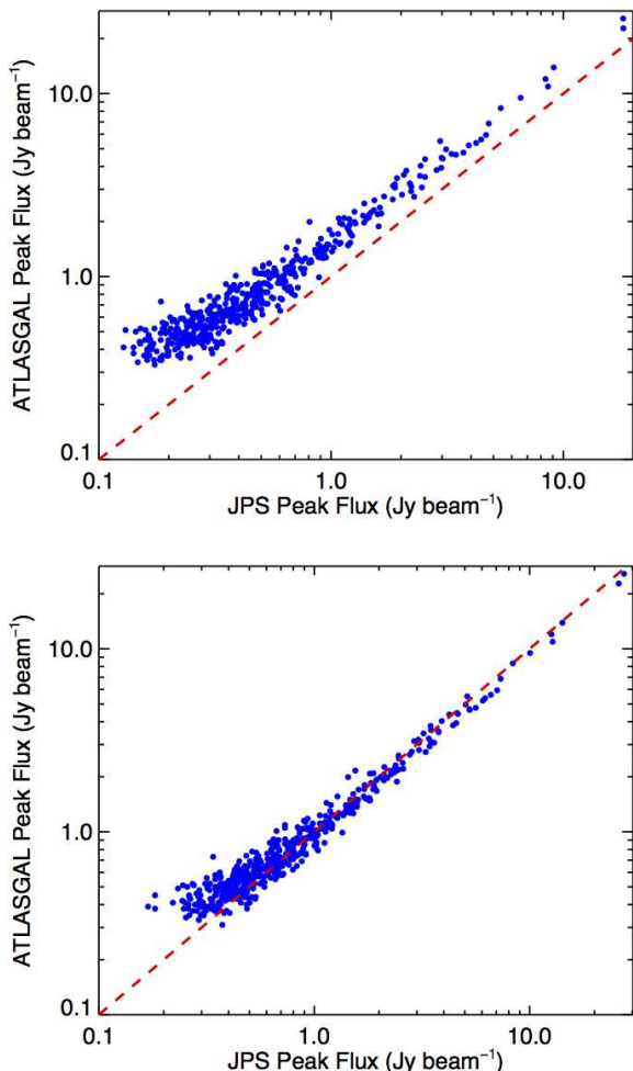
Figure 10. Comparison of the peak flux densities of extracted JPS sources to the corresponding ATLASGAL compact sources - top: unsmoothed data with 484 matches; bottom: with JPS data convolved to the resolution of ATLASGAL, producing 500 matches.
