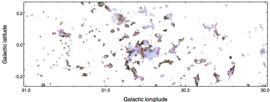
Figure 7. Spatial distribution of the ^{12}\text{CO J=3-2} emission line contamination in the region around W43. The colour scale shows the value of (S(850) - S(^{12}\text{CO}))/S(850) and the range is from 0.7 (darkest) to 1.0 (lightest).
