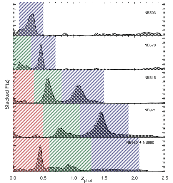
Figure 6. Stacked probability density distributions for each NB-selection of objects, shown over the redshift range relevant for this study. Red ( H\alpha ), green ([O III]) and blue ([O II]) shaded regions represent the redshift ranges assigned to a slice for a particular filter/line combination.
