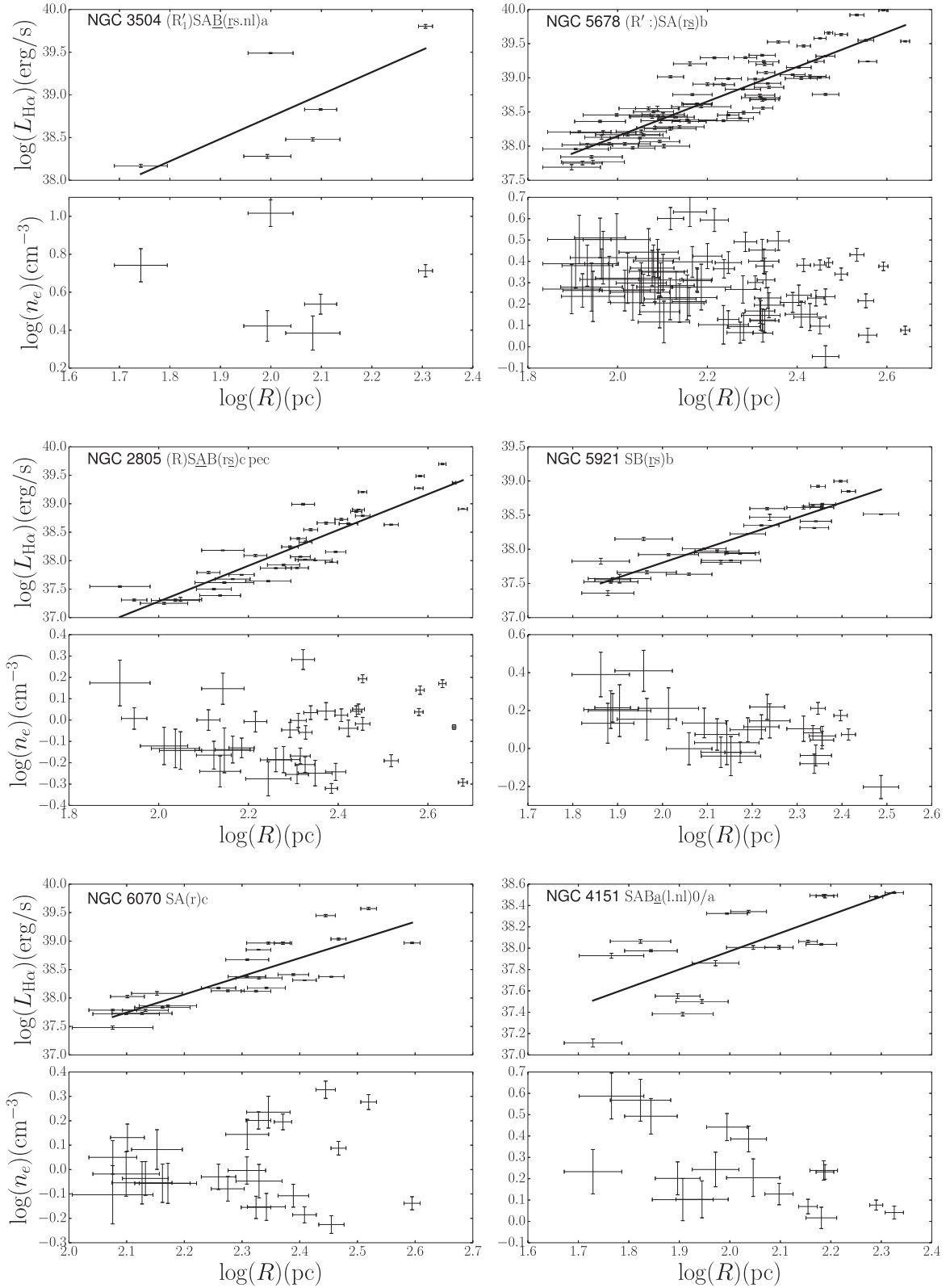
Figure 8. H \alpha luminosity, L_{H\alpha} , versus H II size (radius, R ) for isolated galaxies. The result of the double (or single) linear fit is drawn as a solid line. The n_e versus R of H II regions in isolated galaxies is plotted below each L_{H\alpha} – R plot.
