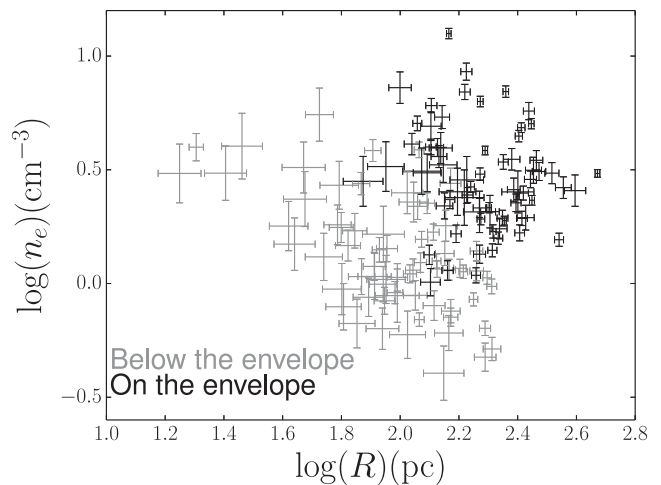
Figure 6. Left: H \alpha luminosity, L_{\text{H}\alpha} , versus velocity dispersion, \sigma_v , for H II regions in interacting galaxies. We have plotted the fitted envelope as a solid line, and the displaced envelope condition explained in the paper, as a dashed line. Right: electron density, n_e , versus the radius, R , for H II regions on the envelope (black) and those regions below the envelope (grey).
