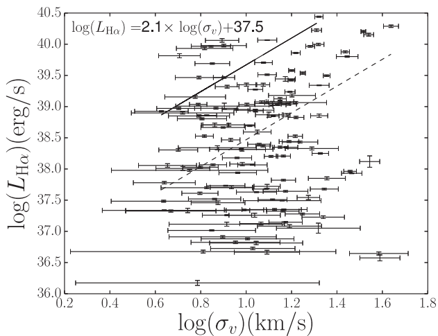
Figure 6. Left: H \alpha luminosity, L_{\text{H}\alpha} , versus velocity dispersion, \sigma_v , for H II regions in interacting galaxies. We have plotted the fitted envelope as a solid line, and the displaced envelope condition explained in the paper, as a dashed line. Right: electron density, n_e , versus the radius, R , for H II regions on the envelope (black) and those regions below the envelope (grey).
