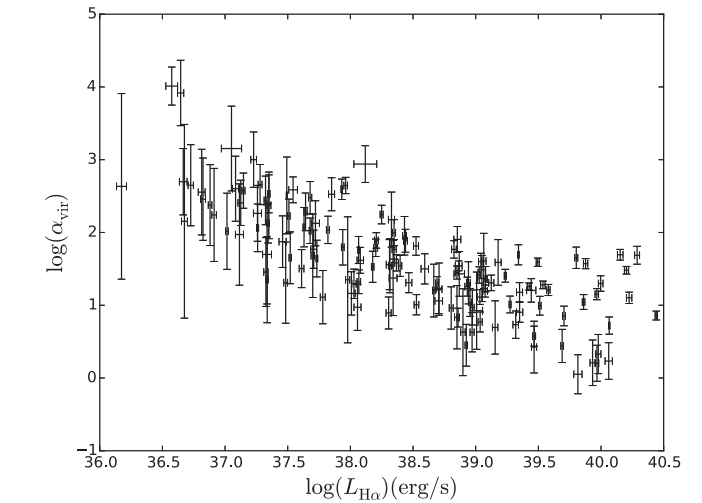
Figure 7. The virial parameter, \alpha_{\text{vir}} = 5 \frac{\sigma_v^2 R_{\text{HII}}}{G M_{\text{gas}}} versus H \alpha luminosity, L_{\text{H}\alpha} . We have used the mass of the ionized gas as the gas mass (in fact it should be a constant fraction of the total mass, but our qualitative conclusions do not depend on the value of this fraction, so we have not included it) M_{\text{gas}} = M_{\text{HII}} .
