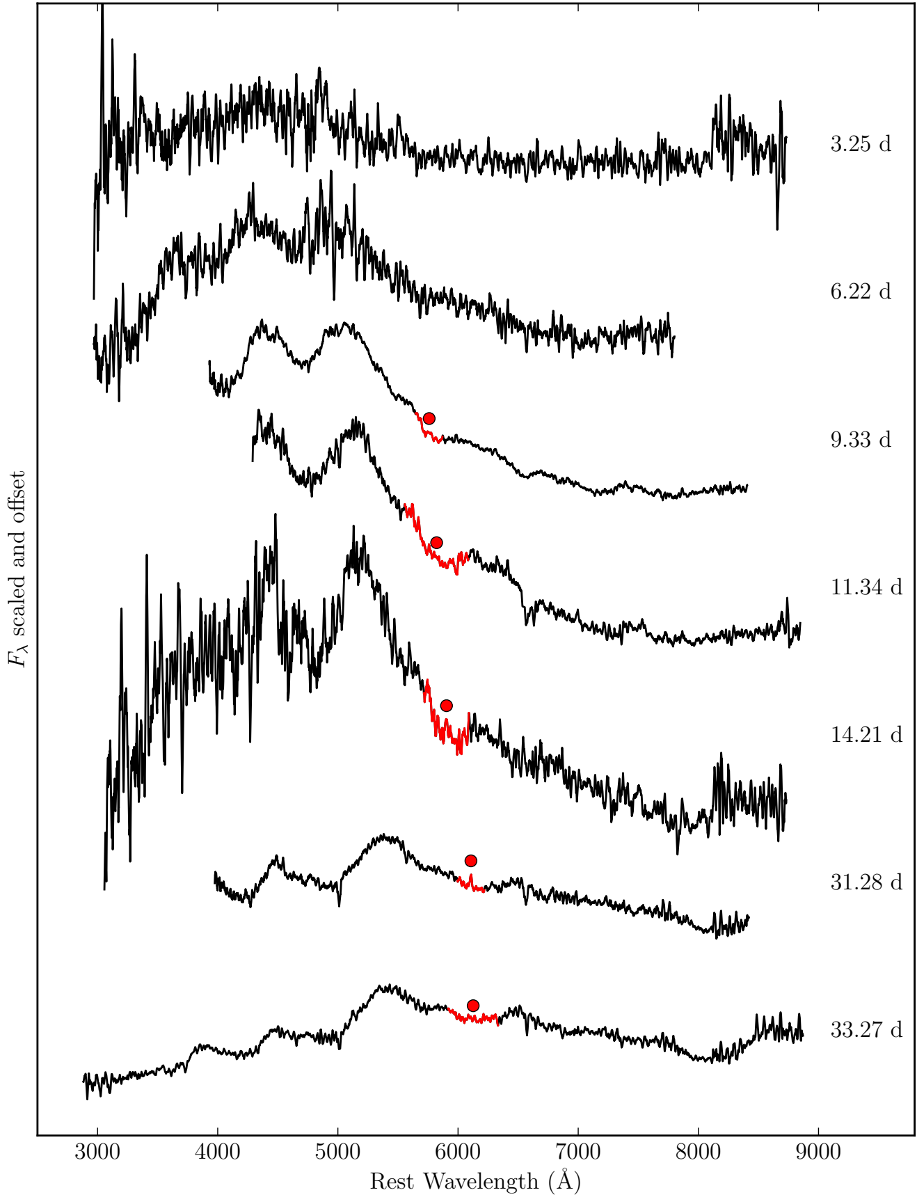
FIG. 5.— SN 2013dx spectra with host galaxy and GRB afterglow removed. They are smoothed using a Savitzky-Golay filter with a 30 \text{ \AA} window. We excluded the spectrum at t = 1.17 \text{ d} because it is dominated by the afterglow. Red filled circles mark the position of Si II \lambda 6355 calculated in § 5.3, used to determine the photospheric velocity of the ejecta. We have highlighted the Si II \lambda 6355 absorption feature in red.
