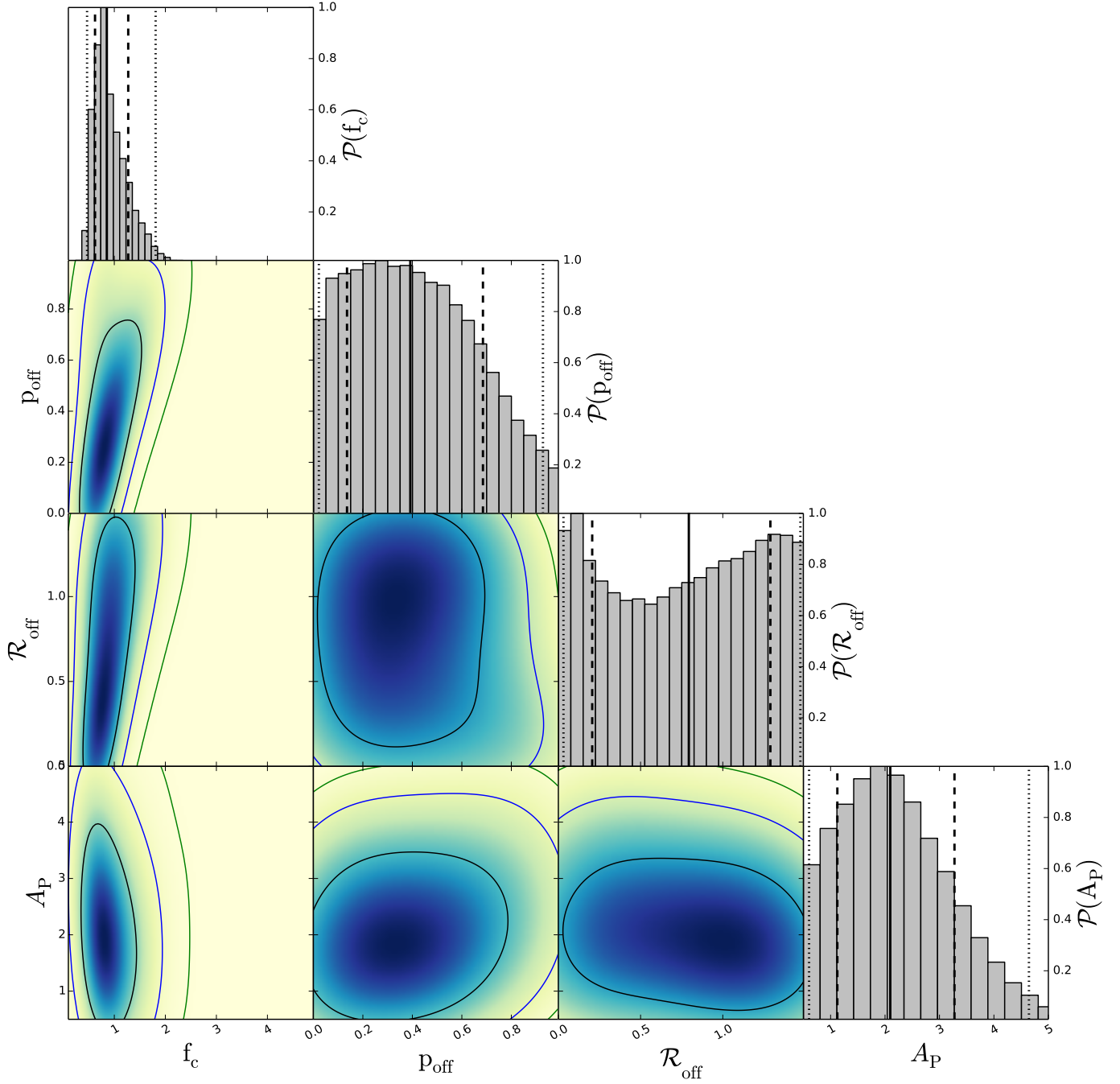
Figure 9. Posterior distribution of the normalisation of the mass-concentration relation f_c , of the mis-centring parameters P_{\text{off}} and R_{\text{off}} and of the amplitude of the point mass A_P . The contours indicate the 1, 2, 3 sigma confidence regions. The dashed vertical lines and the dotted vertical lines correspond respectively to the 1 and 2 sigma marginalised confidence limits. These are the constraints from a joint halo model fit of the ESD signal in the 6 luminosity bins using BCG as the group centre. The range in each panels reflect the priors used for the different parameters.
