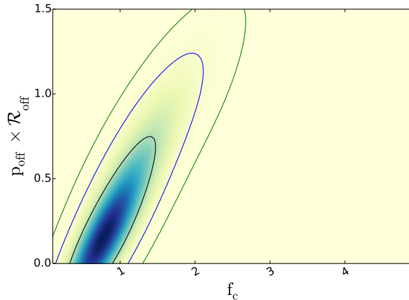
Figure 11. 2D posterior distribution of the average projected offset ( p_{\text{off}} \times \mathcal{R}_{\text{off}} ) and the normalisation of the concentration-halo mass relation f_c . The contours indicate the 68%, 95% and 99% confidence region.
