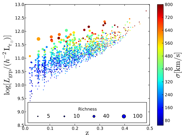
Figure 3. Total group r-band luminosity as a function of the redshift of the group. The size of the points is proportional to the group apparent richness and the colour of the points indicates the group velocity dispersion corrected for velocity uncertainty. The shape of the distribution is typical of a flux limited survey.
