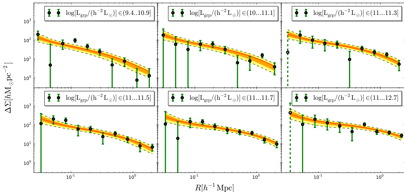
Figure 7. Stacked ESD profile measured around the groups BCG of the 6 group luminosity bins as a function of distance from the group centre. The group r-band luminosity increases from left to right and from top to bottom. The stacking of the signal has been done using only groups with N_{\text{fof}} \geq 5 . The error bars on the stacked signal are computed as detailed in section 3.4 and we use dashed bars in the case of negative values of the ESD. The orange and yellow bands represent the 68 and 95 percentile of the model around the median, while the red line shows the best fit model.
