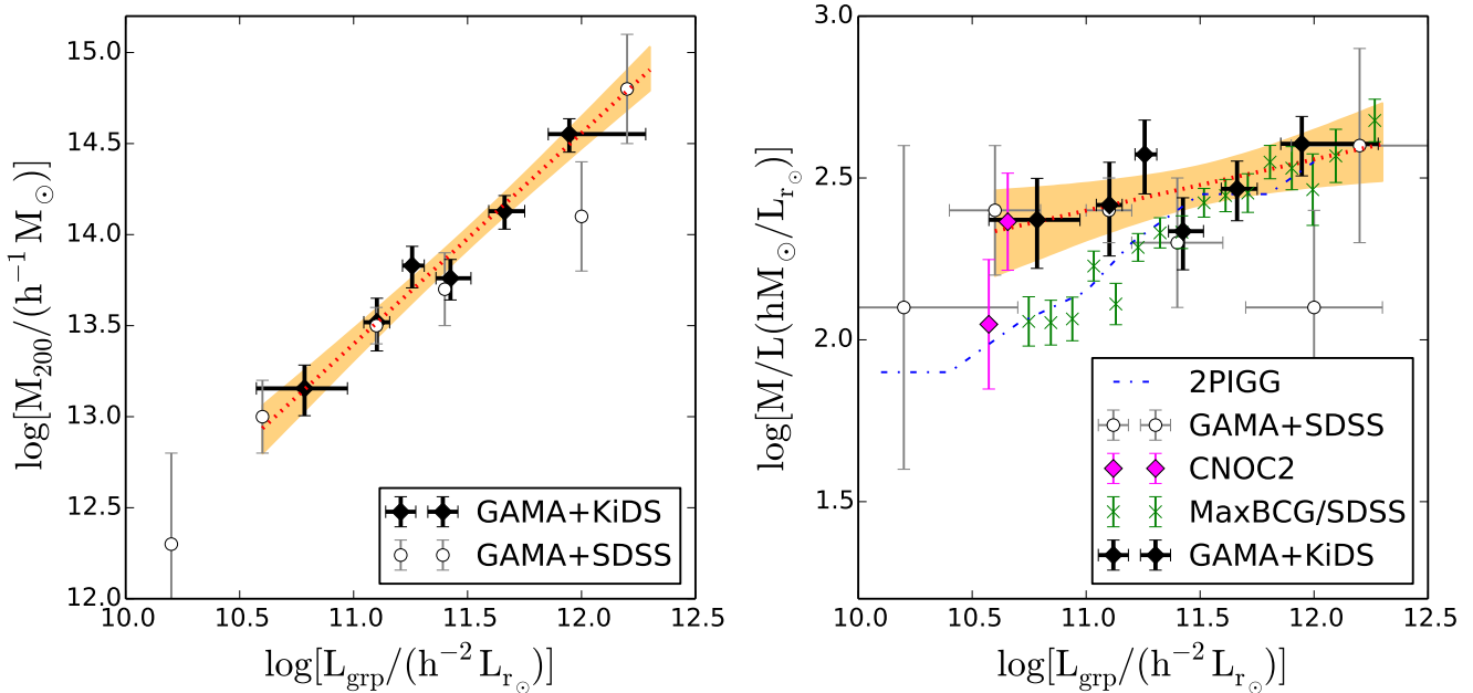
Figure 13. Left panel: Halo mass as a function of the total group r-band luminosity. The solid black points show the halo masses derived in this work from a halo model fit to the stacked ESD profile of groups with at least 5 members brighter than the GAMA magnitude limit. The vertical error bars indicate the 1-sigma uncertainty on the average halo mass after marginalising over the other halo model parameters, while the horizontal error bars indicate the 16th and 84th percentile of the luminosity distribution in each bin. The red line shows the best fit power-law to the data points, while our estimate of the 1-sigma dispersion around this relation is shown as the orange area (see text). The open black circles show the halo masses derived from a lensing analysis of GAMA groups using SDSS galaxies as background sources (Han et al. 2014). Right panel: Derived mass-to-light ratio as a function of the group total luminosity from this work (black points), from the GAMA+SDSS analysis (open black circles), from the analysis of the CNOC2 group sample (Parker et al. 2005) (magenta diamonds) and from a lensing analysis of 130000 groups from the MaxBCG catalogue using SDSS imaging (Sheldon et al. 2009, (green crosses)). In blue we show the median relation derived using the 2PIGG catalogue (Eke et al. 2004). The red lines and the orange area correspond to those of the left panel.
