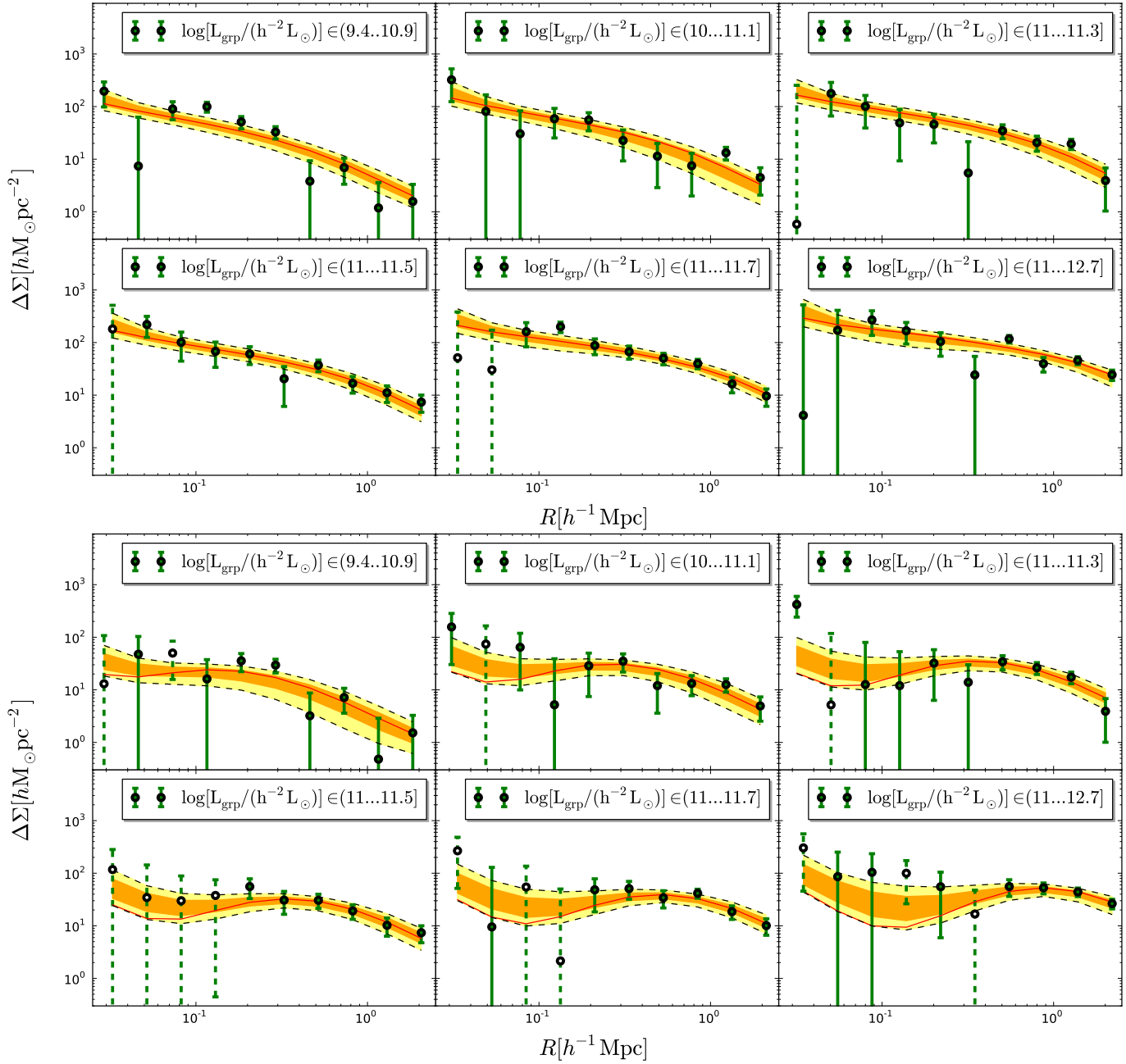
Figure A1. Stacked ESD measured around the groups' IterCen (upper panel) and the groups' centre of light Cen (lower panel) for 6 group luminosity bins as a function of distance from the group centre. The group luminosity increases from left to right and from top to bottom. The stacking of the signal has been performed considering only groups with N_{\text{fof}} \geq 5 . The error bars on the stacked signal are computed as detailed in section 3.4. The orange and yellow bands represent the 68 and 95 percentile of the model around the median and the red lines indicate the best fit model.
