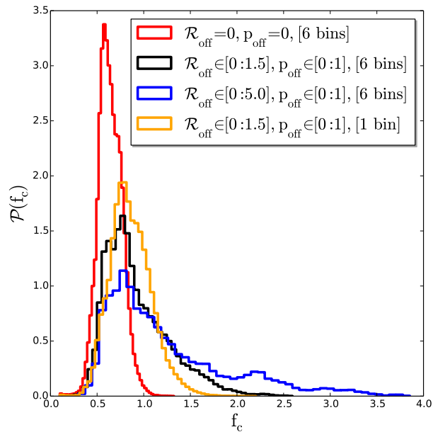
Figure 12. Posterior distribution for the normalisation of the mass-concentration relation (Duffy et al. 2008) after marginalising over the other model parameters. We show here the effect of changing the prior in the miscentring parameters: \mathcal{R}_{\text{off}} = 0 (red line), \mathcal{R}_{\text{off}} \in [0..1.5]r_s (black line) and \mathcal{R}_{\text{off}} \in [0..5]r_s (blue line). As a reference, the orange line shows the posterior distribution for f_c in the case of a global stack of all groups. This has to be compared with the black line, where the constraints were derived from a joint fit of the stacked ESD in 6 luminosity bins.
