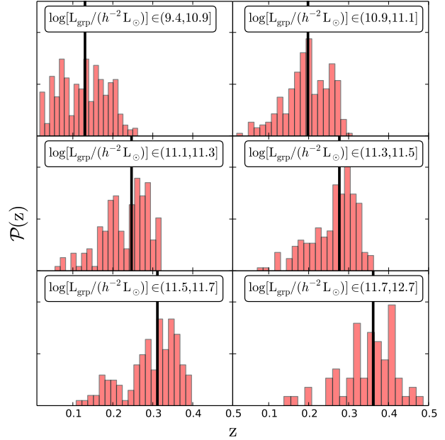
Figure 6. Redshift distributions of the GAMA groups used in this paper in the six r-band luminosity bins. The group luminosity increases from left to right and from top to bottom. The solid vertical black lines indicate the median of the distributions.
