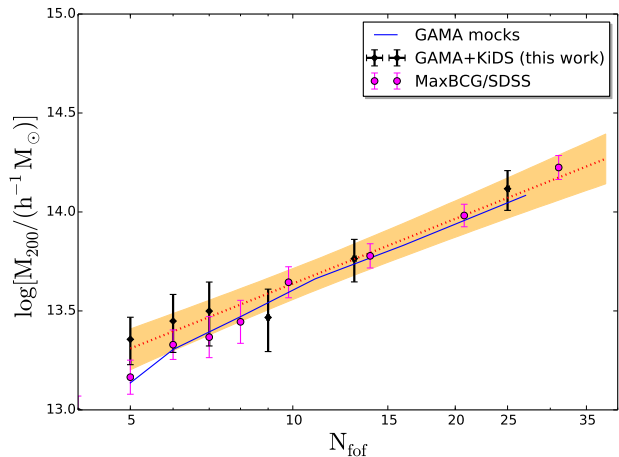
Figure 16. Group halo mass as a function of the richness ( N_{\text{fof}} ). We use here only groups with at least 5 members brighter than r_{AB} = 19.8 . The richness of the groups is not corrected to account for the fainter galaxies not targeted by GAMA. The red line shows the best fit power-law relation to the data points. Our estimate of the 1-sigma dispersion around this relation is shown as the orange area. The blue line shows the mass-richness relation derived from the GAMA mocks using the same selection function applied to the data. The magenta points show the result of a weak lensing analysis of 130,000 groups and clusters of galaxies in the Sloan Digital Sky Survey (Johnston et al. 2007).
