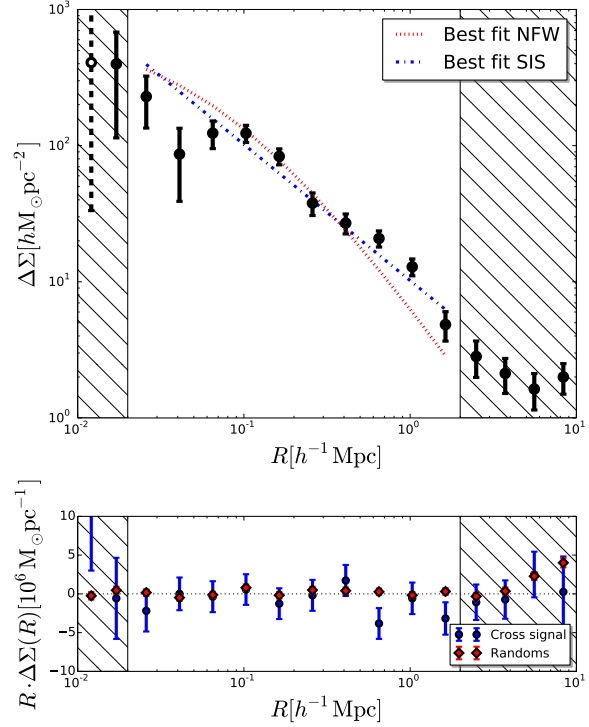
Figure 4. Top panel: ESD profile measured from a stack of all GAMA groups with at least 5 members (black points). Here, we choose the Brightest Cluster Galaxy as the group centre. The open white circle with dashed error bars indicates a negative \Delta\Sigma . The dotted red line and the dash-dotted blue line show the best fits to the data of NFW (Navarro, Frenk & White 1995) and singular isothermal sphere profiles, respectively. Neither of the single-parameter models provides a good fit to the data, highlighting that complex modelling of the signal is required. Bottom panel: ESD profile, multiplied by R to enhance features at large radii, measured from the cross-component of the ellipticities for these same groups (blue points) and measured around random points using the same redshift distribution of the groups (red points). We only use measurements at scales outside the dashed areas for the rest of the paper.
