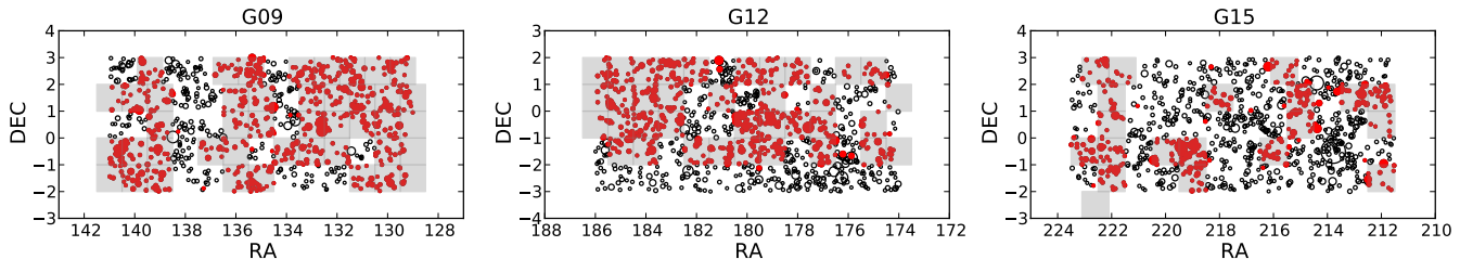
Figure 1. KiDS-ESO-DR1/2 coverage of the three equatorial GAMA fields (G09, G12, G15). Each grey box corresponds to a single KiDS tile of 1 square degree. The black circles represent groups with N_{\text{fof}} \geq 5 in the G^3\text{Cv7} catalogue (R+11). The size of the dots is proportional to the group apparent richness. The filled red circles indicate the groups used in this analysis. These are all groups either inside a KiDS field or whose centre is separated less than 2 h^{-1} \text{Mpc} from the centre of the closest KiDS field.
