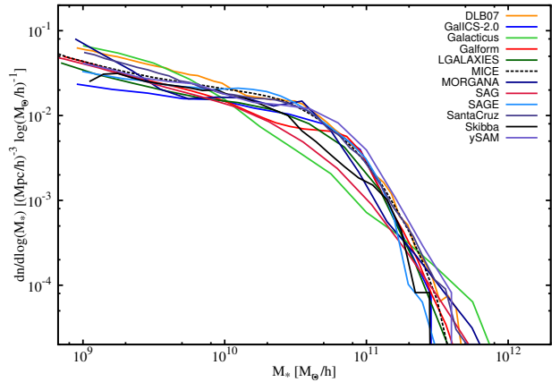
Figure 5. Stellar mass function at redshift z = 0 for all the models when created in the native environment used during the model calibration. All curves have been corrected for the IMF towards Chabrier. This figure uses the same scale as (and should be compared to) Fig. 4.
