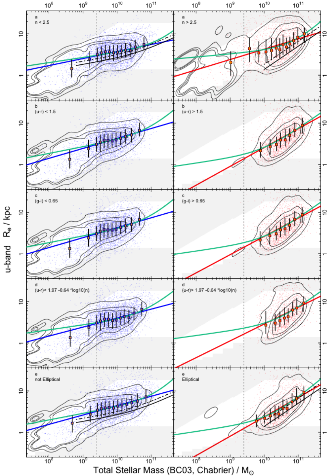
Figure A1. The u -band M_* - R_e relation for late and early-types - left and right hand side respectively. We are using a) the Sérsic index, b) the (u-r)_{stars} colour, c) the (g-i)_{stars} colour, d) a combination of Sérsic index and (u-r)_{stars} colour and e) the visual morphology to divide the populations as described in the paper. Fitting parameters can be found in Tables 2 and 3.
