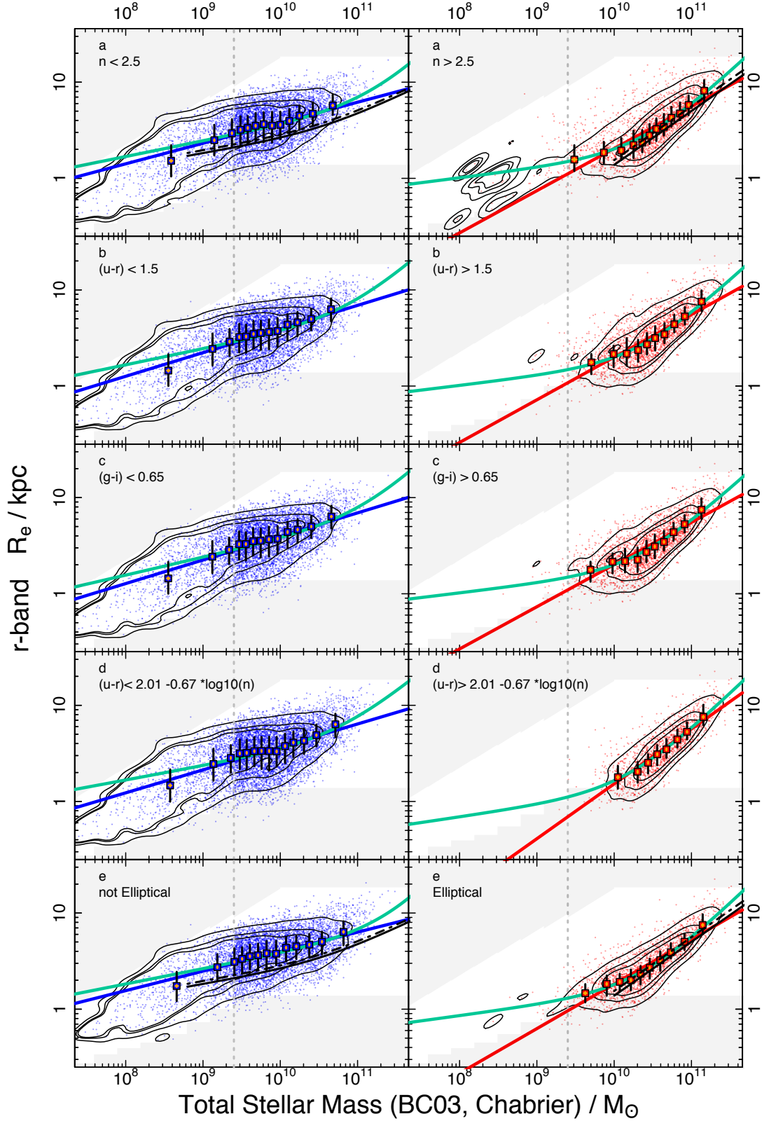
Figure 3. The \mathcal{M}_* - R_e relation for early- (red, right hand side) and late- (blue, left hand side) type galaxies divided by: a) Sérsic index n=2.5 ; b) Dust corrected colour (u-r)_{stars}=1.5 ; c) Dust corrected colour (g-i)_{stars}=0.65 ; d) Rolling Sérsic index division and e) Visual Elliptical/Not-Elliptical classification. The red and blue lines are single power-law fits to the binned data (Eq. 2), the green lines are two component power-law fits (Eq. 3) and the grey dotted line indicates the lower mass limit highlighting the wealth of data that would have been ignored. The grey shaded areas indicate where measurements become less reliable due to our detection limitations. The black solid and dot-dashed lines in panels a) and e) show the S03 \mathcal{M}_* - R_e relation where the dot-dashed line shows the sizes corrected from z - to r -band values and the solid line shows the relation as is. For the fitting parameters see Tables 2 and 3.
