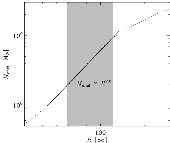
Figure A1. Enclosed mass as a function of galactocentric radius in the range R = 30\text{--}300 pc from Launhardt, Zylka & Mezger (2002, dotted line). The grey region shows the radial range spanned by the best-fitting pericentre and apocentre distances, whereas the solid line shows a power-law fit to the enclosed mass profile in the radial range spanned by our best-fitting pericentre (minus one standard deviation) and apocentre (plus one standard deviation).
