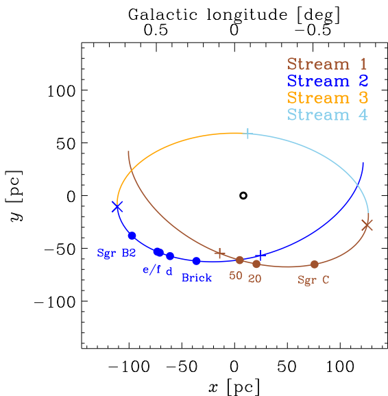
Figure 6. Top-down view of our orbital model (solid line), with the observer located in the negative- y direction. As in Figures 2 and 4, the colours refer to the four coherent streams in position-velocity space. The dots indicate the implied positions in the Galactic plane of several GMCs and cloud complexes in the CMZ, the plus symbols indicate pericentres, the crosses mark apocentres, and the open black circle denotes the position of Sgr A*. Note that we only show the part of the orbit that is currently associated with the observed gas structure – in the future, the gas stream (or its star formation products) will continue on the same rosetta-like orbit, beyond the end of Stream 1 shown here.
