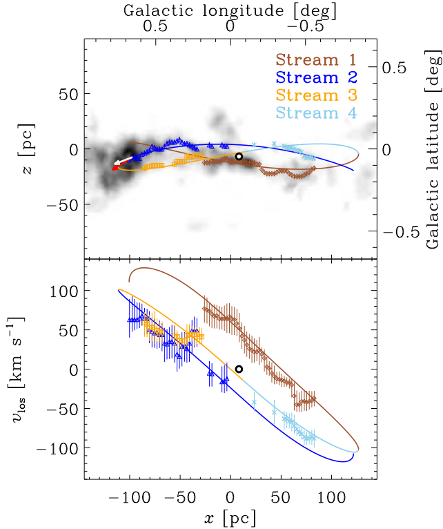
Figure 4. Comparison of our orbital model (solid line) with the observed integrated-intensity map of \text{NH}_3(1,1) emission near the Galactic Centre, tracing gas with volume densities n > several 10^3 \text{ cm}^{-3} (grey scale). Symbols with error bars show the coherent phase-space structure (see §2.2) to which the model was fitted. We have divided the gas into four coherent streams in position-velocity space that are colour-coded as indicated by the legend. In our model, the back side of the gas stream consists of Streams 3 and 4, whereas Streams 1 and 2 represent the two (independent) ends of the stream on the front side. The open black circle denotes the position of Sgr A*. The model starts at Stream 2 (the overlap with Stream 4 is coincidental but could fit too) and continues through Streams 3 and 4 to Stream 1. Top panel: Distribution in Galactic longitude and latitude \{l, b\} . The red arrow indicates the observed proper motion vector of Sgr B2 and the bright yellow arrow represents the model prediction. Bottom panel: Distribution in Galactic longitude and line-of-sight velocity \{l, v_{\text{los}}\} .
