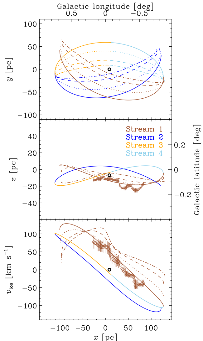
Figure 7. Comparison of the observed \text{NH}_3(1,1) emission of Stream 1 with our orbital model (lines) for different pericentre radii R_p . The {dash-dotted, dashed, dotted, solid} lines indicate pericentre radii of R_p = \{10, 20, 40, 59\} pc, where the latter value corresponds to our best-fitting model. As before, the colours refer to the four coherent streams in position-velocity space. The open black circle denotes the position of Sgr A*. Top row: Distribution in Galactic longitude and along the line of sight \{x, y\} . The different projected apocentre radii arise due to different heights above the plane. Middle row: Distribution in Galactic longitude and latitude \{l, b\} . Note the different scale on the y -axis compared to earlier figures. Bottom row: Distribution in Galactic longitude and line-of-sight velocity \{l, v_{\text{los}}\} . The middle and bottom panels show the effect of a changing pericentre radius only for Stream 1.
