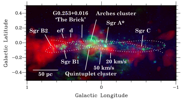
Figure 5. Repeat of the three-colour composite of the CMZ from Figure 1. This time, the white dotted line shows our best-fitting orbit. Note that the clouds near l = -1^\circ have v_{\text{los}} \sim \{0, 140\} \text{ km s}^{-1} (bottom and top, respectively) and hence are not associated with the gas stream that the model was fitted to.
