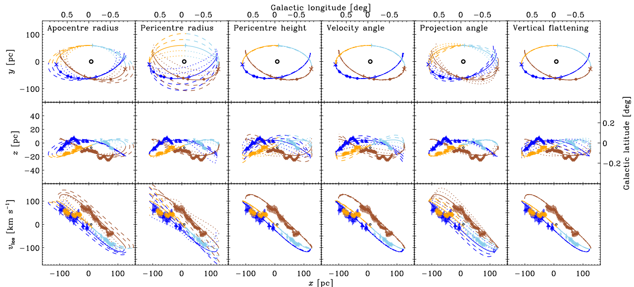
Figure B1. Comparison of the observed \text{NH}_3(1, 1) emission (symbols with error bars, tracing gas with volume densities n > \text{several } 10^3 \text{ cm}^{-3} ) near the Galactic Centre with our orbital model (solid line). The two dotted (dashed) lines indicate the effect of decreasing (increasing) the parameter indicated at the top left of each column by 1\sigma and 2\sigma (see Table 1). As in Figures 2, 4 and 6, the colours refer to the four coherent streams in position-velocity space. The open black circle denotes the position of Sgr A*. Top row: Distribution in Galactic longitude and along the line of sight \{x, y\} . Dots are positioned along the best-fitting orbital model to indicate the longitudes of the clouds discussed in §4.1 and Figure 6, whereas crosses (plus symbols) mark the apocentres (pericentres). Middle row: Distribution in Galactic longitude and latitude \{l, b\} . Bottom row: Distribution in Galactic longitude and line-of-sight velocity \{l, v_{\text{los}}\} .
