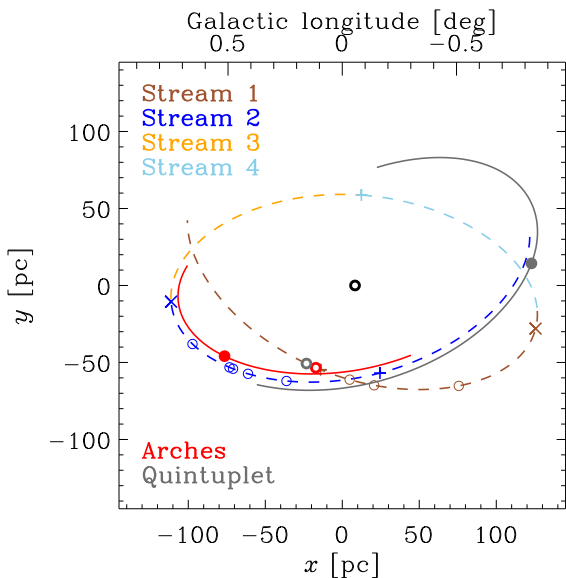
Figure 8. Top-down view of the present and past of the Arches and Quintuplet clusters in the context of our orbital model (dashed line). As in Figure 6, the observer is located in the negative- y direction. The colours again refer to the four coherent streams in position-velocity space, the thin circles indicate the implied positions in the Galactic plane of several GMCs and cloud complexes in the CMZ, the plus symbols indicate pericentres, the crosses mark apocentres, and the open black circle denotes the position of Sgr A*. The present-day positions of the Arches and Quintuplet clusters are represented by the thick circles on Stream 1, close to pericentre. The formation sites of these clusters as implied by their ages are indicated by the solid dots on lines running in parallel to the orbital model. The lengths of the lines indicate the uncertainty ranges implied by the age measurements.
