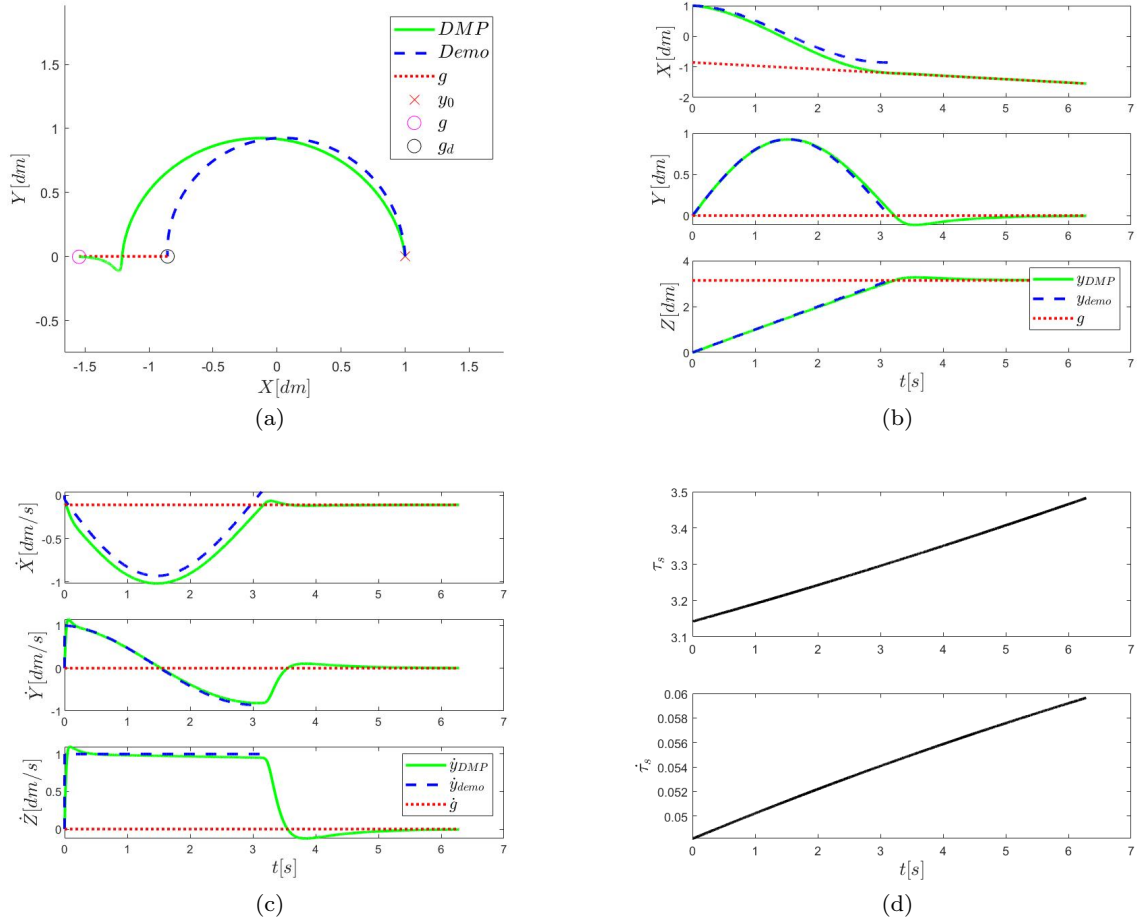
Fig. 4 In (a), the blue line is the human demonstration trajectory; the green line is the reproduced trajectory by DMPs; the red dash line represents the moving target. b The position trajectory generated by demonstration and DMP; the red dash line is the goal's position trajectory. c The velocity trajectory generated by demonstration and DMP; the red dash line is the goal's velocity trajectory. d Provides the evolution of the temporal coefficient and its derivative.
