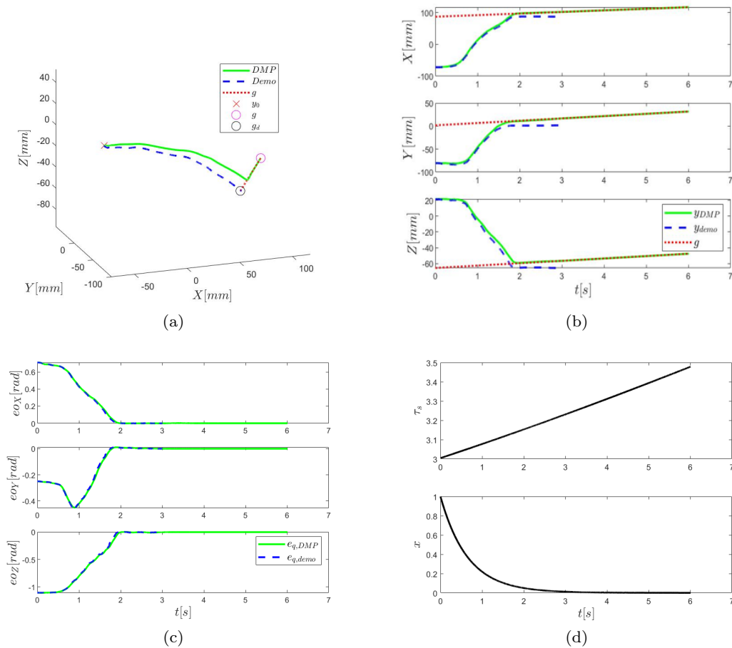
Fig. 7 a 3D trajectory. The blue and green lines in b show the demonstration and DMP trajectory in each direction; the red dash line is the goal trajectory in XYZ directions. c The orientation error between the current orientation and the goal orientation. d provides the evolution of the temporal coefficient and the phase variable x with time.
