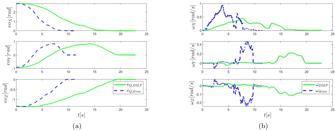
Fig. 6 (a) Pose of Omni: the blue line is the demonstration trajectory; the green one is the output of DMP when the execution time is set twice the demonstration one; b provides the angular velocity generated by demonstration and DMP
