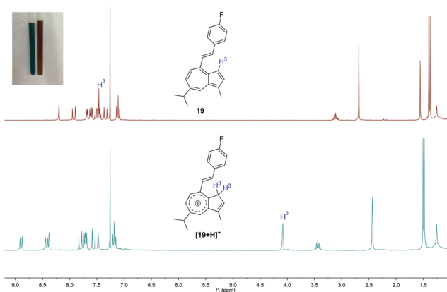
Fig. 4 Top: ^1\text{H} -NMR spectrum of 19 in \text{CDCl}_3 . Bottom: ^1\text{H} -NMR spectrum of 19 in TFA/ \text{CDCl}_3 1 : 9. Inset: NMR tubes containing 19 in \text{CDCl}_3 (left) and 19 in TFA/ \text{CDCl}_3 (right).
