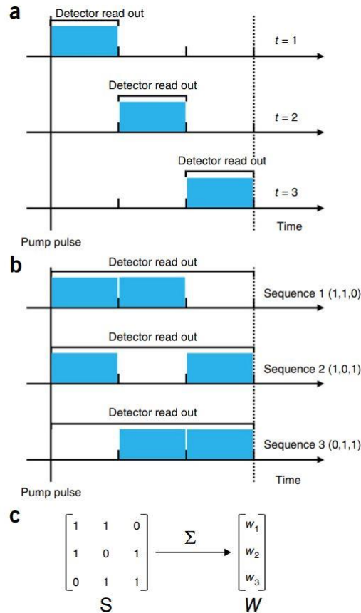
Fig. 4. (a) The time sequence for the classical pump-probe method showing three time delays. (b) The simplest Hadamard pulse sequence set up to measure three time points. (c) The 3 \times 3 Hadamard \mathbf{S} matrix showing how each row produces a single summed intensity for each reflection on the detector ( w_1, \dots, w_n ) forming the vector \mathbf{W} . Figure reproduced from ref [28] with permission from Nature Methods.
