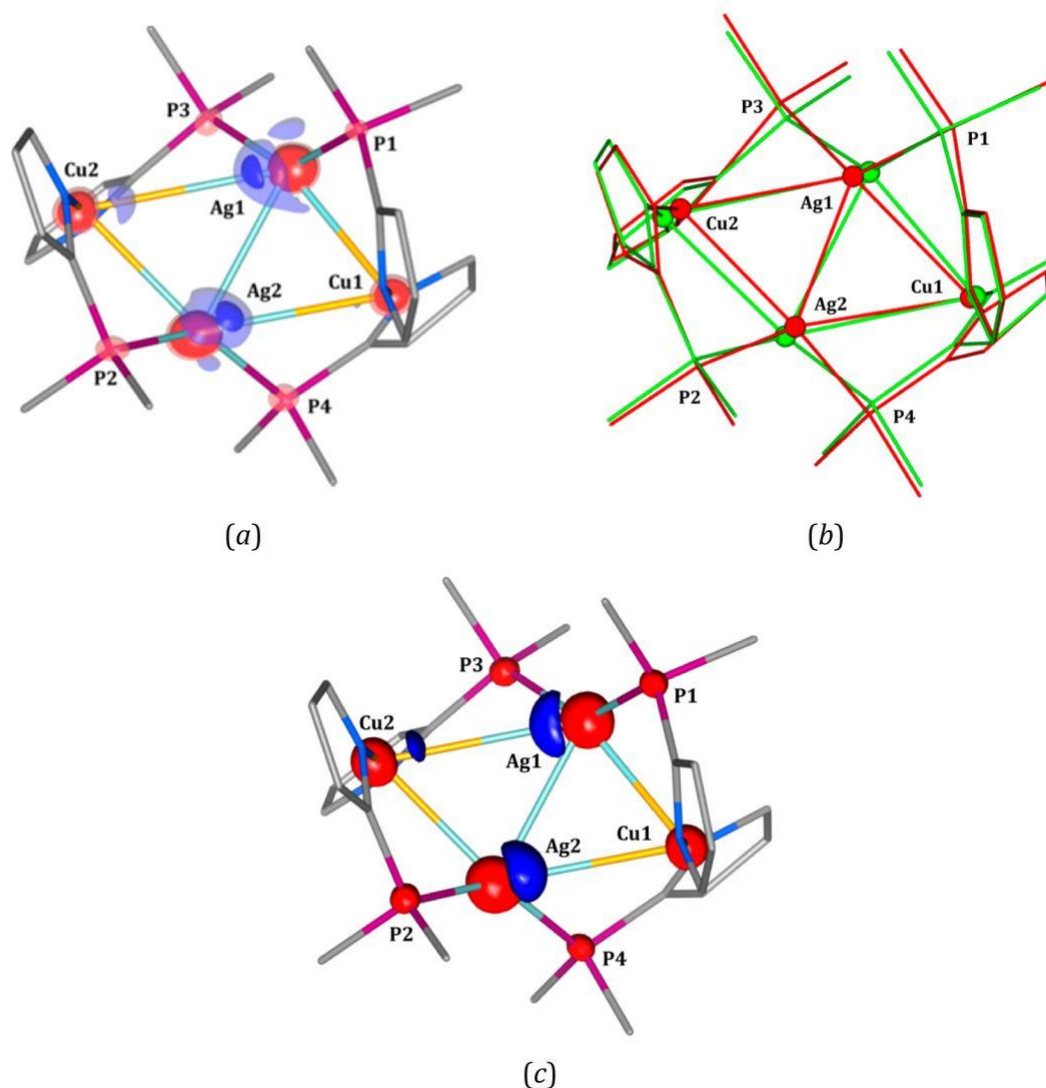
Fig. 10. a) Photodifference map ( F_o^{ON} - F_o^{OFF} ) of the complex showing atomic shifts upon excitation (solid isosurfaces, \pm 0.55 \text{ e} \cdot \text{\AA}^{-3} ; semi-transparent, \pm 0.35 \text{ e} \cdot \text{\AA}^{-3} ; blue, positive; red, negative). (b) Refined excited-state geometry related to that of the ground-state crystal structure (green, ground state; red, excited state; methylindole ligands were omitted for clarity). (c) Photodeformation map ( F_c^{ON} - F_c^{OFF} ) based on the refined model parameters (isosurfaces, \pm 0.30 \text{ e} \cdot \text{\AA}^{-3} ; blue, positive; red, negative; k_B = 1.06 ). Reproduced with permission from ref [134].
