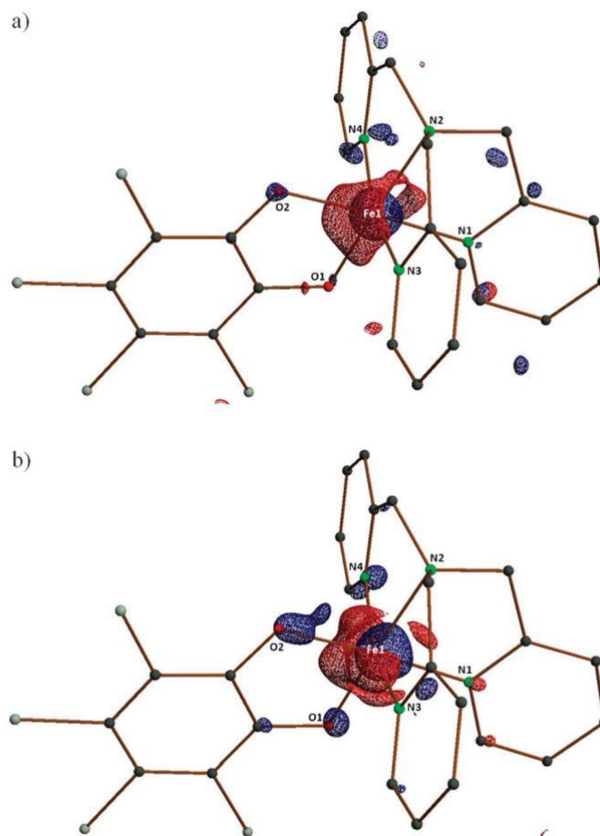
Fig. 11. Photodifference maps obtained for the monoclinic polymorph with isosurfaces (red positive, blue negative) of (a) \pm 0.14 \text{ e}\text{\AA}^3 for the 500 ps data and (b) \pm 0.46 \text{ e}\text{\AA}^3 for the 50 \mu s data. Reproduced with permission from ref [39].
