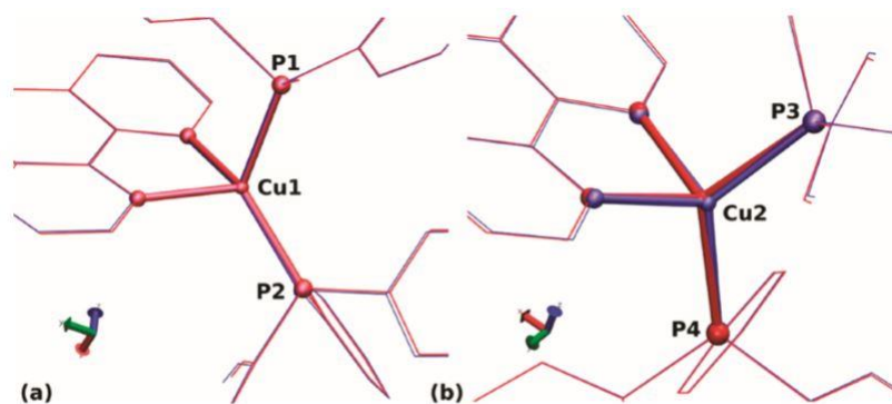
Fig. 9. Comparison of the ground state (in blue) and the excited state (in red) structures of the two independent molecules at 90 K. (a) molecule A; (b) molecule (b). Reproduced with permission from ref [131].
