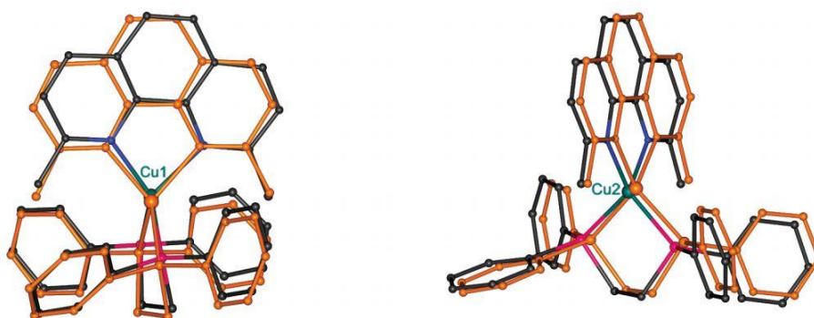
Fig. 8. Excited state geometries of the two independent molecules (orange) superimposed on the ground state of the complex (Cu, green; C, black; P, purple; N, blue). Slightly different views are shown to
