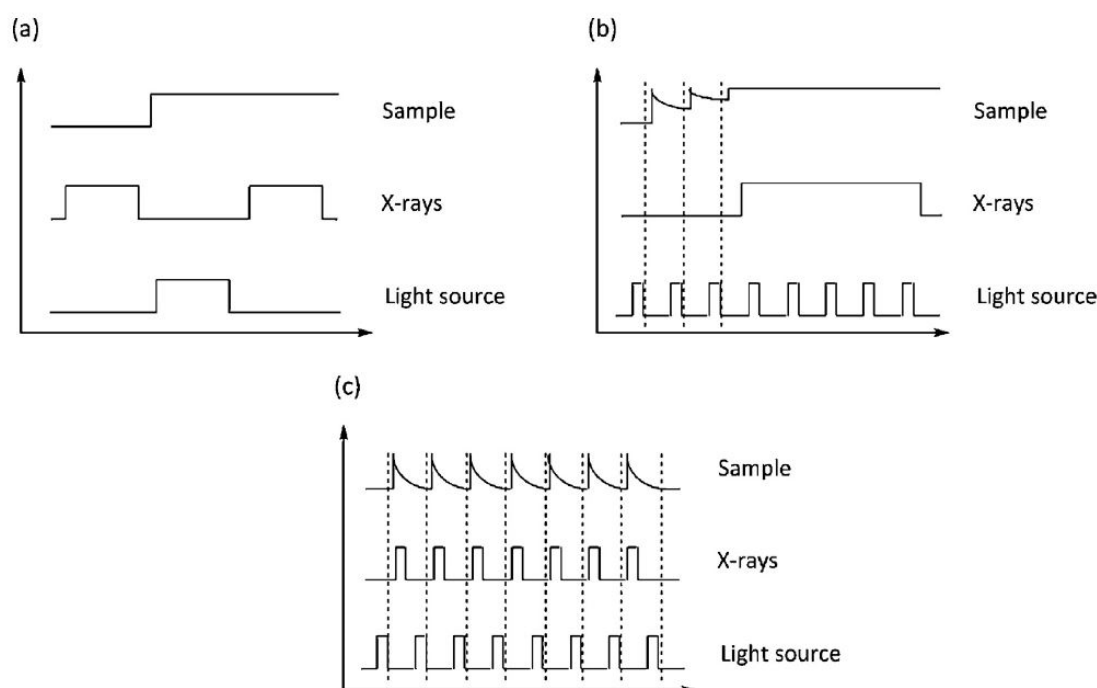
Fig. 3. Schematic diagrams to show the timing sequences used in the different types of photocrystallographic experiments: (a) steady-state methods, (b) pseudo-steady state methods, and (c) pump-probe methods. Taken from reference [18] with permission from Elsevier.
