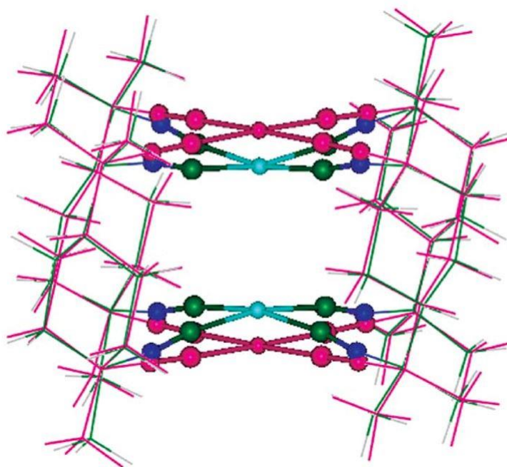
Fig. 7. Theoretical ground state (in pink) and excited state (green and blue colours) geometries of the [\text{Rh}_2(1,8\text{-diisocyanomenthane})_4]^{2+} cation. Reproduced with permission from ref [82].
