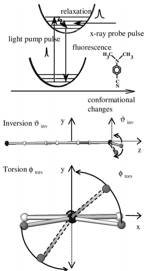
Fig. 6. Top: The principle of TR X-ray diffraction on the excited state PES of DMABN crystals. Bottom: the intramolecular degrees of freedom, which contribute to the relaxation process (inversion \vartheta_{\text{inv}} and torsion \phi_{\text{tors}} ). C atoms of the phenyl moiety are given as open, N atoms as black, and the amino C as grey circles. Note that the H atoms are not shown, since they do not contribute to the X-ray diffraction signal. Reproduced from ref [108] with permission from the ACS.
