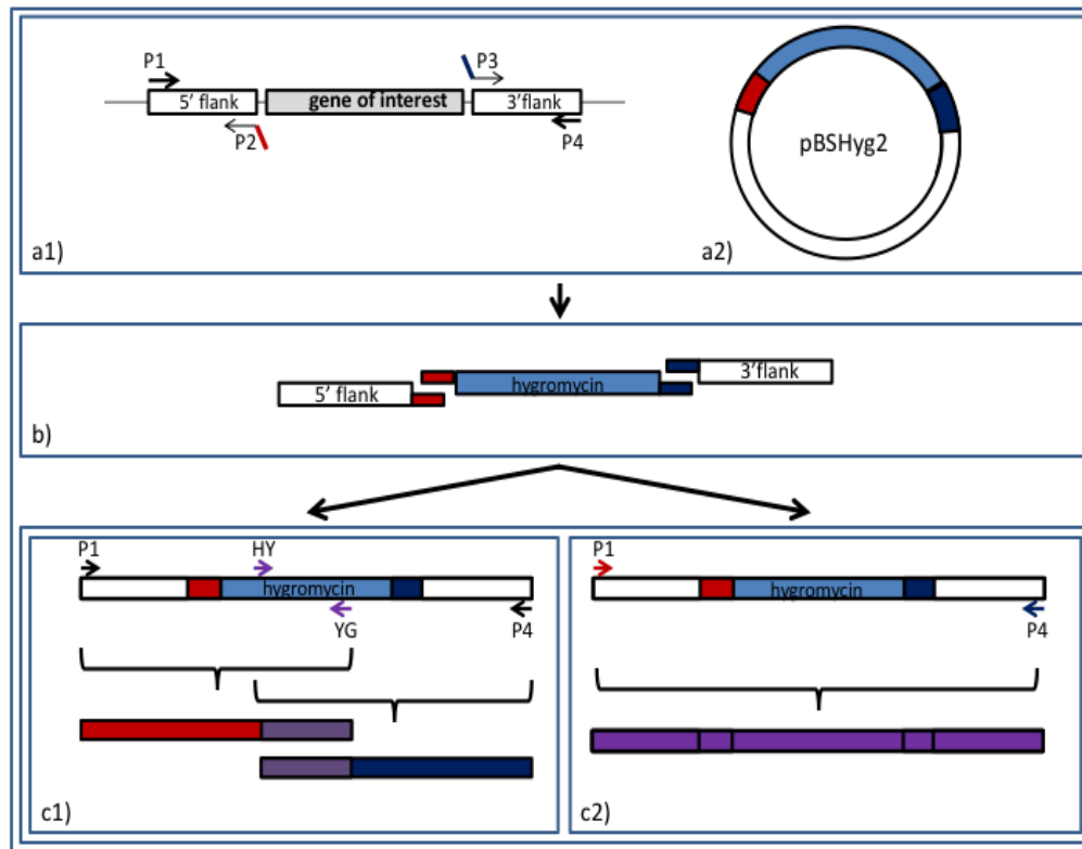
Figure 1. Split-marker and intact-marker gene-replacement strategies. a1) PCR amplification of flanking regions with overhangs containing RE recognition sequences; a2) release of hygromycin resistance gene from pBSHyg2 by digestion with EcoRI and BamHI ; b) Ligation of PCR-amplified flanking regions with the hygromycin gene released from pBSHyg2; c1) PCR amplification of split-marker fragments with combination of flanking region (5'flankP1 or 3'flankP4) primer and hygromycin-gene specific primer (HY or YG); c2) PCR amplification of an intact marker cassette with gene specific 5'flankP1 and 3'flankP4 primers.
