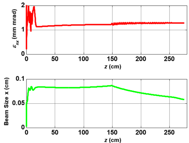
Figure 1: Beam size and emittance evolution along the electron source.
