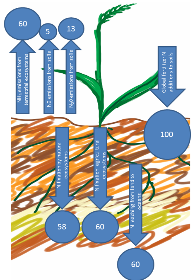
Figure 1. Global fluxes of N through soils ( \text{Tg N yr}^{-1} ). Based on data from Fowler et al. (2013).
