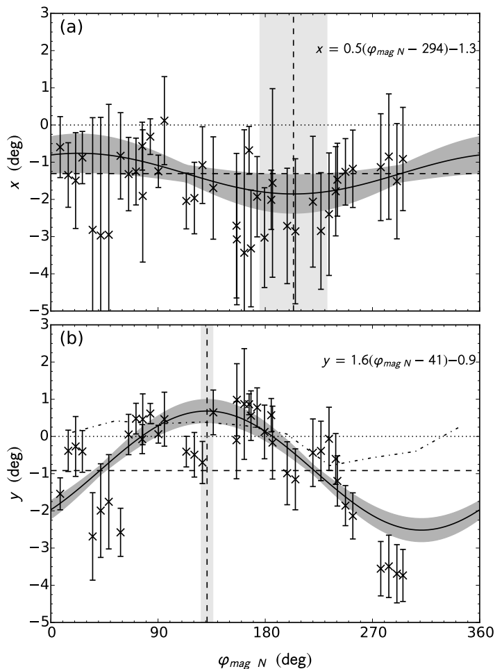
Figure 7: Figure showing the locations in degrees of co-latitude of the circles fitted to the northern auroras in the (a) x (positive sunward) and (b) y (positive duskward) directions versus PPO phase for northern PPO system \phi_{mag N} . The error bars indicate the uncertainty in the location of the circle fit. The best fit sinusoidal functions are shown by the solid lines, whose equations are shown in the top right of each panel. The associated dark grey shaded areas indicate the combined 1\text{-}\sigma range arising from the uncertainty in the amplitude and vertical offset of the best fit function parameters. The dashed vertical line indicates the location of maximum duskward displacement, while the associated vertical light grey region indicate the 1\text{-}\sigma uncertainty in phase offset \varphi_0 . In panel (b) the binned dawn-dusk location of the northern oval as determined by Nichols et al. (2010b) is shown by the dot-dashed line.
