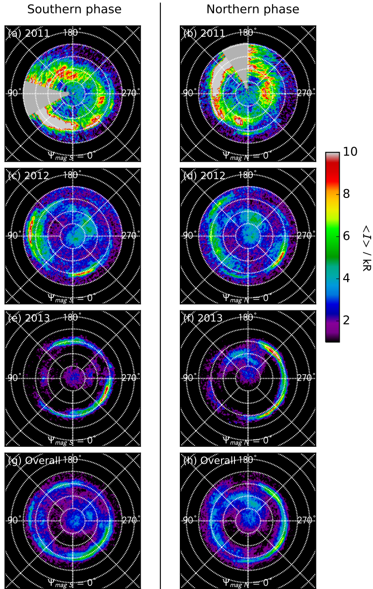
Figure 12: As for Fig. 11 but for the northern images. A data gap in the 2011 images in the top row is shown in grey.
