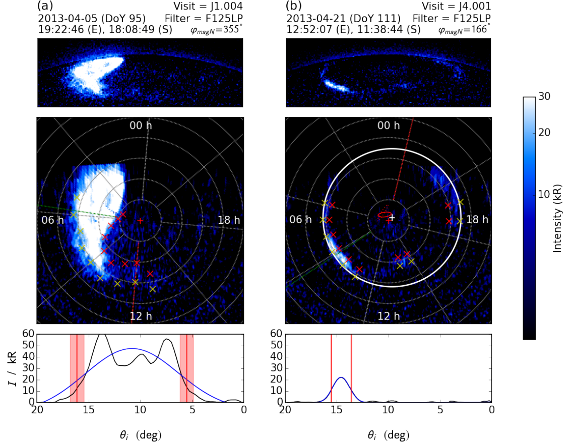
Figure 3: Figure showing two example images with the computed poleward and equatorward boundaries overplotted with the red and yellow crosses, respectively. The unprojected and projected images are shown, with the latter in the same format as Fig. 1. At the bottom of each panel, representative latitudinal intensity profiles along the meridians highlighted in green in the projections are shown. The Gaussian fits are shown in blue, and the 1- \sigma envelope of the FWHM locations are shown by the vertical red lines and shaded regions. The best fit ellipse for the oval motions observed in this program (solid line) and the 2008 program (dotted line) are shown in red, along with a red cross indicating the spin pole. In panel (b) the best fit circle is shown by the white circle, and its centre is shown by the white cross, with the length of the arms of the cross indicating the uncertainties in each direction as given by the fitting procedure.
