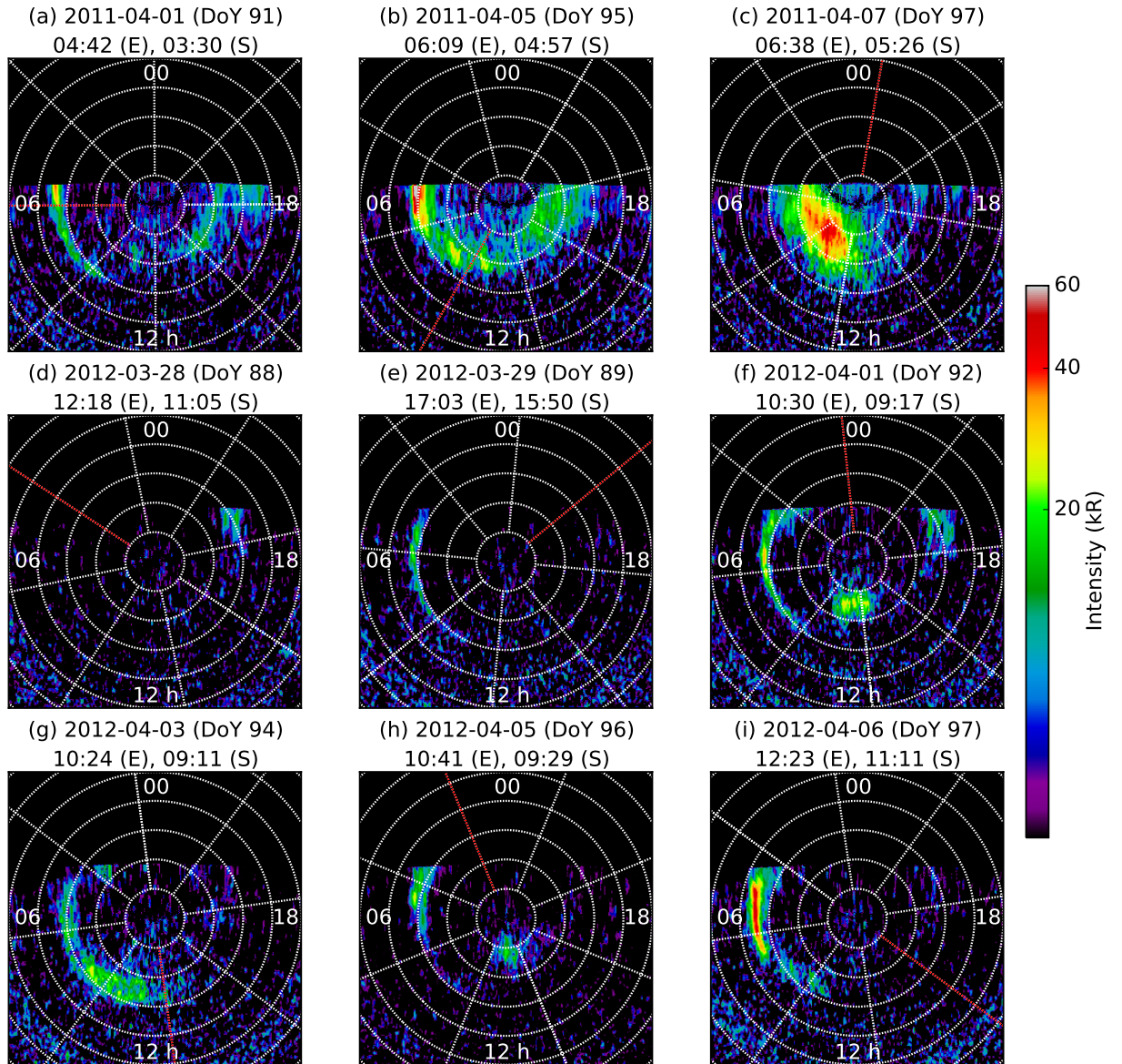
Figure 1: Figure showing representative images obtained during 2011 and 2012. Each image is labelled with the date and time of the exposure at Earth (E) and corrected for one-way light travel time from Saturn (S). Each image is shown on a Lambert Equal Area Azimuthal projection, with noon oriented to the bottom. A 5^\circ \times 45^\circ latitude-longitude grid is overlaid by the grey dotted lines, and the direction of \Psi_{mag S} = 0^\circ is shown by the red line. The intensities are shown on a log-scale, saturated at 30 kR.
