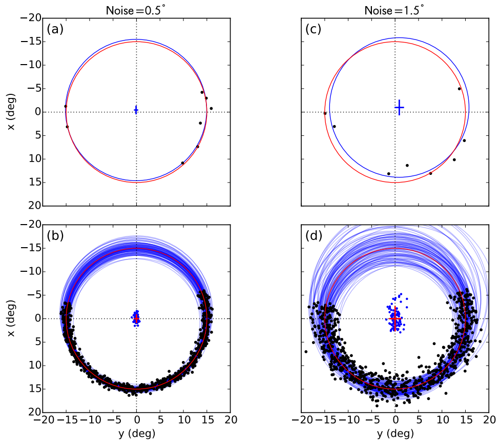
Figure 13: Circle fits (blue circles) to simulated data (black points) with (left) \sim 0.5^\circ and (right) \sim 1.5^\circ radial noise about a 15^\circ circle centred on the origin (red circle). In panels (a) and (c) the centre of the fitted circle is shown by the blue cross, with the length of the arms of the cross indicating the uncertainties in each direction. In panels (b) and (d) the centre of each fit is shown by a point, while the red crosses centred on the origin indicate the mean uncertainty values obtained in the fits.
