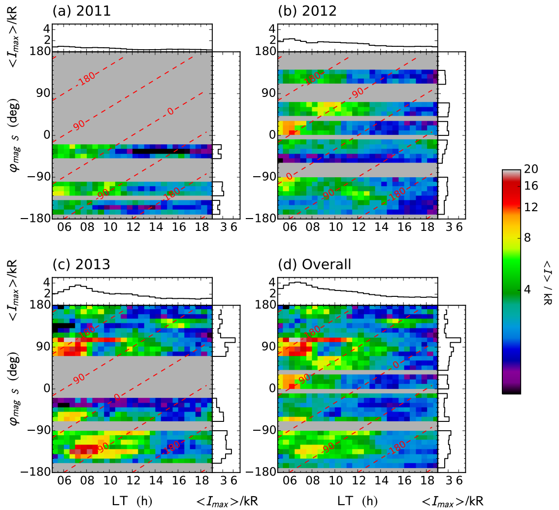
Figure 10: As for Fig. 9 but for the southern PPO phase.
