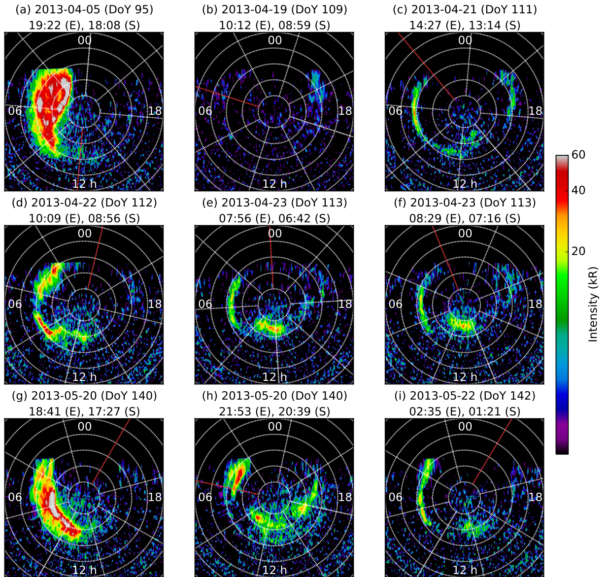
Figure 2: As for Fig. 1 but for images obtained in 2013.
