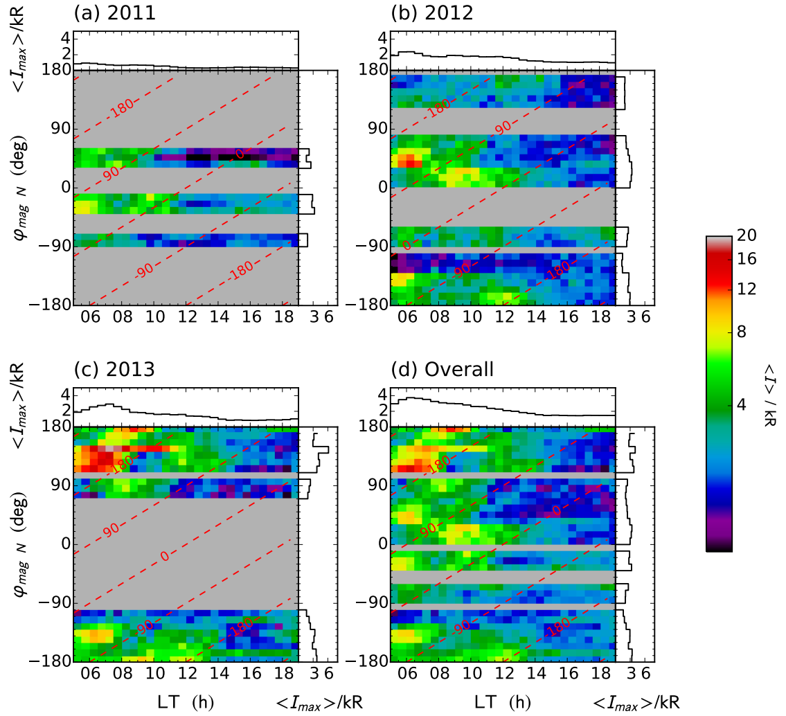
Figure 9: Figure showing the maximum intensities I_{max} in kR determined as discussed in the text for the northern auroras, in LT-northern PPO phase space for (a) 2011, (b) 2012, (c) 2013, and (d) overall. Lines of constant \Psi_{mag N} are shown by the red dashed lines, and data gaps are shown in grey. Means along each axis are also shown by the sub-panels to the top and right of each main panel.
