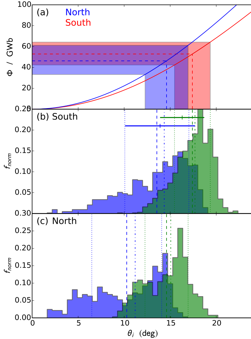
Figure 5: Figure showing normalised histograms of the equatorward (green) and poleward (blue) boundary co-latitudes for (panel b) the south and (c) the north. The distribution means (medians) are indicated by the dashed (dot-dashed) lines, and the 1- \sigma ranges about the means are shown by the dotted lines. In panel (b) the horizontal lines indicate the means and 1- \sigma range of the Badman et al. (2006) boundaries. In panel (a) we show the magnetic flux \Phi in GWb contained within co-latitude \theta_i for the south (red solid line) and the north (blue solid line). The similarly-coloured vertical dashed lines with shaded areas show the mean and 1- \sigma ranges of the equatorward boundaries, and the horizontal regions indicate the corresponding magnetic fluxes.
