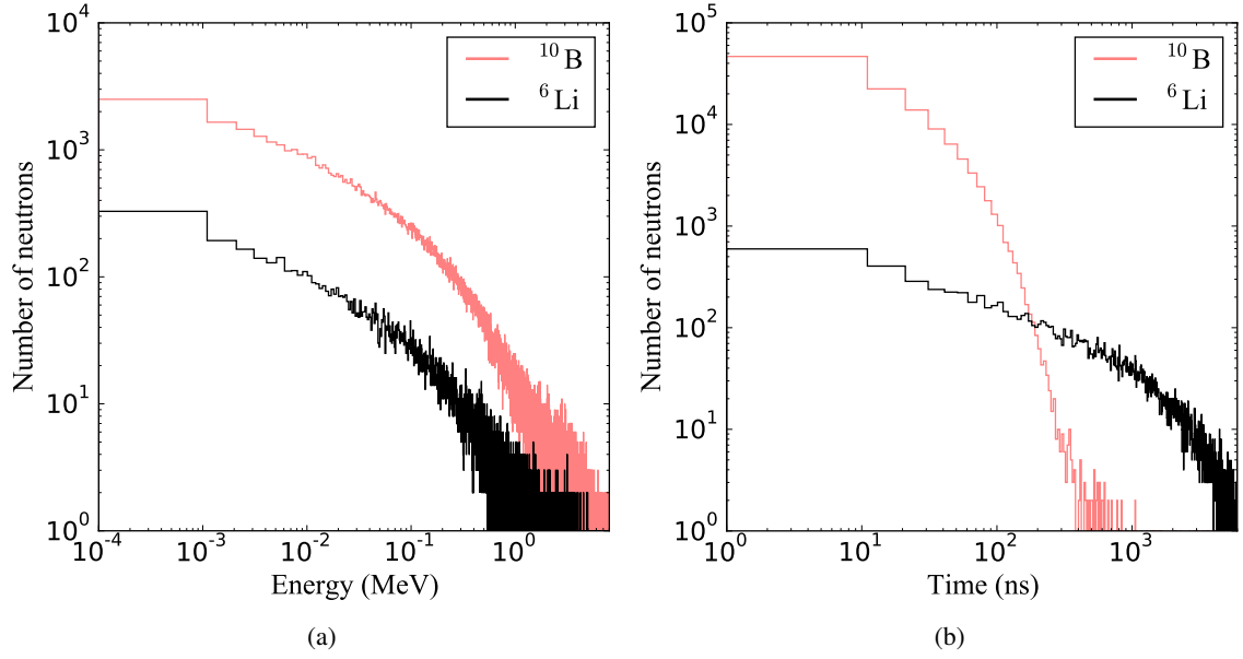
Figure 2. Simulated results of two different loading elements ( {}^6\text{Li} and {}^{10}\text{B} ) in a scintillator. The figures show (a) a histogram of neutron energy deposited in the scintillator from an event resulting in neutron capture (b) a histogram of time between fast neutron interaction and capture of this neutron for a number of events.
