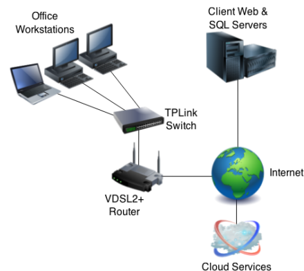
Figure 9: SME-3 Network
