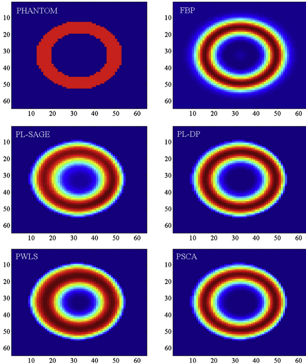
Fig. 44. Reconstructions of a simulated phantom using various techniques. The phantom is shown in the top-left image, with the reconstructions following, and labelled as per their reconstruction technique [Caruso et al. (2009)].
