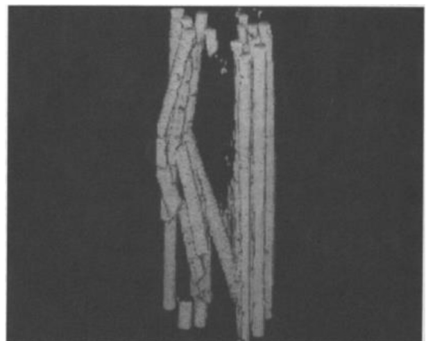
Fig. 36. A 3D FBP reconstruction of a failed LWR assembly from digitised radiographs [ Hansche (1989) ].
