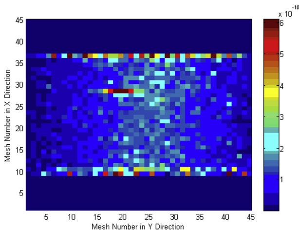
Fig. 10. A simulated result of a single UO_2 fuel pin lay on its side tomographed using muons and the MLEM reconstruction technique [Jonkmans et al. (2013)].
