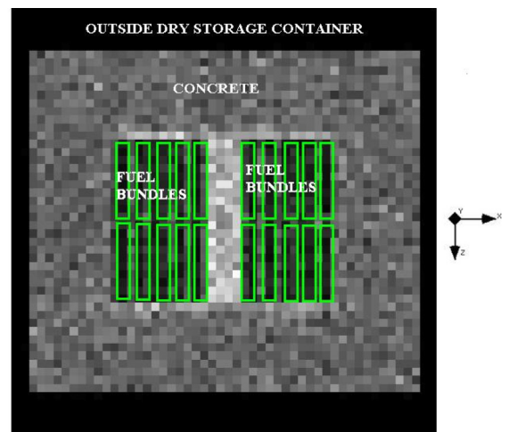
Fig. 12. The results of muon tomography on simulated fuel bundles within a Dry Storage Container (DSC) [Jonkmans et al. (2013)].
