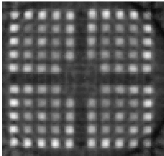
Fig. 4. A \gamma tomograph reconstructed from measured data, showing all rods in place in a spent fuel assembly [Lundqvist et al. (2007)].
