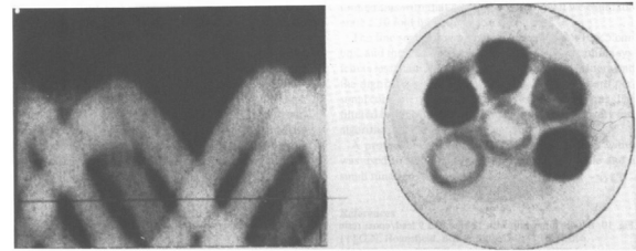
Fig. 7. Sinogram and tomogram showing a set of 6 phantom pins interrogated by a 0.025 eV neutron beam [Steinbock (1991)].
