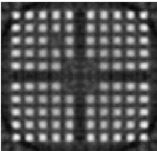
Fig. 3. A \gamma tomograph reconstructed from simulated data showing a missing rod from a spent fuel assembly (top left) [Lundqvist et al. (2007)].
