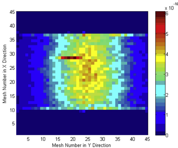
Fig. 11. A simulation of a single UO_2 fuel pin lay on its side tomographed using muons and the SDE reconstruction technique [Jonkmans et al. (2013)].
