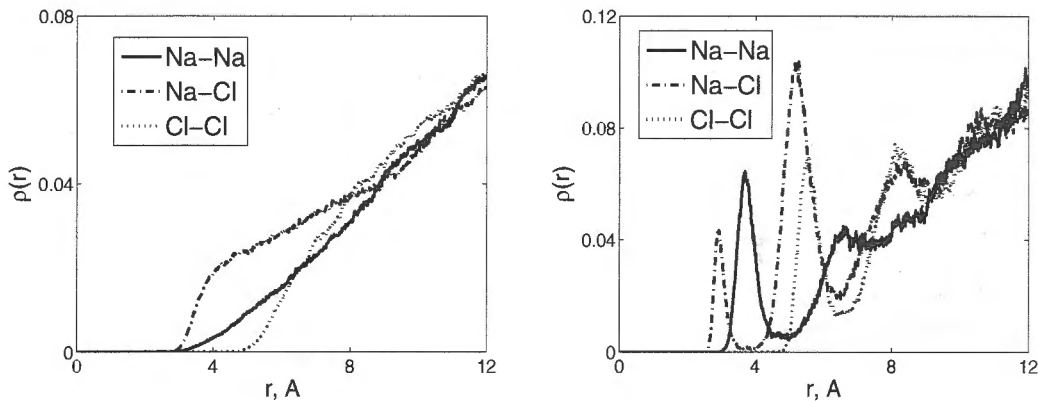
Figure 1. (left) number of ions as a function of the distance between ions of different type: C=400 mMol; Box size: 40 Å. Forces included into the simulations: (i) Coulomb interaction; (ii) short range repulsion. (Right) The number of ions as a function of the distance between ions of different type: C=400 mMol; Box size: 40 Å. Forces included into the simulations: (i) Coulomb interaction; (ii) short range repulsion; (iii) hydration.
