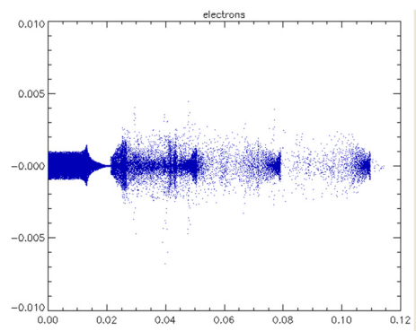
Figure 3: Electron horizontal offset plotted against longitudinal position in metres.
