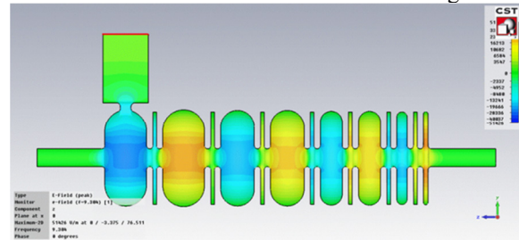
Figure 1: Compact Linac Cavity modelled in CST [4].
