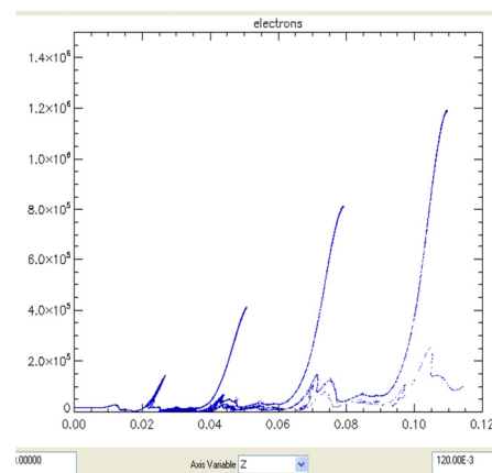
Figure 2: Electron energy, in eV, as a function of longitudinal position in the linac, in metres.
