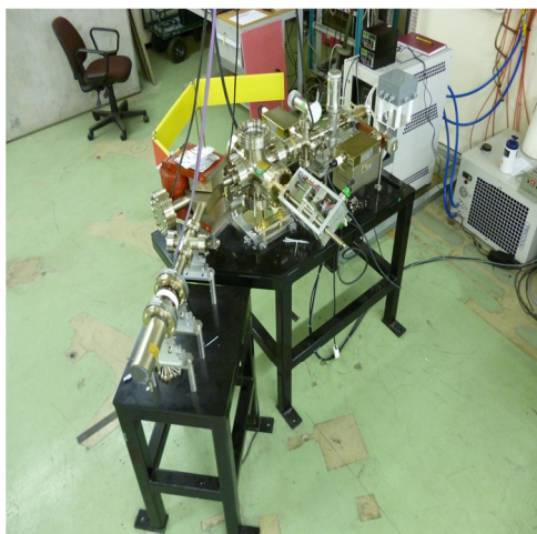
Figure 6: Compact linac Diagnostics Line.
