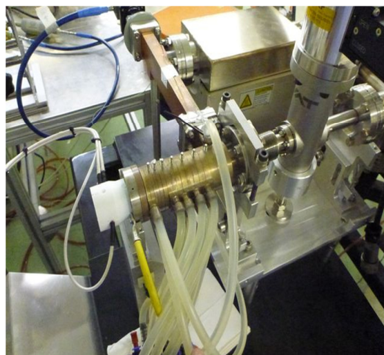
Figure 5: Compact linac cavity and gun installed.
