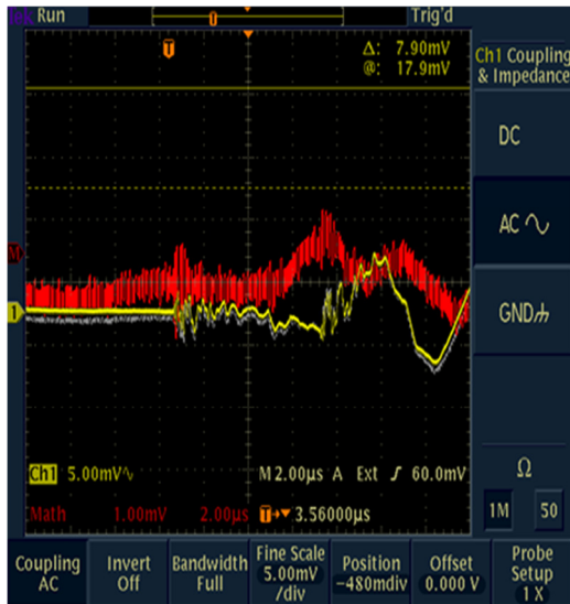
Figure 7: Faraday cup signal after the spectrometer magnet at 610 keV.
