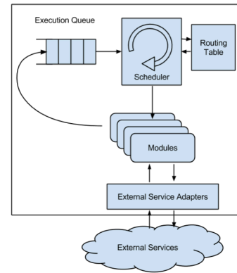
Figure 3. WoTKit Processor Architecture
