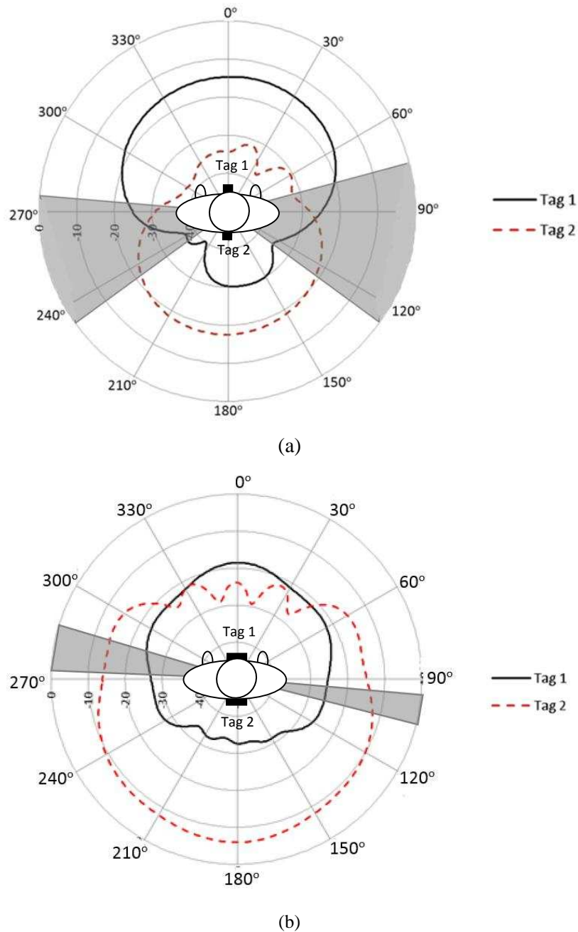
Fig. 6.25 Azimuth plots for (a) vertically oriented tags placed on the chest and back (b) horizontally oriented tags placed on the chest and back
