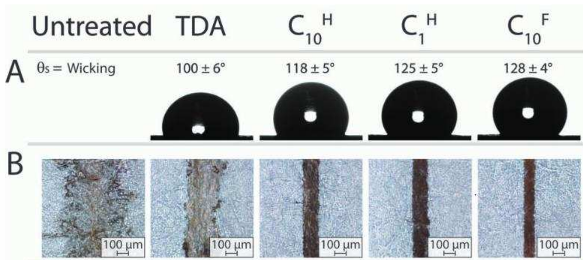
Fig. 5.2 Influence of surface energy on ink interaction (A) Images of 10- \mu L drops of water on a series of Canson tracing papers, modified with different organosilanes, and their corresponding static contact angles ( \theta_s ) (with standard deviation for n = 7 measurements). (TDA = Tris Dimethylamino Silane) (B) Optical micrographs of silver wires printed on the modified or unmodified Canson tracing paper substrates using the reactive silver ink with a target resolution of 80 \mu m [13].
