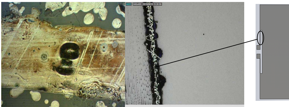
Fig. 5.7 Pinhole on feedline
