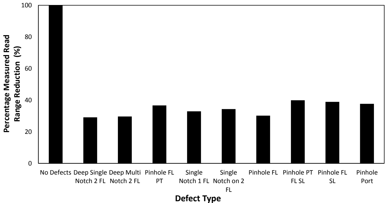
Fig. 5.18 Measured Tag Read Range as Percentage of Perfect Tag. FL = Feedline, PT = Port, SL = slot
