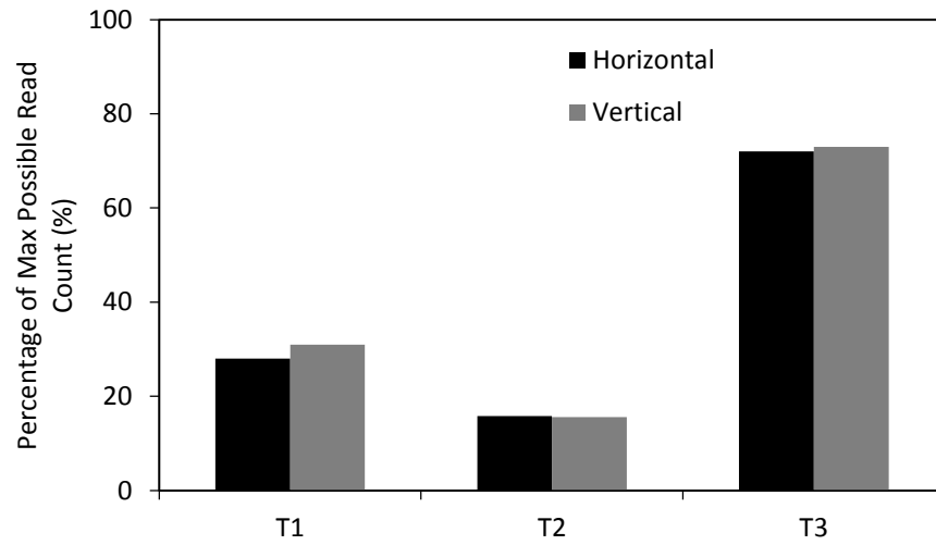
Fig. 6.45 Twisting motion with 3 tags on body
