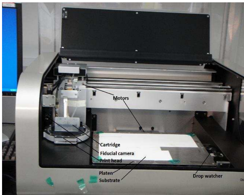
Fig. 3.10 Dimatix DMP-2831 Materials Printing System
