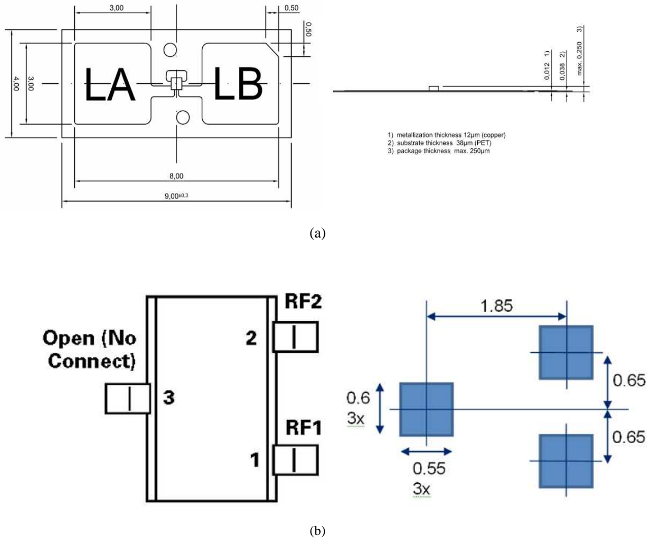
Fig. 3.8 Schematic of showing tag dimensions of (a) NXP G2X chip [11] and (b) Higgs-4 chip [12]. All dimensions in mm
