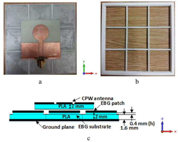
Fig. 2 Coplanar waveguide (CPW) fed on EBG structure: a) configuration, b) EBG stencil, c) side view with dimensions.
