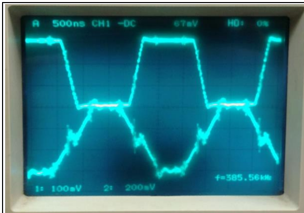
Fig. 6a Power switching waveform (top), and gate drive waveform (bottom trace).
