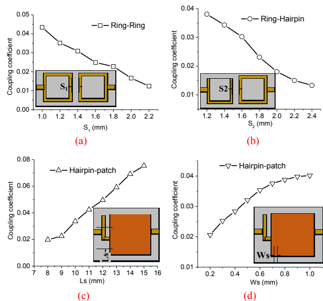
Fig. 6. Coupling coefficients between resonators: (a) two ring strip resonators with S_1 (b) ring strip resonator and hairpin resonator and the patch resonator with length of slot L_s and (d) hairpin resonator and the patch resonator with width of slot W_s .
