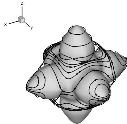
Fig. 2: Simulated flow structure of TEMHD around an equiaxed dendrite growing from an undercooled melt under an arbitrarily low static magnetic field (taken from ref. [11]).
