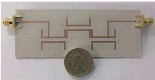
Figure 11. Fabricated microstrip dual-band filter.
