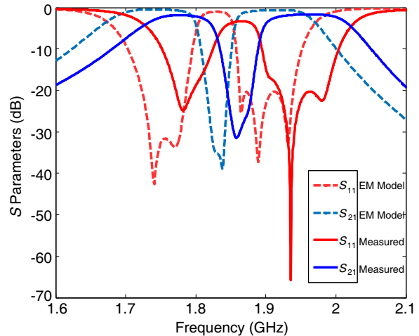
Figure 12. Simulated and measured responses.
