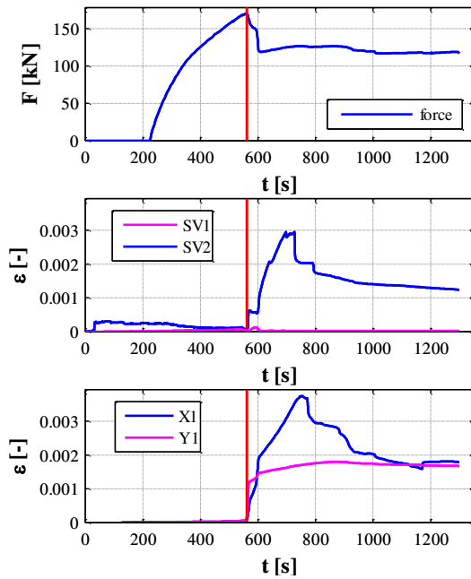
Figure 9. Instrumentations records. From the top: force of the actuator, deformations of the concrete and deformations of the upper stirrup in the column
