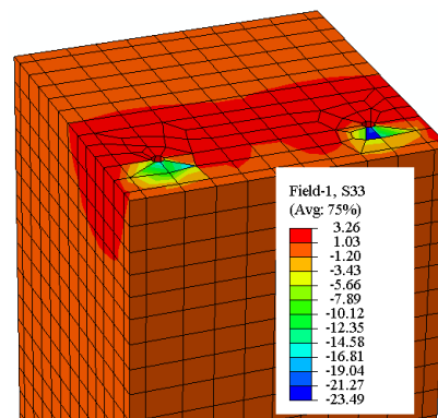
Figure 18. Column stress distribution at the failure step resulting from the numerical model
