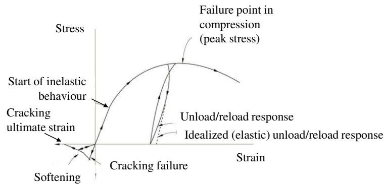
Figure 12. Mechanical behavior of the smeared crack concrete model (Systèmes, 2008)
