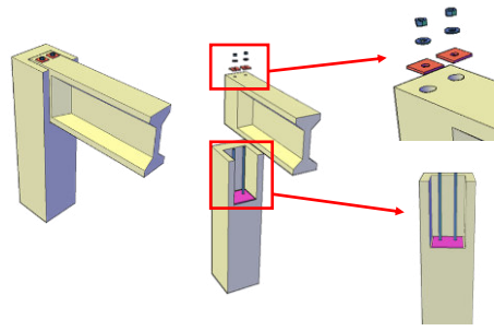
Figure 1. Beam-to-column dowel connection
