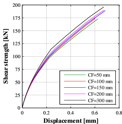
Figure 24. Shear force against the concrete core: force-displacement curves varying the frontal cover
