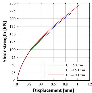
Figure 26. Shear force against the concrete core: force-displacement curves varying the lateral cover
