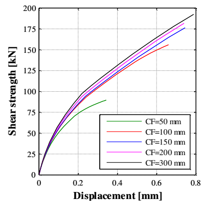
Figure 25. Shear force against the concrete cover: force-displacement curves varying the frontal cover
