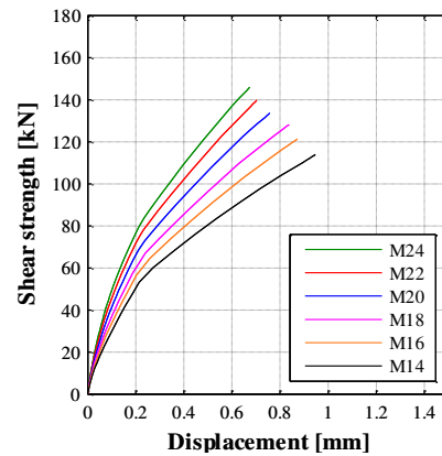
Figure 23. Shear force against the concrete cover: force-displacement curves varying the dowels diameter
