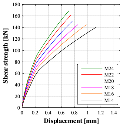
Figure 22. Shear force against the concrete core: force-displacement curves varying the dowels diameter
