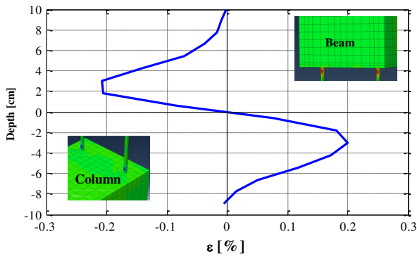
Figure 20. Deformation of the dowel at the failure step versus the beam and column depth
