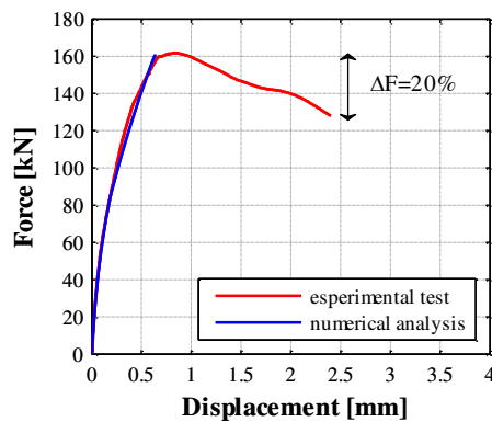
Figure 17. Comparison numerical analysis (blue line) vs experimental test (red line) in terms of force-displacement curve
