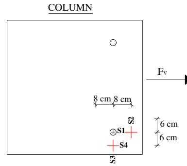
Figure 19. Layout of the strain gauges on the column top surface
