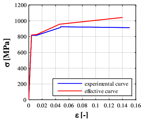
Figure 13. Stress-strain relationships for steel dowel: experimental curve (blue curve) and effective curve (red curve)
