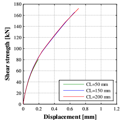
Figure 27. Shear force against the concrete cover: force-displacement curves varying the lateral cover
