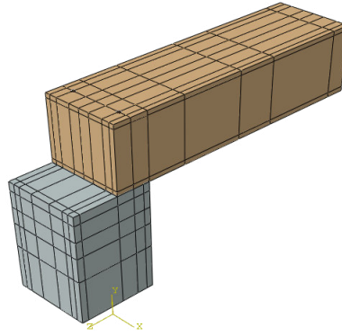
Figure 11. FEM model of the dowel connection by ABAQUS (Corp., 2010)
