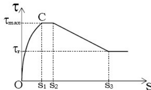
Figure 16. Bond-stresses versus slip for the deformed bar – confined concrete contact behavior according to the Eligehausen model (Eligehausen et al., 1986)
