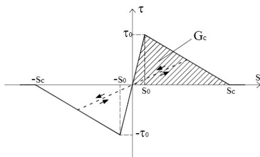
Figure 15. Adopted analytical model for cohesive interface elements
