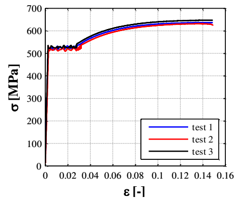
Figure 14. Experimental stress-strain relationships for steel reinforcement ( \phi=8\text{mm} )
