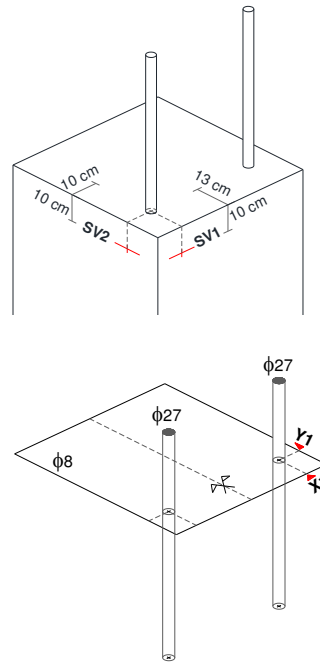
Figure 10. Geometrical layout of the column instrumentations
