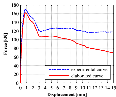
Figure 5. Force-displacement curve of the monotonic test (dashed blue line) and “elaborated” curve (solid red line)
