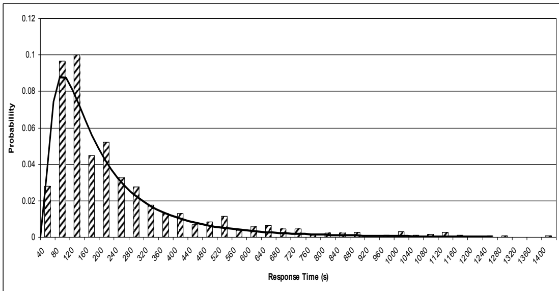
Fig.3. Overall log normal response time distribution for the CS assembly trial
