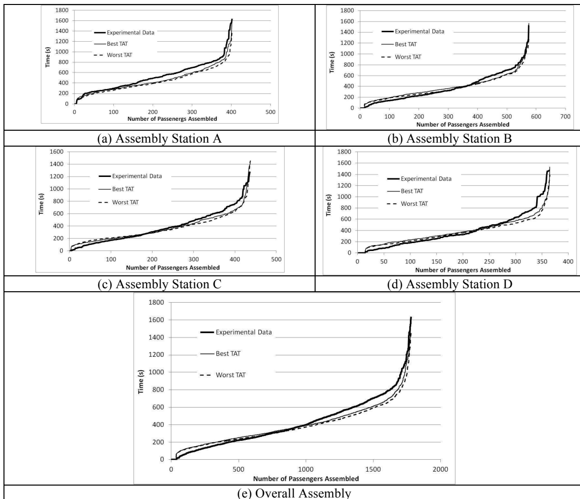
Fig.4. Comparison of model predictions with experimental data for CS
