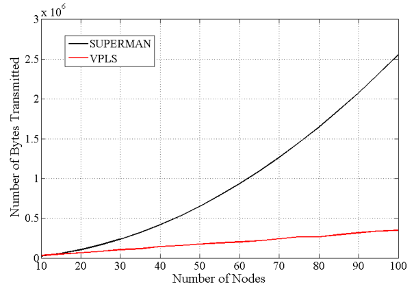
Fig. 4 Graph showing the number of bytes transmitted when authenticating all nodes with the network
