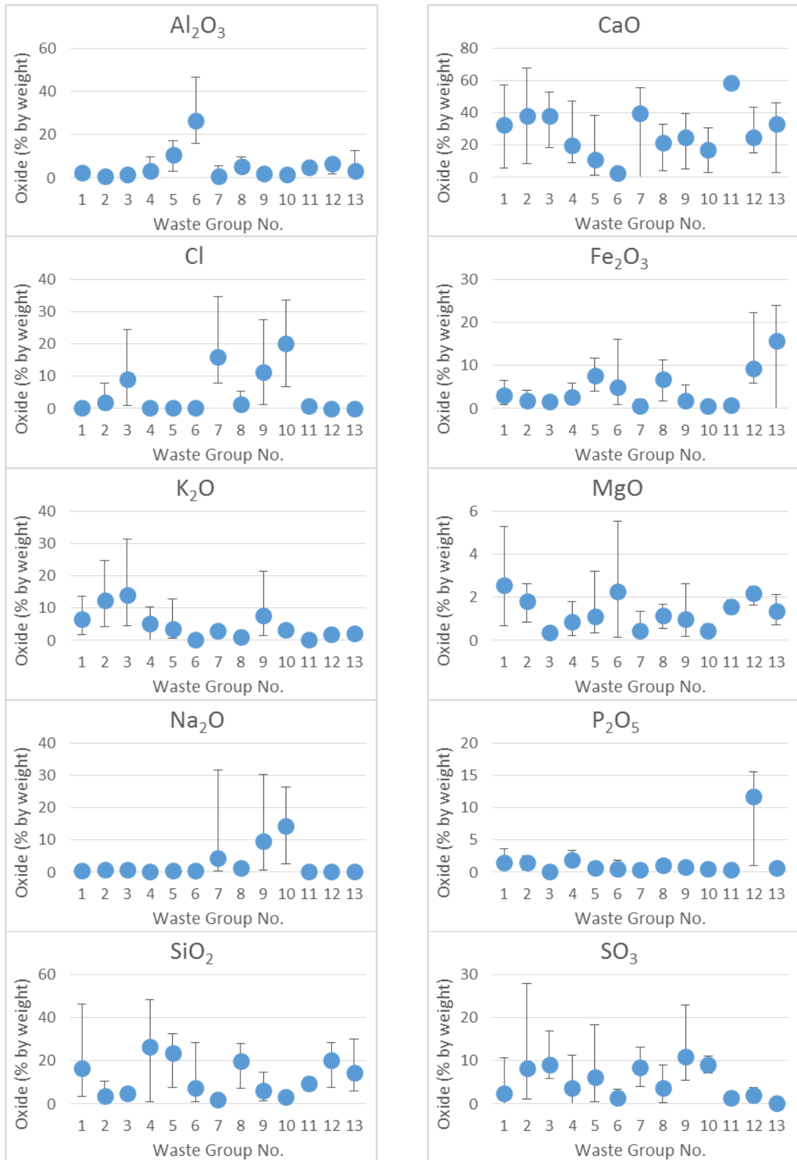
Figure 1: Bulk chemistry of waste groups (error bars denote minimum and maximum values in the group)
