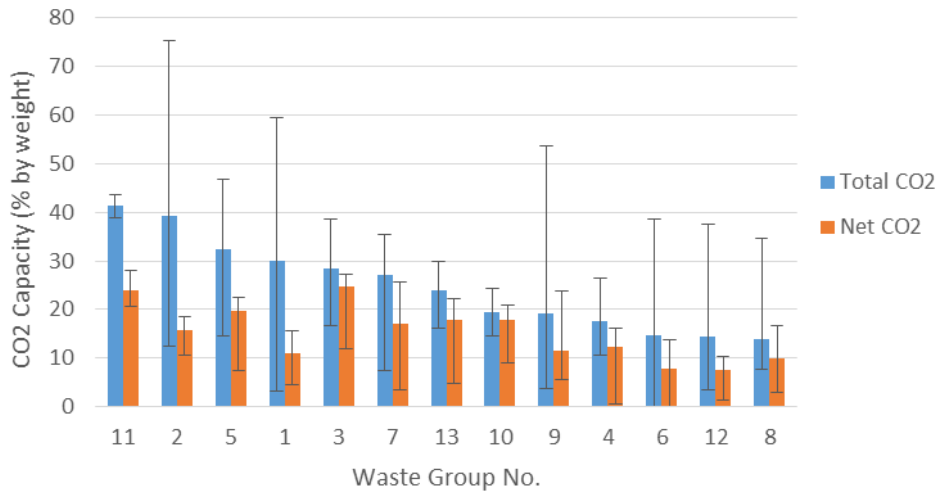
Figure 2: Carbon dioxide capacity of wastes (whiskers illustrate minimum and maximum values)
