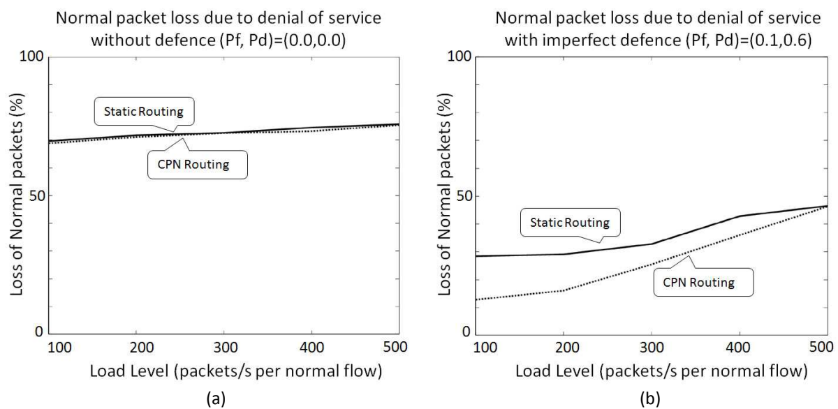
Figure 9 Packet loss during a DoS attack for static and CPN dynamic routing, (a) without DoS defence and (b) with an imperfect defence system
