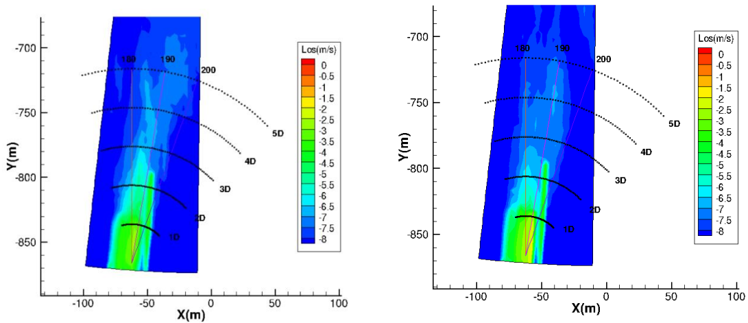
Fig. 2 Ten-minute averaged line of sight (Los) velocity, measured on 07-07-2014, 14:20 – 14:30 (left), 14:30 – 14:40 (right).
