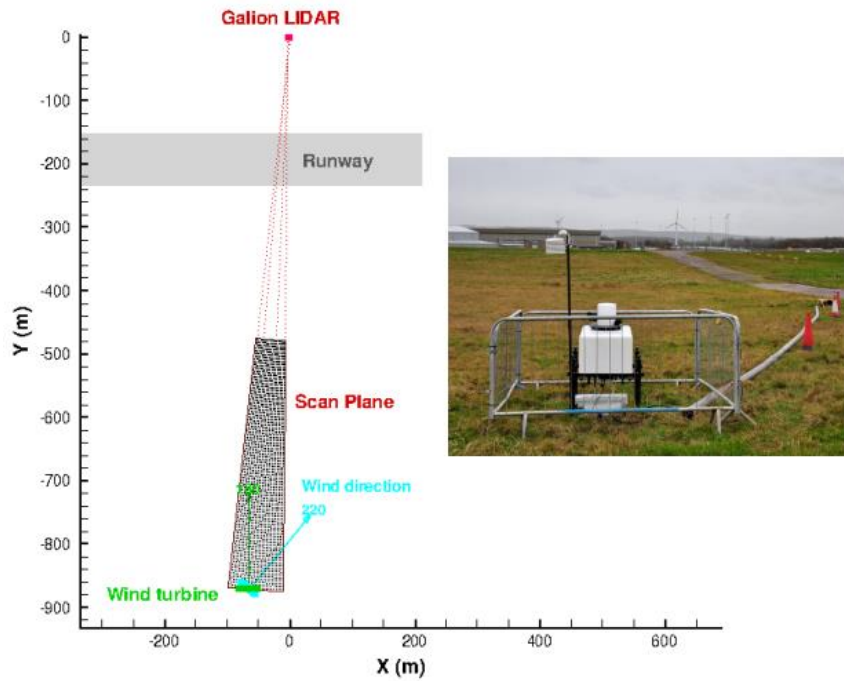
Fig. 1 Schematic of the LIDAR scan plane of wind turbine wake measurements. On-site Galion LIDAR is shown by the insert picture.
