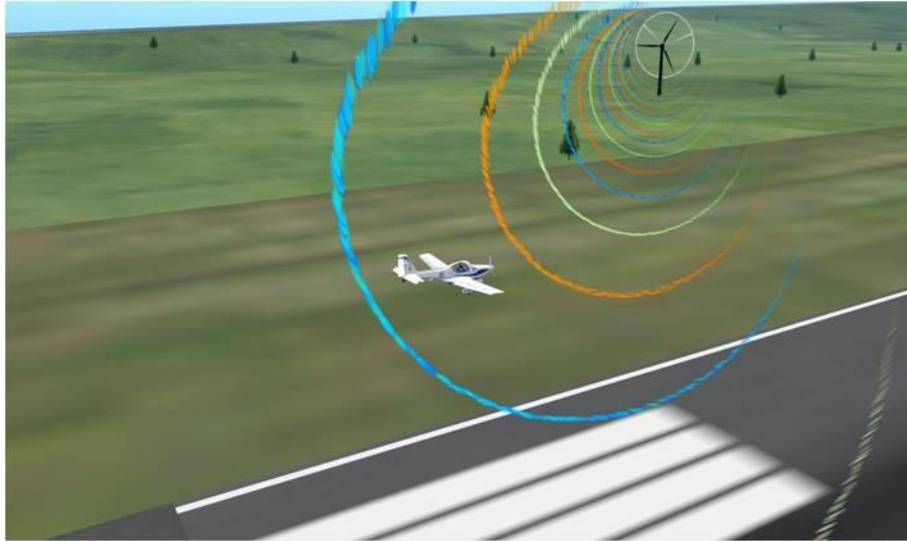
Fig. 3 Simulation scene of a light aircraft encountering wind turbine wakes.
