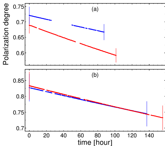
FIG. 4: Time dependence of the target polarization for the running periods in 2010 (a) and 2011 (b). The red (blue) points correspond to a polarization vector oriented upwards (downwards) in the laboratory system. The error bars at the beginning and end of each period indicate direct NMR measurements. The polarization degree for each run was obtained from the exponential relaxation.
