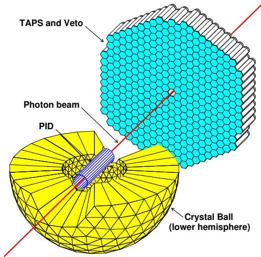
FIG. 3: Detector setup consisting of the Crystal Ball and TAPS calorimeters. The upper hemisphere of the Crystal Ball is omitted to show the barrel of plastic scintillators surrounding the target (PID).
