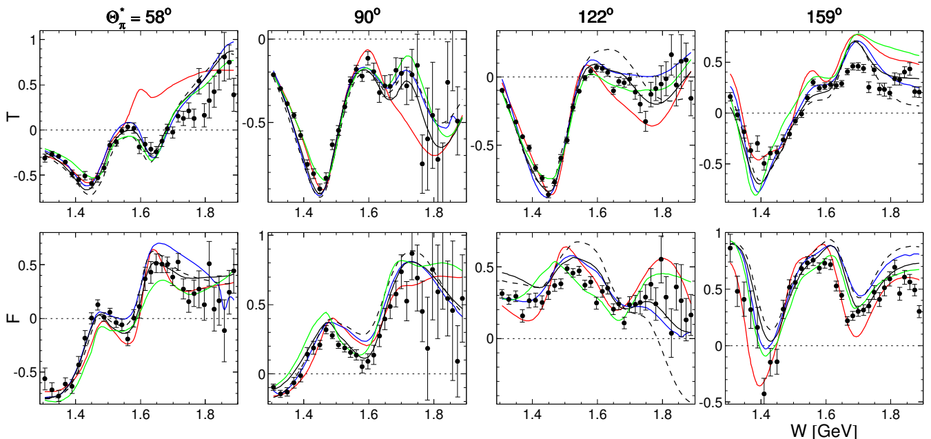
FIG. 8: (Color online) Dependence of the asymmetries T and F on the center-of-momentum energy W for selected angular bins. The experimental data (filled circles) are compared to theoretical predictions of MAID 2007 (red) [21], SAID PR15 (blue) [2, 22], BG2014-2 (black solid) [23], BG2011-2 (black dashed) [24], and JuBo2015-B (green) [25]. Only statistical uncertainties are given for all data points.
