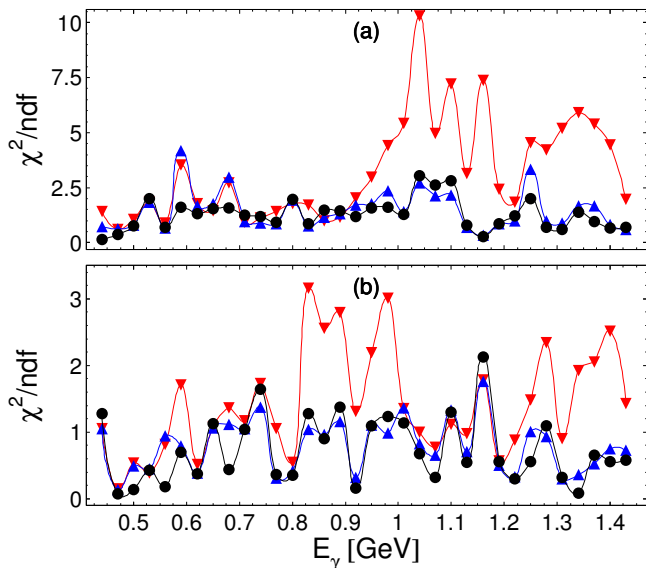
FIG. 10: (Color online) Energy dependence of the reduced \chi^2 values for Legendre fits of the present polarization observables T (a) and F (b) with N=4 (red triangles down), 6 (blue triangles up), and 8 (black circles).
