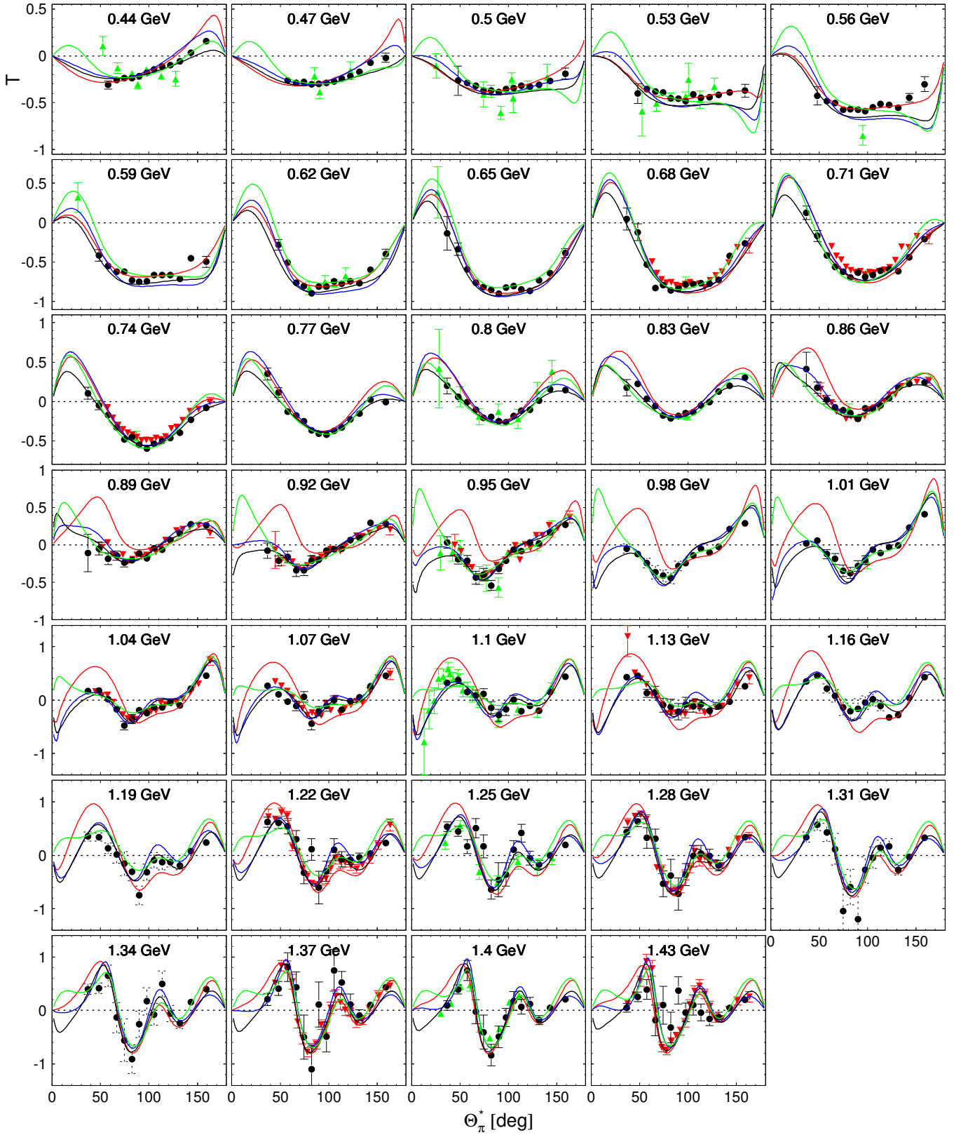
FIG. 6: (Color online) Target asymmetry T . Our experimental data shown by the filled circles are compared with older data (green triangles) from [20] as well to the latest CBELSA/TAPS data [4] (red triangles). Theoretical predictions of MAID 2007 [21], SAID PR15 [2, 22], BG2014-2 [23], and JuBo2015-B [25] models are shown by the red, blue, black, and green lines, respectively. The energy label in each panel indicates the central photon energy for each energy bin. Only statistical uncertainties are given for all data points.
