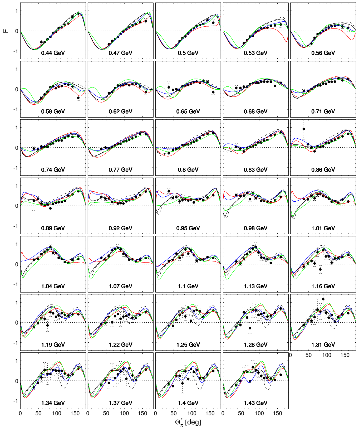
FIG. 7: (Color online) Beam target asymmetry F . Notations as in Fig. 6. The dashed curve shows the prediction of the BG2011-2 analysis.
