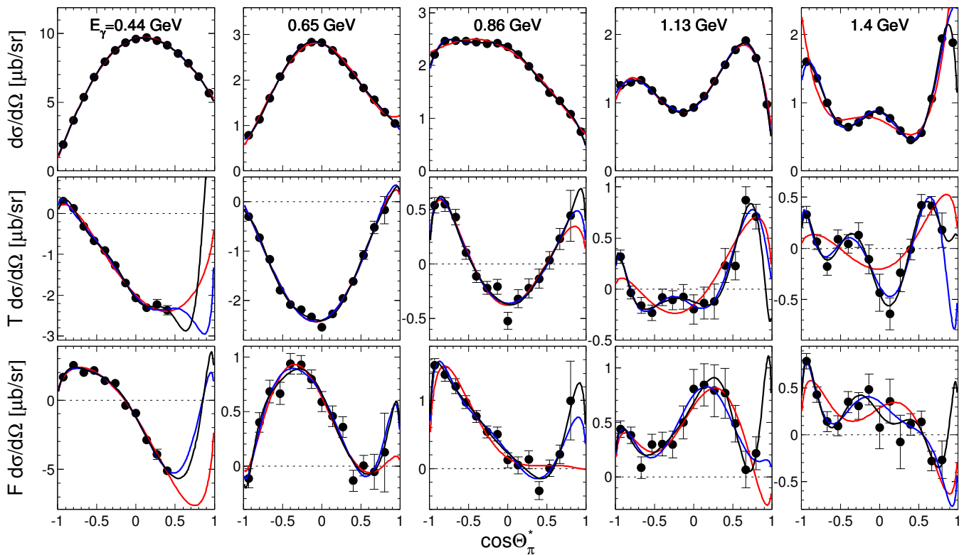
FIG. 9: (Color online) Unpolarized and polarized differential cross sections of the \gamma p \rightarrow \pi^0 p reaction for selected energy bins. Black circles are experimental data. Only statistical uncertainties are indicated. Legendre fit results for the polarized differential cross sections are shown by red ( N=4 ), blue ( N=6 ), and black ( N=8 ) lines.
