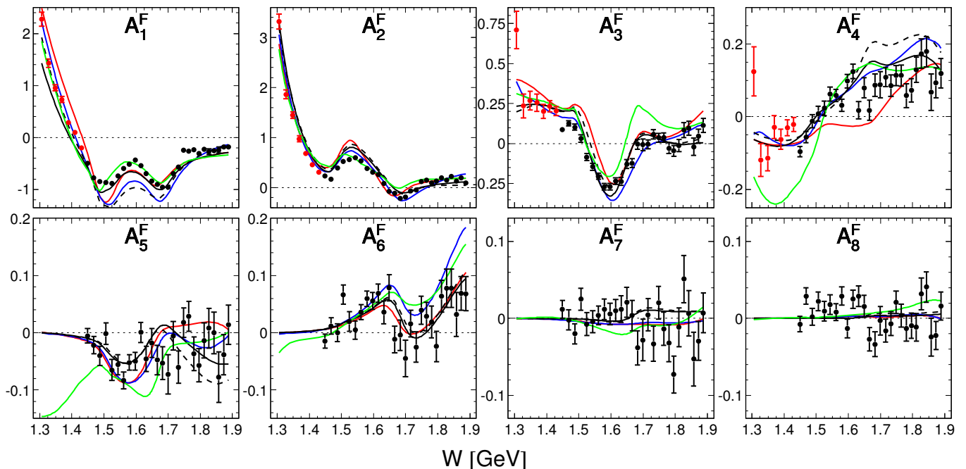
FIG. 12: (Color online) Same as Fig. 11 for Fd\sigma/d\Omega . The dashed curve shows the prediction of the BG2011-2 analysis.
