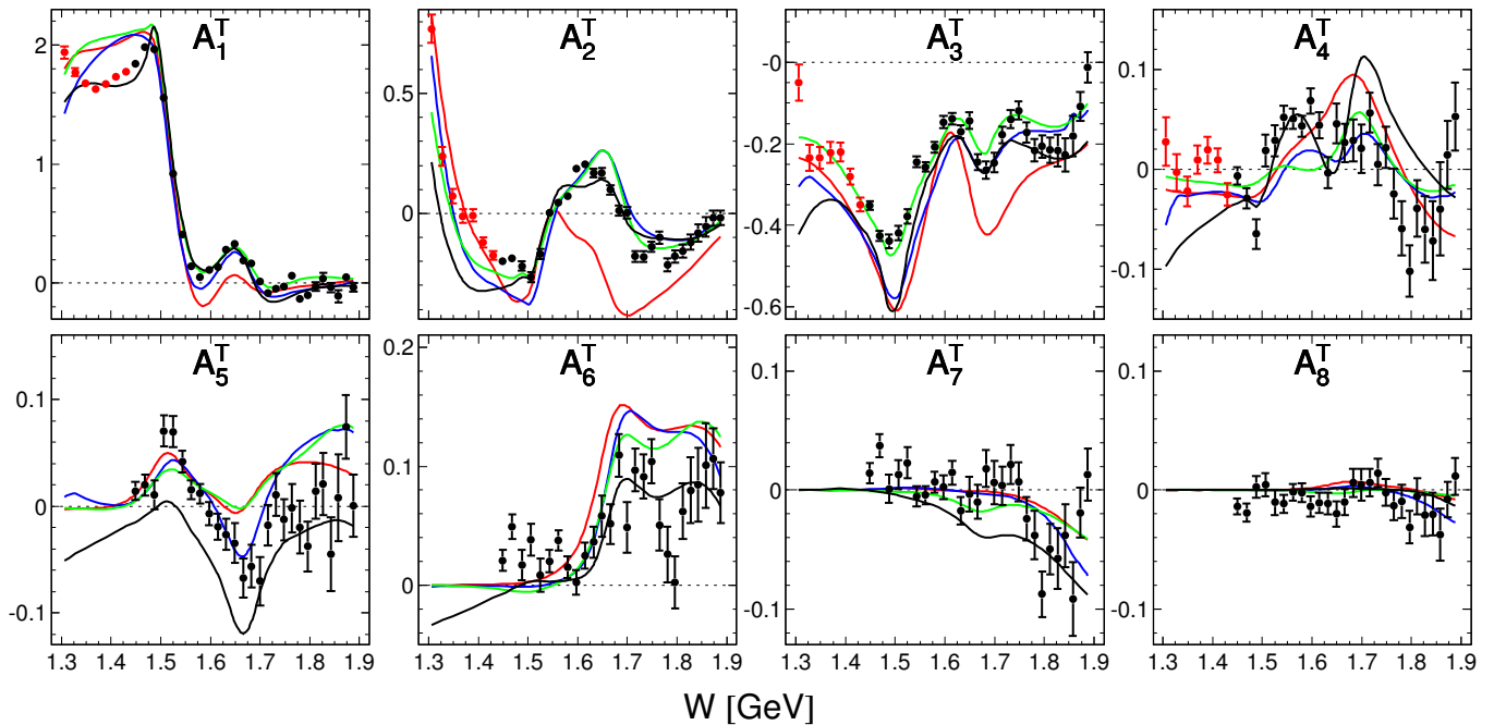
FIG. 11: (Color online) The coefficients A_n^T in the expansion (5) in units [\mu\text{b}/\text{sr}] obtained from the 8th-order (black circles) and 4th-order (red circles) least-square fit of Td\sigma/d\Omega as functions of the total center-of-momentum energy W . Notations for model predictions are the same as in Fig. 6.
