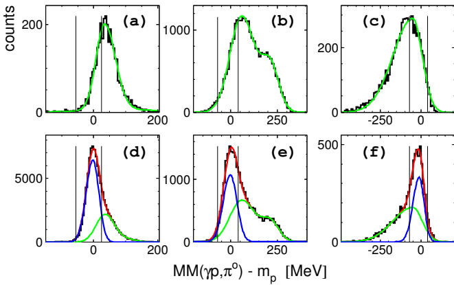
FIG. 5: (Color online) Distributions of the missing mass, MM(\gamma p, \pi^0) - M_p obtained with Carbon ((a)-(c)) and Butanol ((d)-(f)) targets at E_\gamma = 440 MeV, \Theta = 65^\circ ((a),(d)) and E_\gamma = 680 MeV, \Theta = 65^\circ ((b),(e)), \Theta = 160^\circ ((c),(f)). The Butanol distributions can be fitted by a normalized sum of Carbon (green line) and pure Hydrogen (blue line). The vertical solid lines indicate the selection of \gamma p \rightarrow \pi^0 p reactions used in the analysis.
