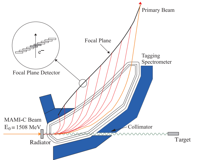
FIG. 1: The Glasgow-Mainz photon tagging spectrometer.
