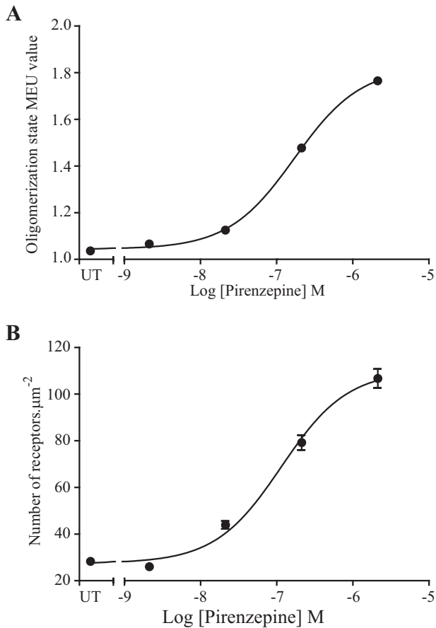
FIGURE 5. Pirenzepine-induced increases in both receptor oligomerization and expression levels are concentration-dependent. Experiments akin to those of Fig. 4 were performed on Flp-In T-REx 293 cells harboring hM 1 -mEGFP that had been treated with doxycycline (100 ng·ml -1 ) for 24 h and then treated with the indicated concentrations of pirenzepine. QB values corresponding to hM 1 -mEGFP were plotted as monomeric equivalent units against pirenzepine concentration (A) as were the number of receptor molecules· \mu\text{m}^{-2} (B). Data are presented as median (A) and mean (B). Error bars represent \pm S.E.; n = 84 in each case. UT, untreated.
