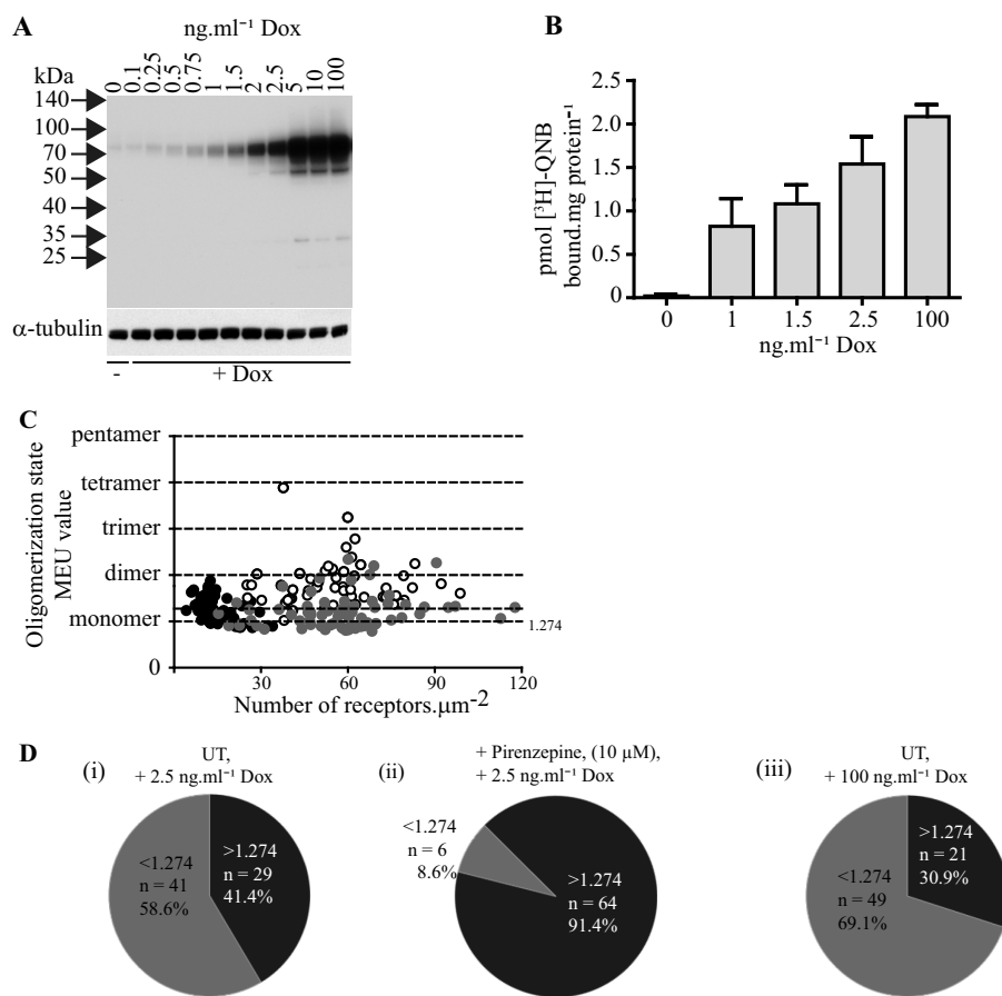
FIGURE 6. Pirenzepine stabilizes hM 1 -mEGFP dimers/oligomers independently from effects on receptor expression levels. Flp-In T-Rex 293 cells harboring hM 1 -mEGFP were treated with varying concentrations of doxycycline ( Dox ). A , lysates from these cells were immunoblotted with an anti-GFP antiserum to assess relative expression levels of the receptor construct. \alpha -Tubulin acted as a loading control. B , specific binding of a single near receptor saturating concentration of [ 3 H]QNB (5 nM) was assessed in cell membrane preparations generated from cells treated with the indicated concentrations of doxycycline. Shown are combined data from n = 3 experiments; error bars represent \pm S.E. C , comparisons of QB (presented as monomeric equivalent units) and receptor expression levels in cells induced to express hM 1 -mEGFP by treatment with 2.5 ng·ml -1 doxycycline ( black symbols ), treatment with 100 ng·ml -1 doxycycline ( gray symbols ), and after induction with 2.5 ng·ml -1 and pirenzepine treatment ( open symbols ). D , in this data set, 91% of the RoIs contained a majority of ligand treatment. UT , untreated.
