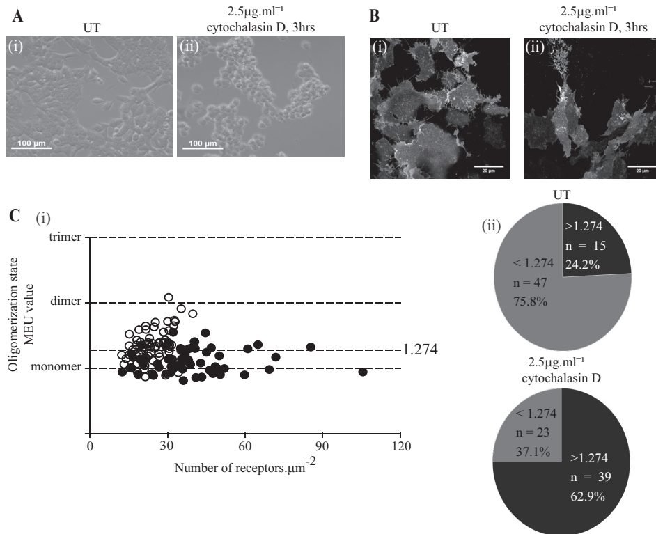
FIGURE 9. Actin cytoskeleton destabilization promotes M 1 receptor oligomerization. Flp-In T-Rex 293 cells harboring hM 1 -mEGFP were treated with doxycycline (100 ng·ml -1 ) for 24 h. A , bright field images of cells treated with vehicle (UT) ( panel i ) or with cytochalasin D ( panel ii ). B , images of the basolateral surface of cells treated with vehicle (UT) ( panel i ) or cytochalasin D ( panel ii ). C , comparisons of QB (presented as monomeric equivalent units) and receptor expression levels in cells treated with the vehicle ( panel i , filled symbols) or with cytochalasin D ( panel i , open symbols) for 3 h. Treatment with cytochalasin D produced a substantial increase in the proportion of RoIs containing a high percentage of receptor dimers/oligomers ( panel ii ).
