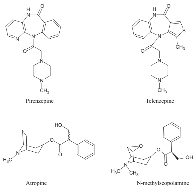
FIGURE 1. Structures of muscarinic antagonists. The chemical structures of pirenzepine, telenzepine, atropine, and N -methylscopolamine are shown.
