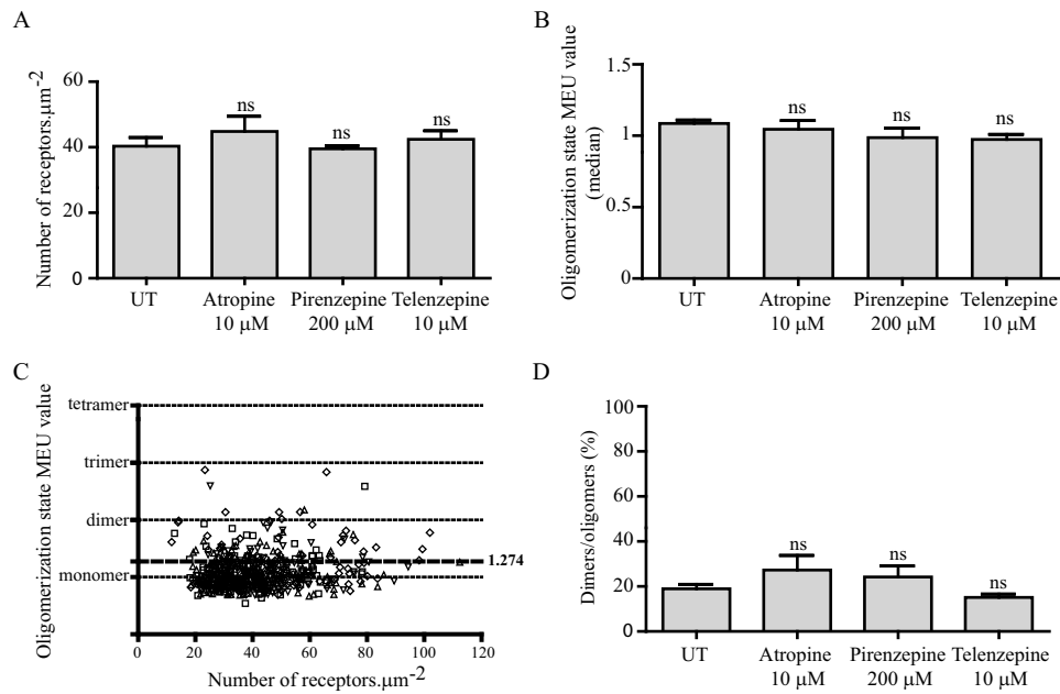
FIGURE 11. Muscarinic antagonists do not affect the quaternary organization of the M_3 receptor. Cells, as in Fig. 9, that had been induced to express hM 3 -mEGFP were treated with the indicated concentrations of atropine, pirenzepine, or telenzepine for 16 h. Imaging of Rol within the basolateral surface indicated that treatment with the ligands did not alter the mean receptor expression level (A) or the overall organizational state of the receptor (B). Data are presented as monomeric equivalent units. C, full data set of individual QB values (again expressed as monomeric equivalent units) for untreated cells (squares) and those treated with atropine (diamonds), pirenzepine (triangles), or telenzepine (inverted triangles). D, assessment of percentage of Rol containing predominantly dimers/oligomers following each treatment. ns, not significantly different from untreated. All graphs show combined data from at least n = 3 experiments; error bars represent \pm S.E. UT, untreated.
