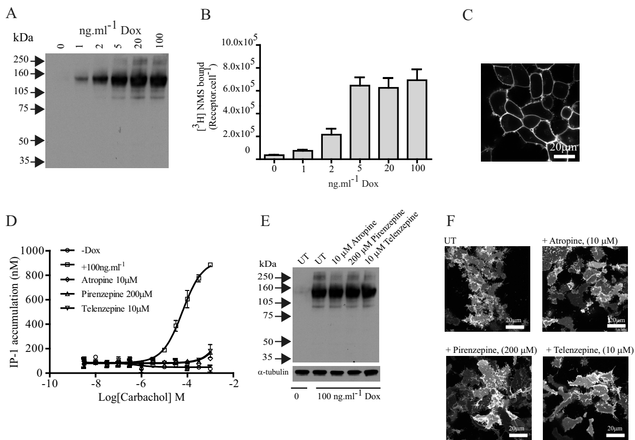
FIGURE 10. Muscarinic antagonists do not up-regulate levels of the M_3 receptor. Flp-In T-Rex 293 cells harboring hM_3 -mEGFP were treated with the indicated concentrations of doxycycline (Dox) for 24 h to induce expression of the receptor construct. A , anti-GFP immunoblotting of cell lysates detected hM_3 -mEGFP as a 140-kDa polypeptide. B , specific binding of [ ^3 H]NMS confirmed that the level of expression of hM_3 -mEGFP at the surface of intact cells is dependent on doxycycline concentration. Shown are combined data from n = 3 experiments; error bars represent \pm S.E. C , confocal image of cells induced to express hM_3 -mEGFP shows it to be restricted to the plasma membrane. D , the ability of the muscarinic agonist carbachol to promote generation of inositol monophosphates in these cells is dependent upon treatment with doxycycline (compare -Dox and 100 ng\cdot ml^{-1} ) and is fully blocked by the indicated concentrations of each of atropine, pirenzepine, and telenzepine. Shown are representative plots from n = 3 ; error bars represent \pm S.E. E and F , sustained treatment with atropine, pirenzepine, or telenzepine does not up-regulate levels of hM_3 -mEGFP. E , anti-GFP immunoblotting was performed on SDS-PAGE-resolved lysates from cells not induced with doxycycline or induced to express hM_3 -mEGFP and then treated for 16 h with the indicated concentration of atropine, pirenzepine, or telenzepine. Detection of \alpha -tubulin acted as a loading control. F , images of the basolateral surface of such cells. Scale bar, 20\ \mu m . UT, untreated.
