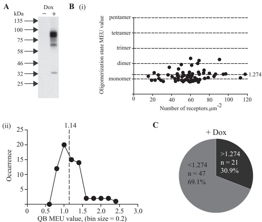
FIGURE 3. hM 1 -mEGFP exists as a mixture of monomers and oligomers in the basal state. Flp-In T-Rex 293 cells harboring hM 1 -mEGFP were maintained in the absence of doxycycline (– Dox ) or treated with doxycycline (100 ng·ml –1 ) for 24 h (+ Dox ). Lysates of these cells were resolved by SDS-PAGE and immunoblotted with an anti-GFP antiserum (A). B, panel i, shows QB detected in individual RoIs (presented as monomeric equivalent units) plotted against number of hM 1 -mEGFP·μm –2 of the basolateral surface (55.7 ± 2.3 μm –2 , mean ± S.E., n = 68). B, panel ii, QB values from individual RoIs were binned (bin size, 0.2 MEU). These displayed a non-symmetrical distribution skewed to values >1.00 MEU. Dotted line, median value. C, in this data set, 47 of the 68 measurements were assessed as being predominantly monomeric (69.1%).
