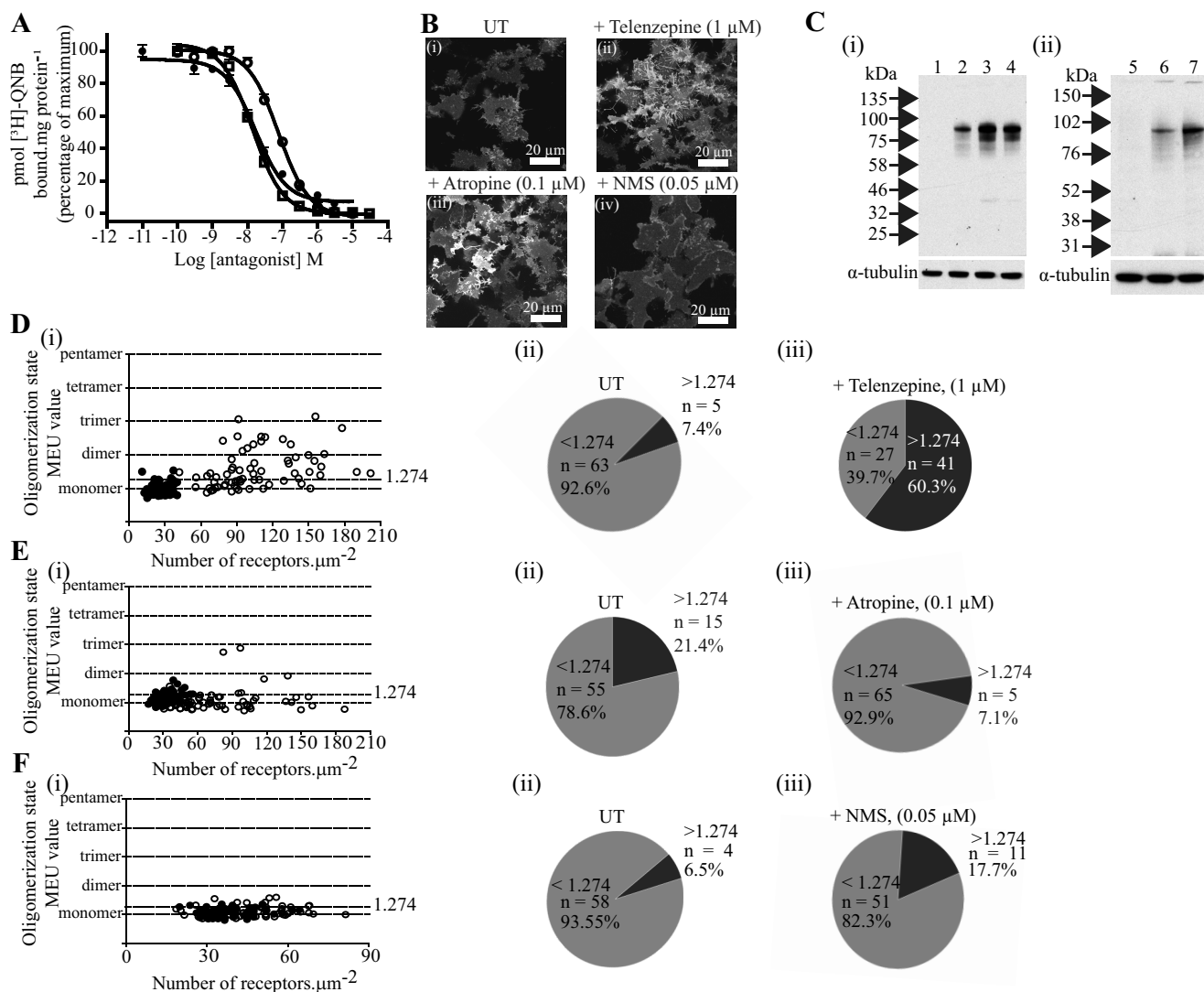
FIGURE 8. Telenzepine, but not atropine or N -methylscopolamine, also promotes M_1 receptor oligomerization. As in Fig. 3, cells harboring h M_1 -mEGFP were treated with 100 ng \cdot\text{ml}^{-1} doxycycline for 24 h to induce expression of the receptor construct. A , membrane preparations from these cells were used in ligand binding studies using a fixed concentration of [ ^3\text{H} ]QNB (1 nM) and varying concentrations of either telenzepine (open circles), atropine (open squares), or N -methylscopolamine (filled circles). Shown are representative plots from n = 3 ; error bars represent \pm S.E. B , images of the basolateral surface of cells treated with vehicle (UT) (panel i), telenzepine (panel ii), atropine (panel iii), or NMS (panel iv). C , immunoblotting of cell lysates confirmed up-regulation of h M_1 -mEGFP following treatment with telenzepine (panel i, lane 3), atropine (panel i, lane 4), or N -methylscopolamine (panel ii, lane 7). Cell lysate from uninduced cells (panel i, lane 1 and panel ii, lane 5) and from cells treated with the vehicle (panel i, lane 2 and panel ii, lane 6) were also loaded for comparison. Detection of \alpha -tubulin acted as a loading control. D , E , and F , comparisons of QB (presented as monomeric equivalent units) and receptor expression levels in cells induced to express h M_1 -mEGFP by treatment with 100 ng \cdot\text{ml}^{-1} doxycycline that were then untreated (filled symbols) or treated with 1 \mu\text{M} telenzepine ( D , panel i, open symbols), 0.1 \mu\text{M} atropine ( E , panel i, open symbols), or 0.05 \mu\text{M} N -methylscopolamine ( F , panel i, open symbols) for 16 h. Although treatment with telenzepine produced a large increase in the proportion of Rols containing predominantly receptor dimers/oligomers ( D , panels ii and iii), atropine ( E , panels ii and iii), and N -methylscopolamine ( F , panels ii and iii) did not.
