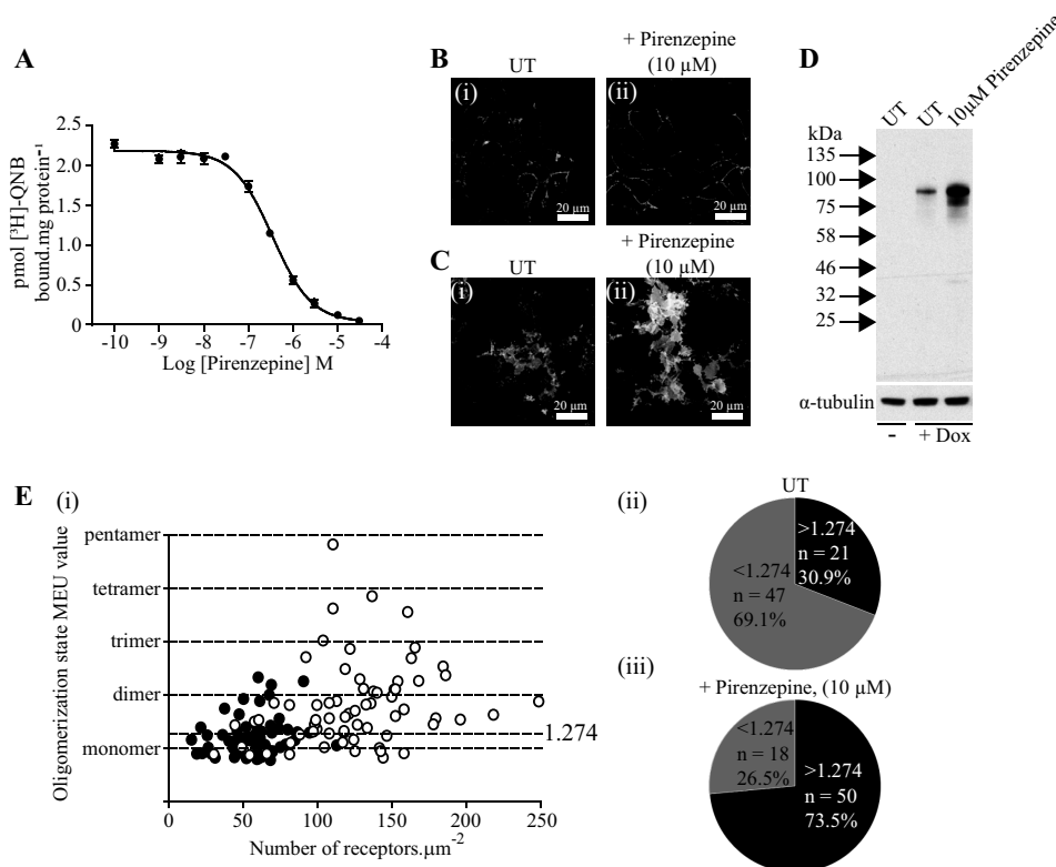
FIGURE 4. Sustained treatment with pirenzepine causes relocation and up-regulation of hM 1 -mEGFP and promotes oligomerization of the receptor. Flp-In T-REx 293 cells harboring hM 1 -mEGFP were treated with doxycycline (100 ng·ml -1 ) for 24 h. A , membrane preparations from these cells were used in ligand binding studies using 1 nM [ 3 H]QNB and varying concentrations of pirenzepine. Based on the K_d for [ 3 H]QNB, estimated as 98 \pm 17 pM, the inhibition constant ( pK_i ) for pirenzepine was calculated as 7.66 \pm 0.04 . Shown is a representative graph from n = 3 ; error bars represent \pm S.E. Cells were then treated with vehicle (UT) or with pirenzepine (10 \mu M) for 24 h. B , panels i and ii , confocal images as in Fig. 2 showed that treatment with pirenzepine resulted in relocation of hM 1 -mEGFP to enhance cell surface/plasma membrane localization. C , panels i and ii , imaging the basolateral surface of a group of cells indicated that pirenzepine caused up-regulation of hM 1 -mEGFP. D , immunoblotting studies confirmed that pirenzepine caused up-regulation of hM 1 -mEGFP. \alpha -Tubulin acted as a loading control. E , panels i – iii , quantal brightness and fluorescence intensity analysis from SpIDA confirmed an overall 2.1-fold up-regulation of receptor number at the basolateral surface and that a substantially greater proportion of the RoIs were identified as containing dominantly receptor dimers/oligomers (73.5%) following pirenzepine treatment ( open symbols ) than in vehicle-treated controls (30.9%) ( filled symbols ).
