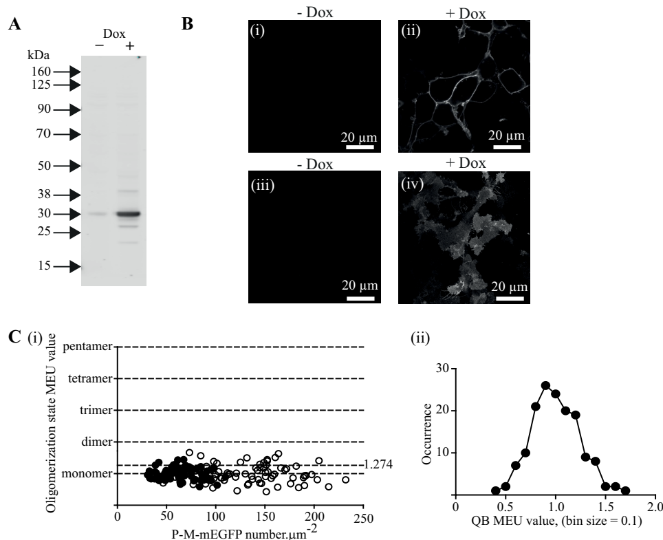
FIGURE 2. Expression, cellular distribution profile, and quantal brightness analysis of plasma membrane-targeted mEGFP. Flp-In T-REx 293 cells harboring P-M-mEGFP were maintained in the absence of doxycycline ( -Dox ) or treated with doxycycline ( 10 \text{ ng}\cdot\text{ml}^{-1} ) for 24 h ( +Dox ). Lysates of these cells were resolved by SDS-PAGE and immunoblotted with an anti-GFP antiserum (A). In B, images of uninduced cells (panels i and iii ) or cells induced to express P-M-mEGFP (panels ii and iv ) are shown. B, panels i and ii , confocal images across groups of cells. B, panels iii and iv , images of the basolateral surface of such cells. C, panel i , shows QB assessed in individual Rols (presented as monomeric equivalent units) plotted against number of mEGFP/ \mu\text{m}^{-2} of the basolateral surface. Filled symbols, cells treated with 2.5 \text{ ng}\cdot\text{ml}^{-1} doxycycline; open symbols, cells treated with 10 \text{ ng}\cdot\text{ml}^{-1} doxycycline. C, panel ii , QB values from individual Rols were binned (bin size, 0.1 MEU), and these displayed a symmetrical distribution (see “Results”).
