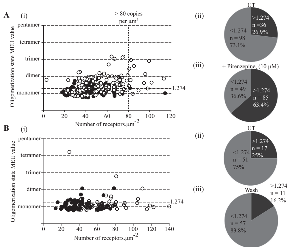
FIGURE 7. Short term treatment with pirenzepine also promotes hM 1 receptor dimer/oligomeric organization, and removal of the ligand results in reversal. Flp-In T-REx 293 cells harboring hM 1 -mEGFP were treated with 100 ng·ml -1 doxycycline for 24 h to induce expression of the receptor construct. A , cells were then treated with pirenzepine (10 \mu\text{M} ) (open symbols) or vehicle (filled symbols) for 90 min. Pirenzepine treatment resulted in a small increase in cell surface receptor levels (54.1 \pm 1.7 versus 41.8 \pm 1.3 copies· \mu\text{m}^{-2} ) (panel i ) but a substantial increase in RoIs containing predominantly high order oligomers (63 versus 27%) (panels ii and iii ). B , following washing of cells that had been exposed to pirenzepine (open symbols) or untreated (filled symbols), quaternary organization was assessed 90 min later (panel i ). In this study, 25% of RoIs from the previously untreated cells were now estimated to have hM 1 -mEGFP in predominantly dimeric/oligomeric forms, whereas for those previously exposed to pirenzepine this was 16% (panels ii and iii ). UT, untreated.
