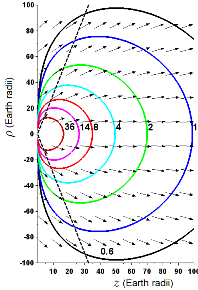
Figure 6: Reflector requirements for a displaced polar orbit. Contours indicate radiation pressure acceleration \kappa ( \text{mms}^{-2} ) and the dashed line indicates the stability boundary (linear stable orbits if \rho > 3.1z ).
