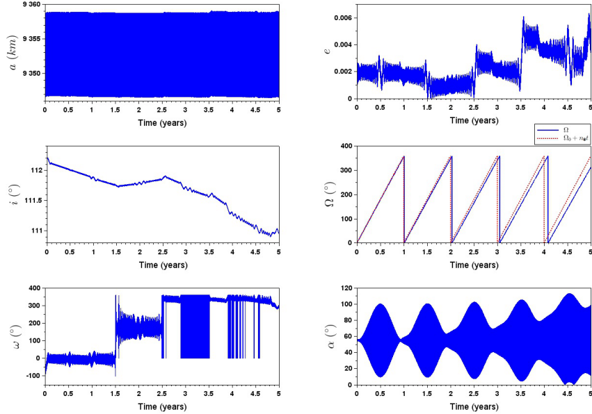
Figure 3: Classical orbit elements of a sun-synchronous orbit and Sun angle variation with \phi = 55^\circ and \kappa = 1.0 \text{ mm/s}^2 during 5 years.
