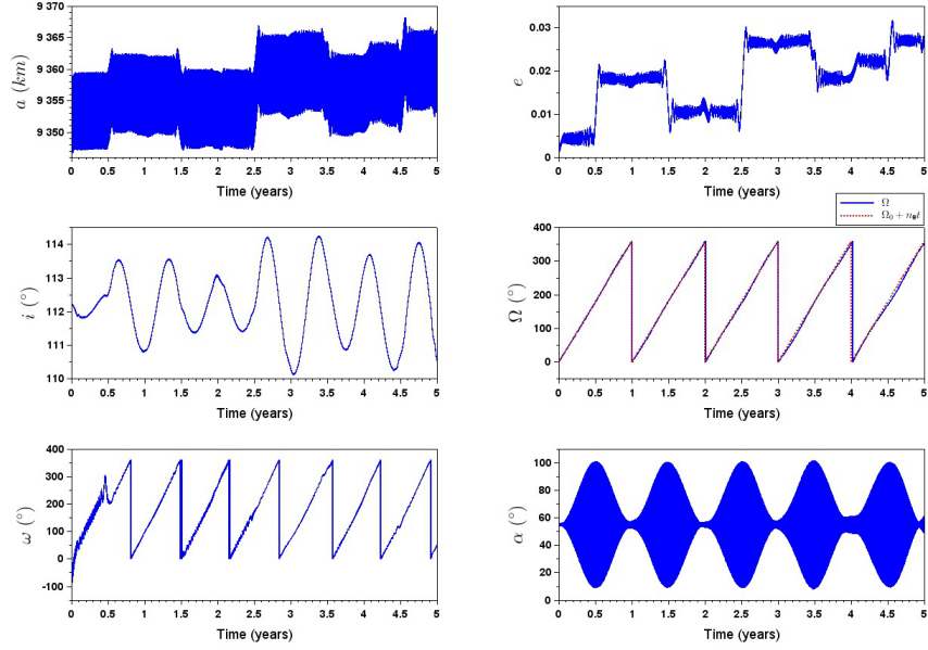
Figure 4: Classical orbit elements of a Sun-synchronous orbit and Sun angle variation with \phi = 55^\circ and \kappa = 5.0 \text{ mm/s}^2 during 5 years.
