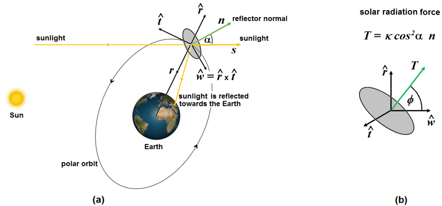
Figure 1: (a) Solar reflector on a polar orbit and radial, transverse and normal (RTN) frame, (b) Solar radiation force.
