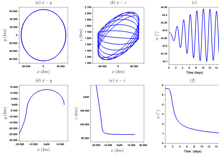
Figure 7: (a)-(b) Uncontrolled stable orbit I ( \rho_0 = 10.0 Earth radii, z_0 = 0.25 Earth radii, \xi = 10^{-3}\rho_0, \eta_0 = 10^{-3}z_0 ), (d)-(e) Unstable orbit II ( \rho_0 = 2.0 Earth radii, z_0 = 10.0 Earth radii, \xi = 10^{-3}\rho_0, \eta_0 = 10^{-3}z_0 ). Variation of the pitch angle \alpha for orbits I (c) and II (f). First plot: (x, y) projection; Second plot: (x, z) projection.
