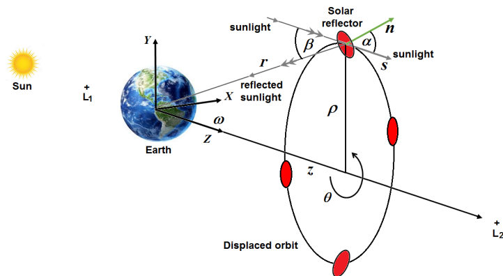
Figure 5: Solar reflectors on a displaced polar orbit along the Sun-line.
