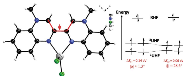
Fig. 7 Thermal ellipsoid view of the asymmetric unit of [\text{CdCl}_2(1^0)] (left). Corresponding energy level scheme showing the relative energies between singlet RHF, 1^{\text{UHF}} and triplet 3^{\text{UHF}} , as well as highlighting the open-shell singlet ground state and the \phi -angle dependent reduction of the singlet to triplet energy gap ( \Delta E_{\text{ST}} ) (right) with \phi the dihedral angle defined by the red lines.
