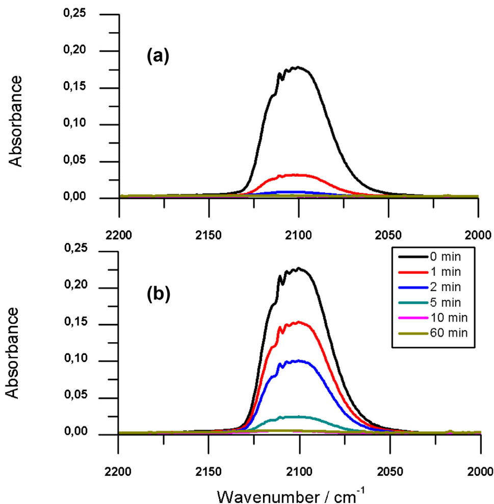
Fig. 1. The infrared spectrum (2200–2000 \text{cm}^{-1} ) for the hydrogenation of 3-butyne-2-one as a function of time (0–60 min) over (a) \text{Pd}(\text{NO}_3)_2/\text{Al}_2\text{O}_3 and (b) \text{PdCl}_2/\text{Al}_2\text{O}_3 .
