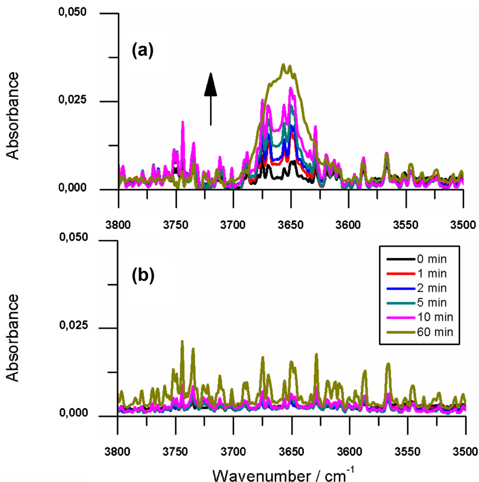
Fig. 4. The infrared spectrum (3800–3500 cm -1 ) for the hydrogenation of 3-butyne-2-one as a function of time (0–60 min) over (a) Pd(NO 3 ) 2 /Al 2 O 3 and (b) PdCl 2 /Al 2 O 3 . The arrow signifies the intensity trend as a function of time for the band at 3655 cm -1 .
