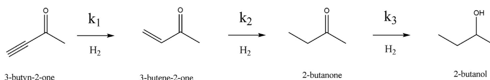
Scheme 1. A reaction scheme for the hydrogenation of 3-butyne-2-one. Stage 1 is the reduction of 3-butyne-2-one to produce 3-butene-2-one; Stage 2 is the reduction of 3-butene-2-one to produce 2-butanone; Stage 3 is the reduction of 2-butanone to produce 2-butanol. k_1 – k_3 are the associated rate coefficients.
