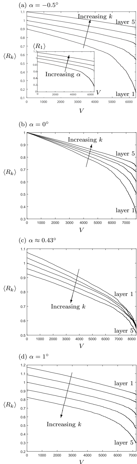
Figure 5: Variation of mean pore radius \langle R_k \rangle = \sum_{i=1}^n \sum_{j=1}^m r_k^{(i,j)} versus throughput V in a non-connected five-layer filter ( N = 5 ) for 1 \leq k \leq 5 with taper angle (a) \alpha = -0.5 , (b) \alpha = 0 , (c) \alpha = \alpha^* \approx 0.43 , (d) \alpha = 1 when filtering particles of size a = 0.5 and adhesivity p_a = 0.1 . For the optimal taper angle the final radius of pores in each layer is approximately equal indicating optimal filter usage. (Note the axes scaling differs in each case.) The inset in (a) compares the evolution of \langle R_1 \rangle with throughput V for the four different taper angles shown in (a)–(d).
