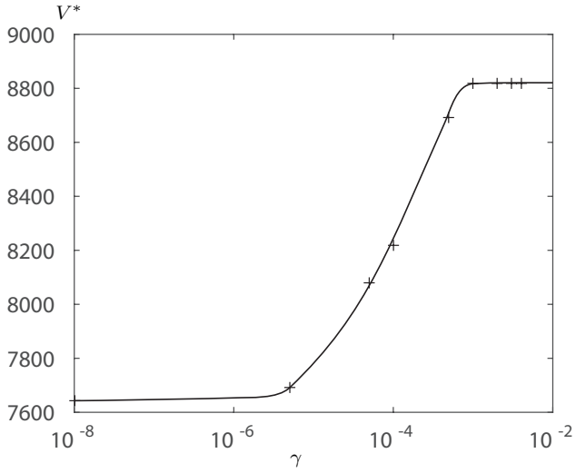
Figure 11: Final throughput V^* versus pore interconnectivity \gamma for a five-layer filter ( N = 5 ) with particle size a = 0.5 , adhesivity p_a = 0.1 , total filter depth h = 20 , and taper angle \alpha = 0 . The crosses show the data points generated by the simulations and the black curve is a fit to the data.
