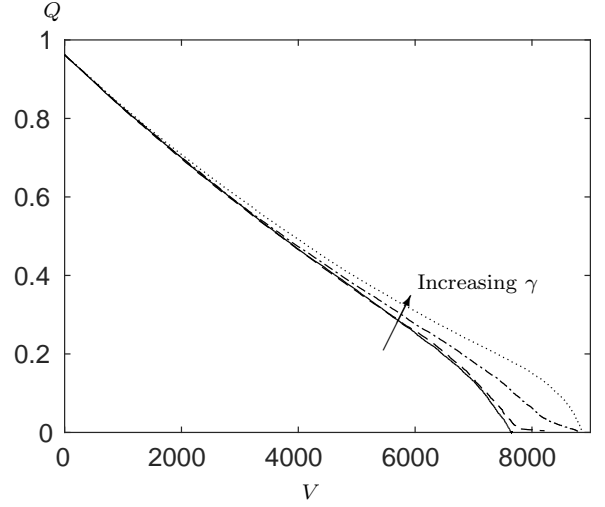
Figure 10: Flux Q versus throughput V for a five-layer filter ( N = 5 ) with particle size a = 0.5 , adhesivity p_a = 0.1 , filter depth h = 20 , taper angle \alpha = 0 and connectivity \gamma = 0 (solid), 1 \times 10^{-4} (dashed), 7 \times 10^{-3} (dot-dashed), 0.02 (dotted). Only a small amount of connectivity is required to increase the throughput, which is achieved through a region of convexity in the QV signature. When \gamma is increased beyond approximately 7 \times 10^{-3} the convex region begins to disappear while the final throughput V^* remains the same. The QV signature is unchanged by increases in connectivity beyond \gamma \approx 0.02 .
