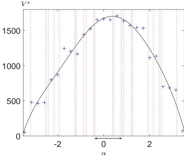
Figure 7: Final throughput V^* versus taper angle \alpha for a non-connected ( \gamma = 0 ) five-layer filter ( N = 5 ) with particle size a = 0.7 , adhesivity p_a = 0.1 , and total filter depth h = 20 . The black curve is a polynomial fit to the data. The discrete variation in throughput with taper angle is much more apparent than when a = 0.5 (figure 4) due to the discrete variations in the number of particles that may be accepted by the filter (figure 6). The red dotted lines denote the taper angles that correspond to a change in the number of particles that can be accepted by the filter and separate the data into the expected discrete regions. The arrows show the region over which the throughput is approximately constant and maximal.
