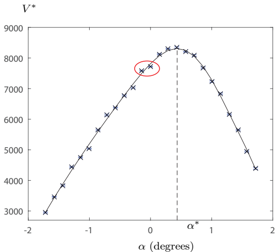
Figure 4: Final throughput V^* versus taper angle \alpha for a non-connected five-layer filter ( N = 5 ) with particle size a = 0.5 , adhesivity p_a = 0.1 , and total filter depth h = 20 . The crosses show the data points and variance from the mean generated by the simulations, and the black curve is a polynomial fit with optimum at \alpha^* \approx 0.43^\circ . The two circled data points correspond to \alpha = 0^\circ and -0.14^\circ .
