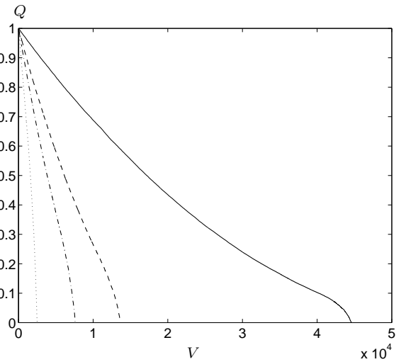
Figure 14: Flux, Q versus throughput V for a non-connected ( \gamma = 0 ) filter with N = 1 (solid), 3 (dashed) 5 (dot-dashed) and 11 (dotted) layers, of constant total filter thickness h = 20 when filtering particles of size a = 0.5 and adhesivity p_a = 0.1 .
