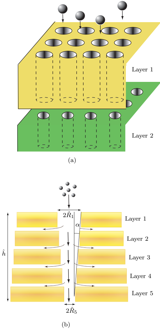
Figure 1: (a) Schematic diagram of a multilayer filter. Each layer, k , is initially composed of an array of n \times m equal-sized pores, but whose radius \hat{R}_k may vary for each layer. (b) Front schematic view illustrating the different pore radii at each layer and the taper angle. At each level the particle may pass into the pore directly beneath, or may traverse to one of four neighbouring pores. (Here two neighbouring pores are shown; the additional two pores are located into and out of the page.) The total filter thickness is \hat{h} .
