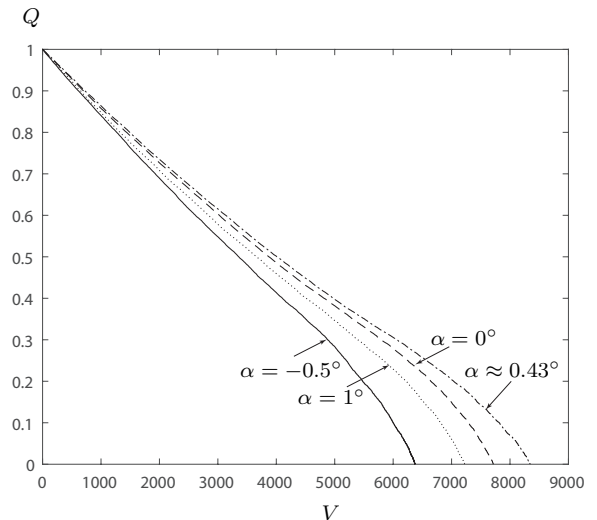
Figure 3: Flux Q versus throughput V for a non-connected ( \gamma = 0 ) five-layer filter ( N = 5 ) with particle size a = 0.5 , adhesivity p_a = 0.1 , filter depth h = 20 and taper angle \alpha = -0.5^\circ (solid), 0^\circ (dashed), \alpha^* \approx 0.43^\circ (dot-dashed), 1^\circ (dotted) illustrating the increase and then decrease in final throughput V^* with increasing taper angle.
