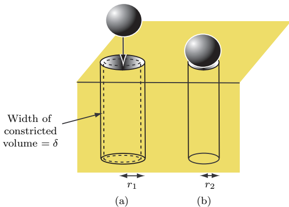
Figure 2: Schematic diagram of possible blocking mechanisms: (a) Standard blocking : Here pore radius r_1 > a . Upon acceptance of n \geq 1 particles the pore radius reduces to a new radius \sqrt{r_1^2 - 4na^3/3h} . (b) Complete blocking : Here the pore radius r_2 < a .
