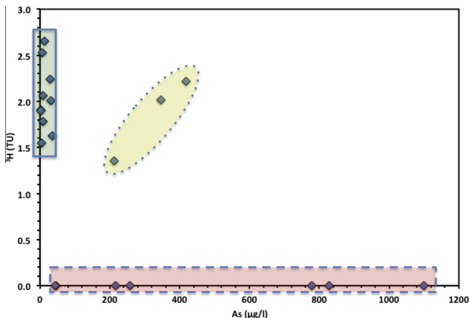
Fig. 4. Distinct groups of groundwaters discriminated by ^3\text{H} and dissolved As. (i) tritium-active groundwaters with \text{As} = 2\text{--}35 \mu\text{g/l} (highlighted by green rectangle demarked by solid lines), (ii) tritium-active groundwaters with \text{As} > 200 \mu\text{g/l} (highlighted by yellow oval and demarked by dotted lines), and (iii) tritium-dead groundwaters with highly variable ( 44\text{--}1100 \mu\text{g/l} ) As (highlighted by red rectangle and demarked by dashed lines). (For interpretation of the references to colour in this figure legend, the reader is referred to the web version of this article.)
