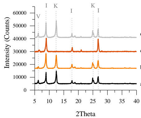
Fig. 3b XRD Diffractogram (Soil V)
